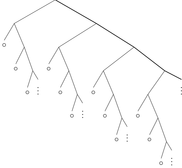
Figure 2: The infinite 2-branching tree. The spine is indicated by the thick edge. The vertices of any T_{k+1} can be partitioned into the vertices on the spine, plus countably many copies of T_k .
