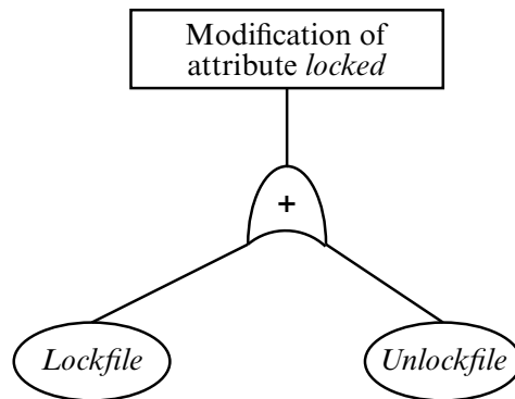
Figure 18–3 Second stage of building tree.
