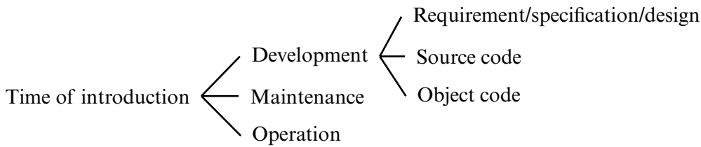
Figure 24-9 NRL taxonomy: flaws by time of introduction.
