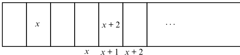
Figure 24–2 An example of the parameter passing conventions. Here, x is the address of the parameter list, and locations x , x + 1 , and x + 2 contain addresses of the actual parameters. Note that location x + 1 contains the address x + 2 , meaning that the last address in the parameter list is itself the location of a parameter (as well as containing the address of another parameter).
