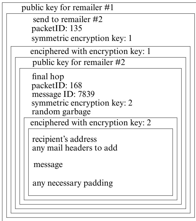
Figure 15–2 A Mixmaster message. This is a fragment of a multipart message sent through two remailers. Messages are enciphered using both a public key and symmetric key algorithm, and random garbage is added as well as padding. The recipient's address is visible only to the last remailer.
