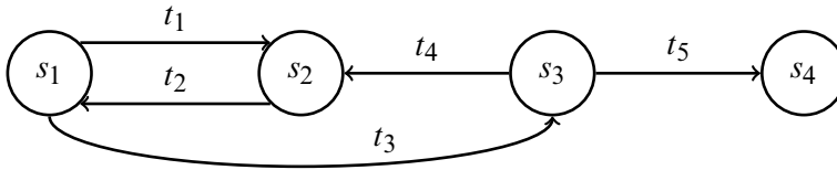
Figure 4-1 A simple finite-state machine.
