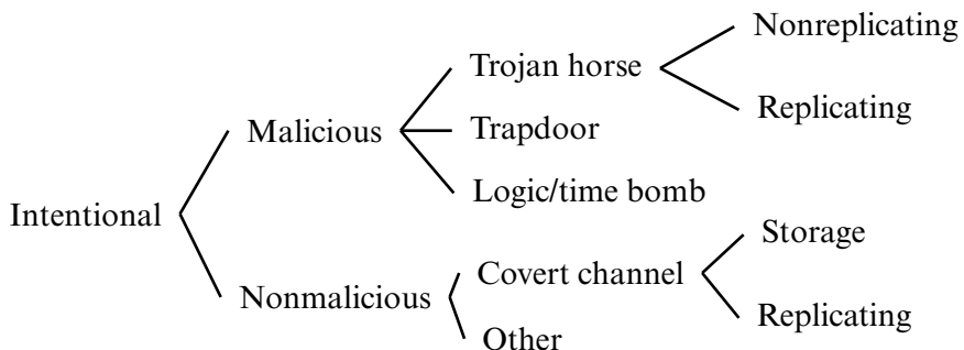
Figure 24–8 NRL taxonomy: flaws by genesis. This diagram shows only the intentional portion of the taxonomy; the inadvertent portion is similar to the RISOS taxonomy except that the first two RISOS classes are merged.
