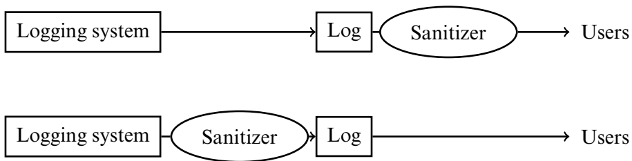
Figure 25-1 The different types of sanitization. The top image shows logs being sanitized for external viewing. The bottom image shows logs being sanitized for privacy of users. In this case, the sanitizer may save information in a separate log that enables the reconstruction of the omitted information. Cryptographic techniques enforce separation of privilege, so multiple administrators must agree to view the unsanitized logs.
