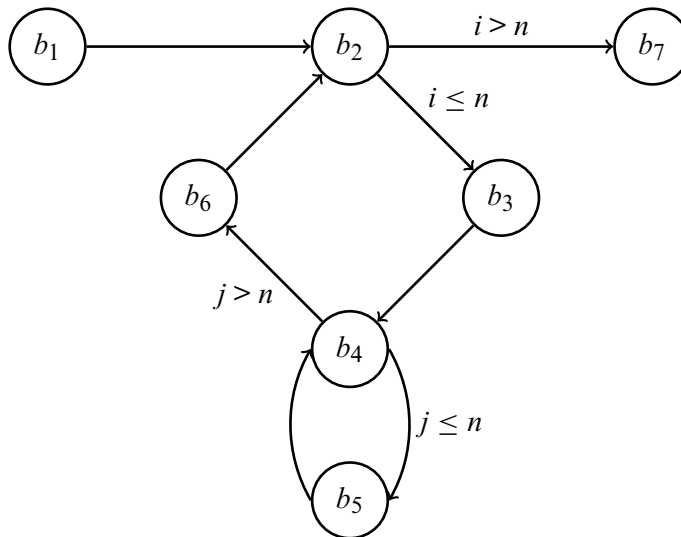
Figure 17–3 The control flow graph of the procedure transmatrix . The basic blocks are labeled b_1 through b_7 . The conditions under which branches are taken are shown over the edges corresponding to the branches.
