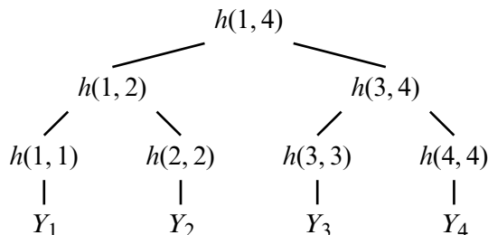
Figure 11–1 A representation of the recursion involved in Merkle's scheme for a file with four identity and public key pairs. The hash of the file is h(1, 4) , and this is known to all parties.
