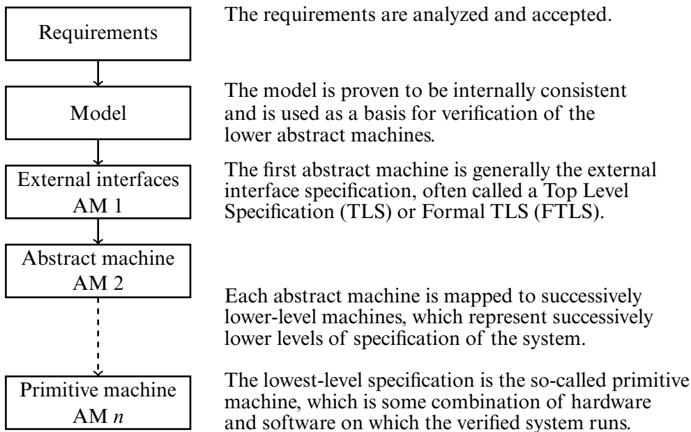
Figure 21–1 Levels of abstract machines in HDM.
