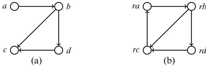
Figure 3–5 The rule of acyclic creates. (a) The can-create relation cc = \{(a, b), (b, c), (b, d), (d, c)\} . Because there are no cycles in the graph, cc satisfies the rule of acyclic creates. (b) Same as (a), except that the can-create relation is cc' = cc \cup \{(c, a)\} , which creates a cycle; hence, cc' does not follow the rule of acyclic creates.
