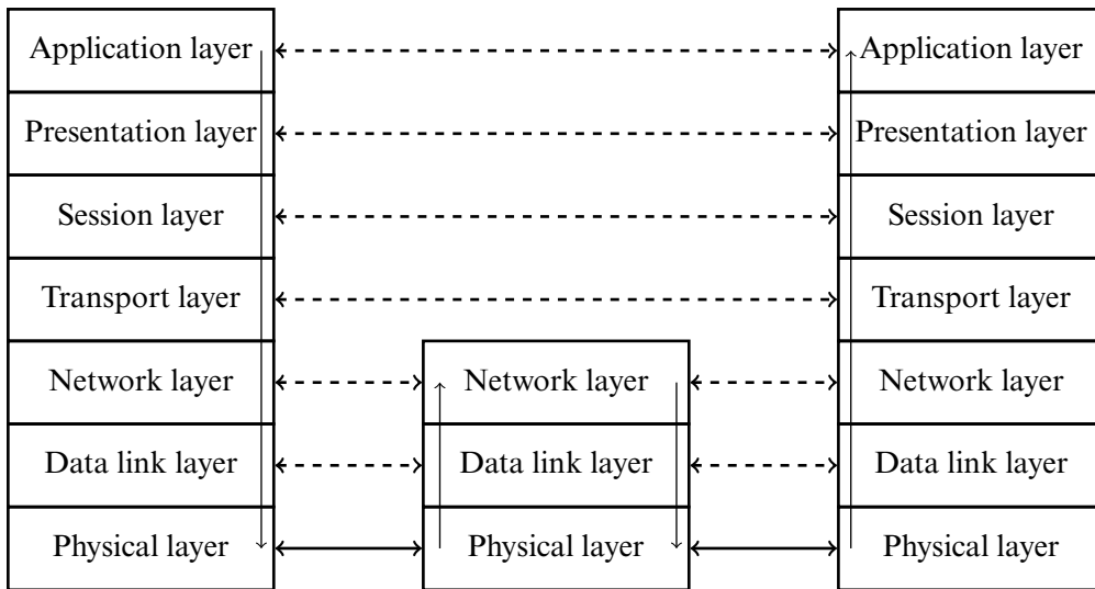
Figure 12–6 The ISO/OSI model. The dashed arrows indicate peer-to-peer communication. For example, the transport layers are communicating with each other. The solid arrows indicate the actual flow of bits. For example, the transport layer invokes network layer routines on the local host, which invoke data link layer routines, which put the bits onto the network. The physical layer passes the bits to the next “hop,” or host, on the path. When the message reaches the destination, it is passed up to the appropriate level.
