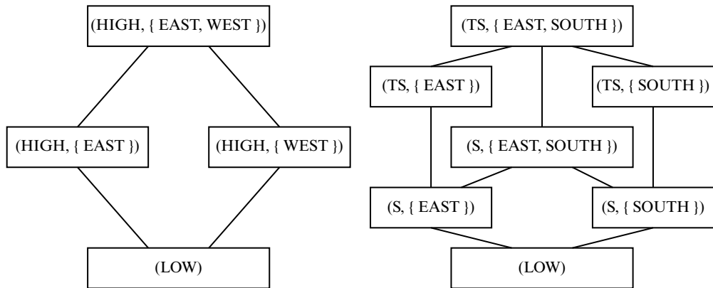
Figure 9-1 The lattice on the left corresponds to the policy of system windsor and the one on the right represents system scout .
