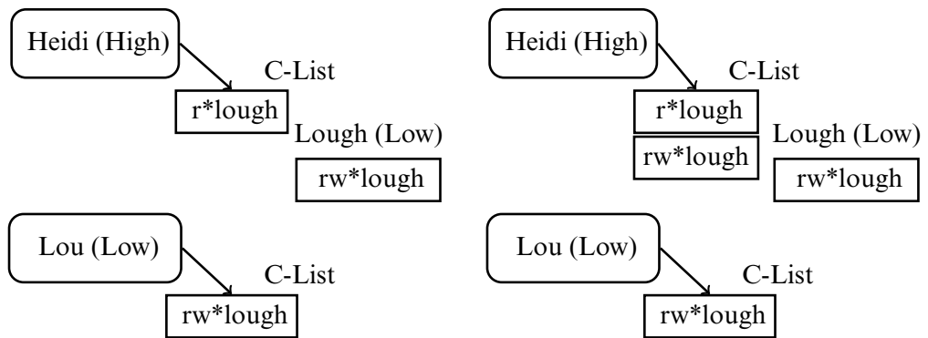
Figure 16–1 Copying and reading capabilities. The left diagram shows the capability rw*lough copied into the file lough . In the right diagram, Heidi has read the contents of the file lough and added the capability it contains to her C-List.
