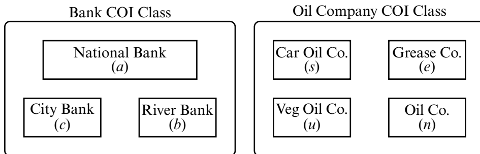
Figure 8–1 The Chinese Wall model database. It has two COI classes. The one for banks contains three CDs. The other one, for oil companies, contains four CDs. Susan may have access to no more than one CD in each COI, so she could access City Bank's CD and Veg Oil Co.'s CD, but not City Bank's CD and National Bank's CD.
