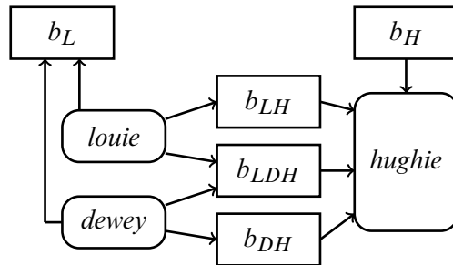
Figure 9–3 Composition of systems.
