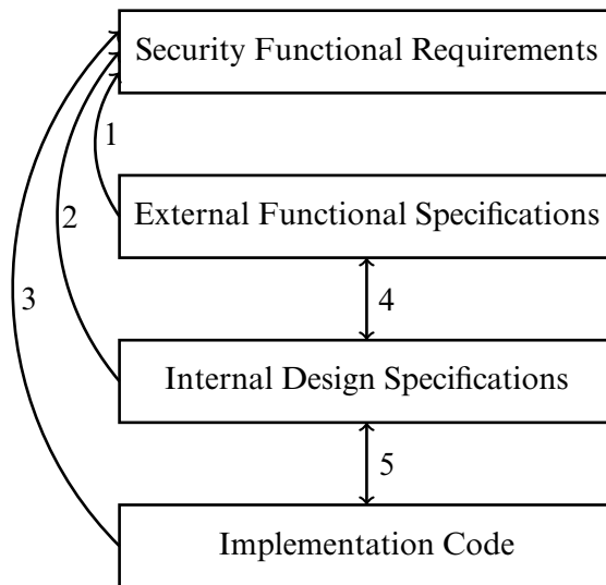
Figure 20–2 Requirements mapping and informal correspondence. Arrows 1, 2, and 3 indicate requirements tracing for each of the three levels of specification. Arrows 4 and 5 represent informal correspondence between adjacent levels of specification.
