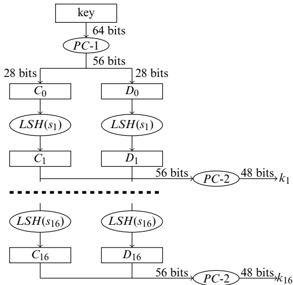
Figure F-5 Key schedule generation.
