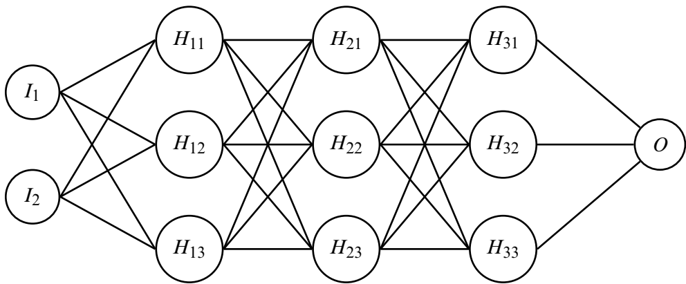
Figure 26-2 A neural net with input nodes I_1 and I_2 , output node O , and three hidden layers of three neurons each. Note the neurons in a layer are not connected to one another. Each connection between neurons also has a weight assigned to it.
