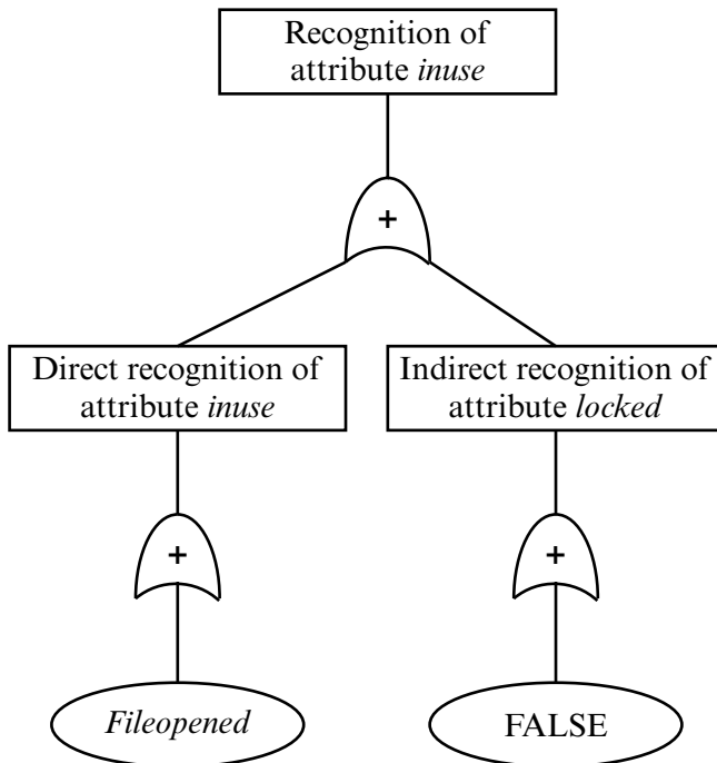
Figure 18-6 Fifth stage of building tree.
