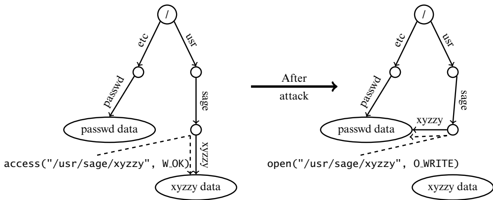
Figure 24–6 (a) The state of the system at the time of the access system call. The labeled arrows indicate the name of the target. Both /usr/sage/xyzzy and /etc/passwd name distinct objects containing their own data. The access system call checks that the data in /usr/sage/xyzzy can be overwritten; this is shown by the dashed arrow in (a). However, before the process makes its open system call, /usr/sage/xyzzy is deleted and a direct alias (hard link) for /etc/passwd is created and named /usr/sage/xyzzy ; the data associated with the previous /usr/sage/xyzzy is no longer accessible by that name. Then the open accesses the data associated with /etc/passwd when it opens /usr/sage/xyzzy because /usr/sage/xyzzy and /etc/passwd now refer to the same file. This is shown in (b), with the dashed arrow indicating which data is actually read.
