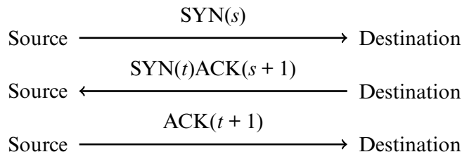
Figure 7–1 The TCP three-way handshake. The SYN packet is a TCP packet with sequence number s (or t ) and the SYN flag set. Likewise, the ACK packet is a TCP packet with acknowledgment number s + 1 (or t + 1 ) and the ACK flag set. The middle message is a single TCP packet with both SYN and ACK flags set.
