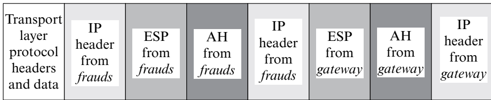
Figure 12–10 An IPsec-protected packet going through nested tunnels. The filled rectangles represent headers. The leftmost IP header and the following data constitute the original packet. The IPsec mechanisms add the ESP, AH, and IP headers of frauds and forward the packet to gateway . This is the first SA and is in tunnel mode. The host gateway adds the ESP, AH, and IP headers shown, putting the packet into the second tunnel mode SA.
