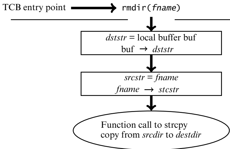
Figure 24–11 The integrated flow path for the rmdir system function in one version of the UNIX operating system. From [837], Figure 11(a), p. 178.
