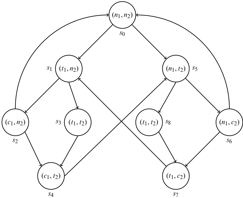
Figure 21-5 Graph of mutual exclusion model.
