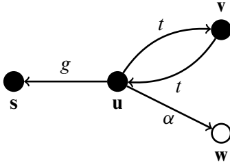
Figure 3–3 The take-grant rules to the right of the graph are a witness to a theft in that graph in which the owner, u , of the stolen right, \alpha , grants other rights to another subject ( t rights to v are granted to s ).
