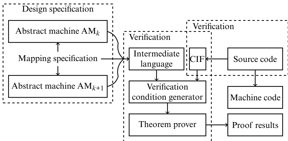
Figure 21–2 Implementation verification in HDM.
