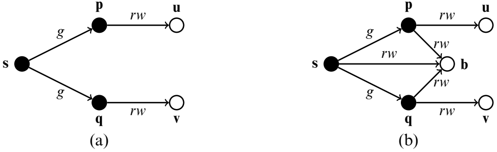
Figure 3–2 (a) The initial state of the system: s , a trusted entity, can grant rights to untrusted processes p and q . Each process p and q controls its own private information (here represented by files u and v ). (b) The trusted entity has created a buffer b shared by the untrusted processes.
