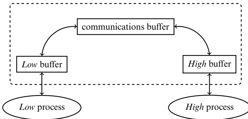
Figure 18–8 The pump. Messages going between the High and Low processes enter the pump (represented by the dashed rectangle). The pump controls the rate at which the messages flow between the two processes. The pump acknowledges each message as it is moved from the process buffer to the communications buffer.
