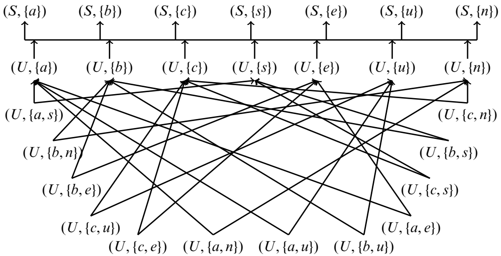
Figure 8–2 The relevant parts of the Bell-LaPadula lattice induced by the transformation applied to the system in Figure 8–1. For example, a subject with security clearance in class (U, \{a, s\}) can read objects with labels (U, \{a\}) and (U, \{s\}) . The Bell-LaPadula Model defines other compartments (such as (U, \{a, b\}) ), but because these would allow access to different CDs in the same COI class, the Chinese Wall model requires that compartment to be empty.
