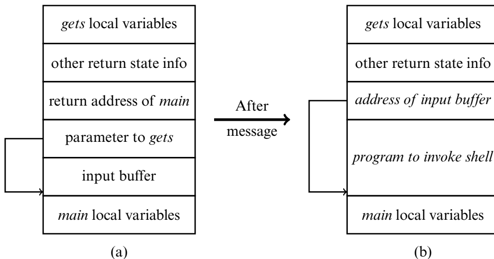
Figure 24–7 (a) The stack frame of fingerd when input is to be read. The arrow indicates the location to which the parameter to gets refers (it is past the address of the input buffer). (b) The same stack after the bogus input is stored. The input string overwrites the input buffer and parameter to gets , allowing a return to the contents of the input buffer. The arrow shows that the return address of main was overwritten with the address of the input buffer. When gets returns, it will pop its return address (now the address of the input buffer) and resume execution at that address.
