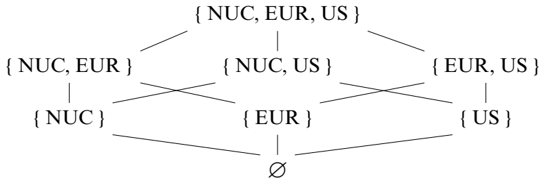
Figure 5–2 Lattice generated by the categories NUC, EUR, and US. The lines represent the ordering relation induced by \subseteq .
