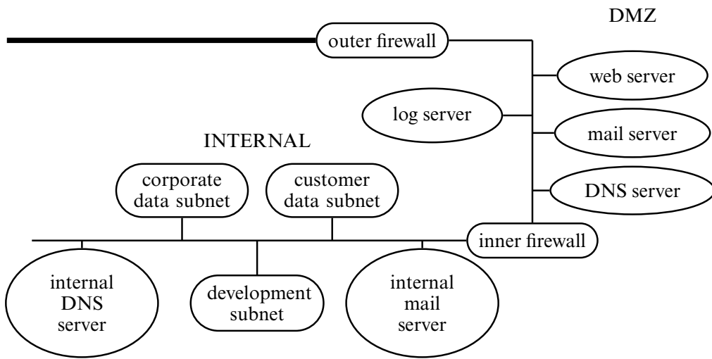
Figure 28–2 The network designed for the Dribble Corporation. The “outer firewall” sits between the Internet and the company network. The subnet labeled “DMZ” provides limited public access to various servers. The “inner firewall” sits between the DMZ and the subnets that are not to be accessed by the public. These subnets share common mail and DNS servers that, like the other hosts, are not publicly accessible.
