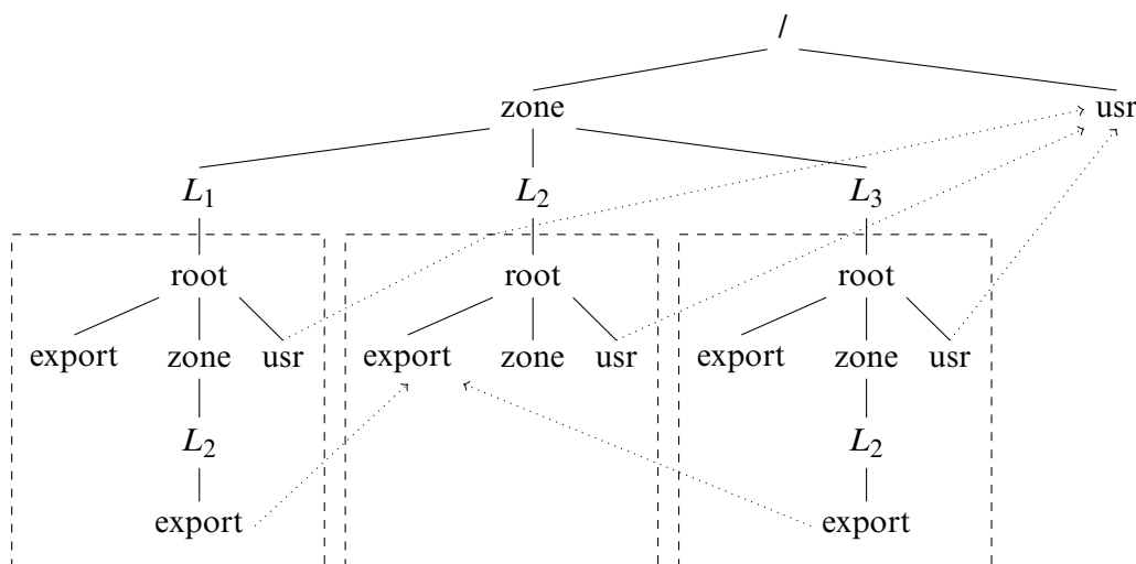
Figure 5–3 An example Solaris Trusted Extensions file system. Three labeled zones ( L_1 , L_2 , and L_3 ) are configured to make their export subdirectories visible. Only zones whose labels dominate L_2 can see those directories. Further, the system directories such as /usr are mounted in each zone so processes can execute system programs. The solid lines are normal mounts; the dotted lines are loopback mounts.
