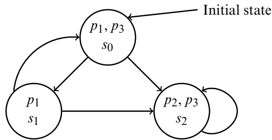
Figure 21-3 Graphical representation of the model M .
