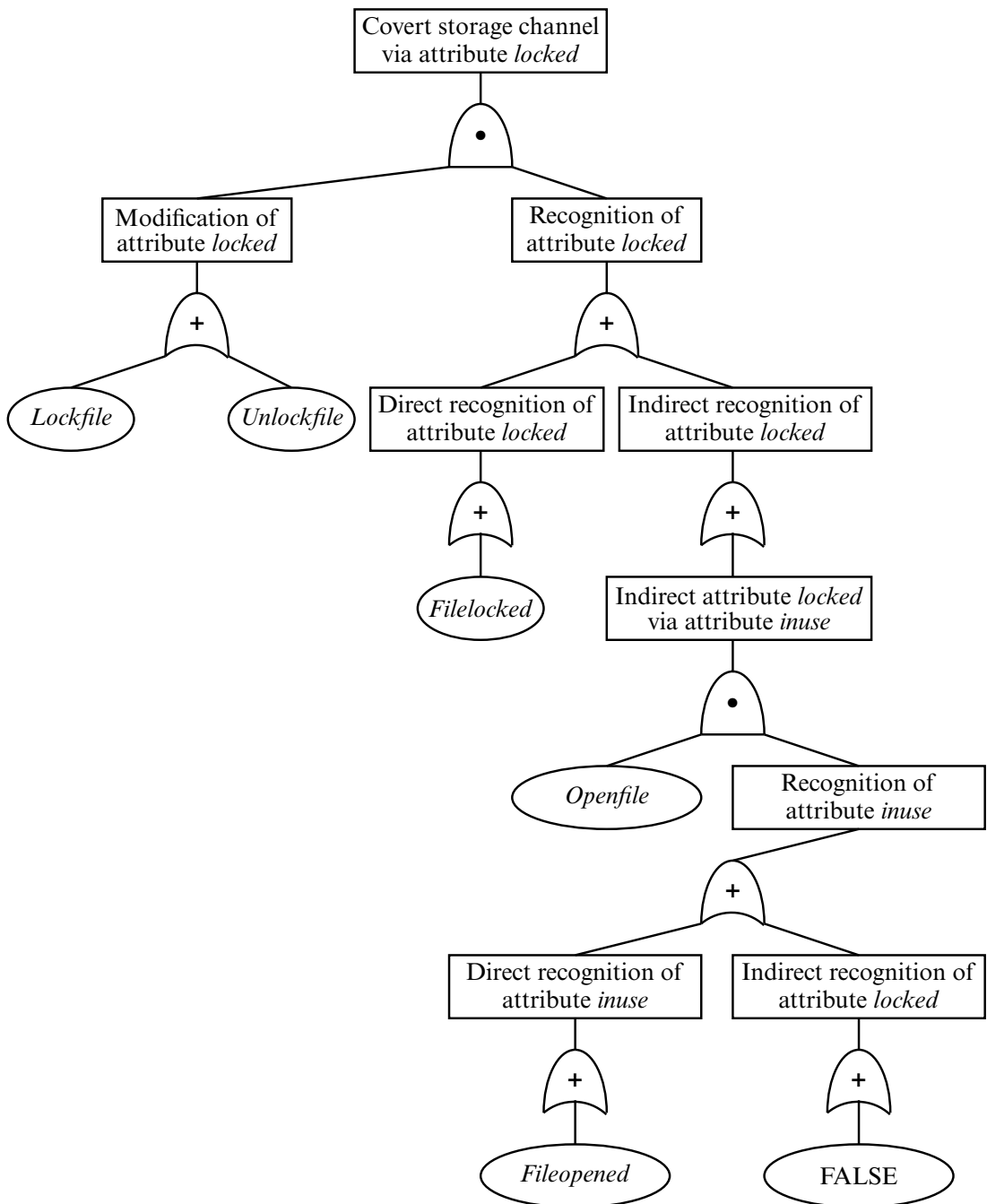
Figure 18–7 The covert flow tree for the operations.
