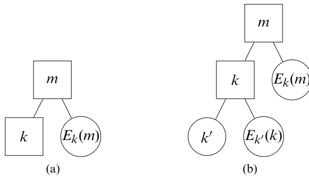
Figure 27-1 Search trees. The square nodes are “required”; the circular ones are “available.”
