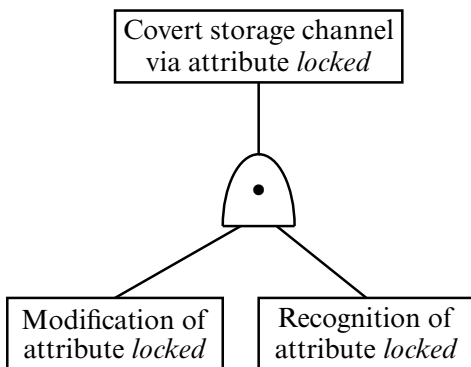
Figure 18–2 First stage of building tree.
