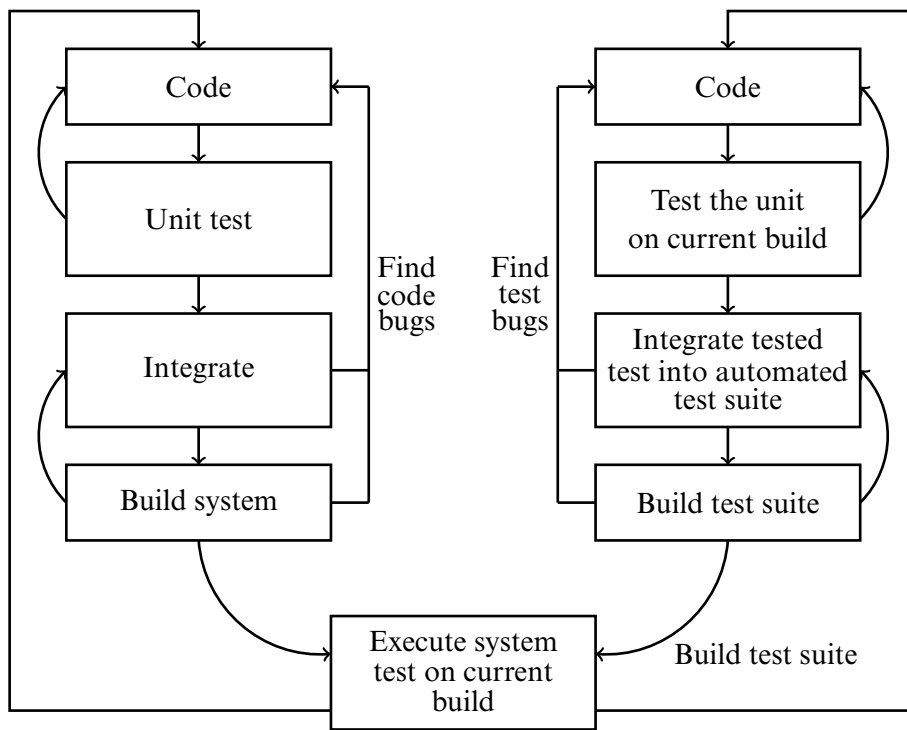
Figure 20–3 Relationship between code development and testing. At the left are the development tasks, and at the right are the testing tasks. Reverse arrows indicate iterative steps.
