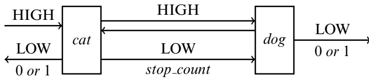
Figure 9–6 The composite machine catdog . Both cat and dog are noninterference-secure, but the composite machine is not.
