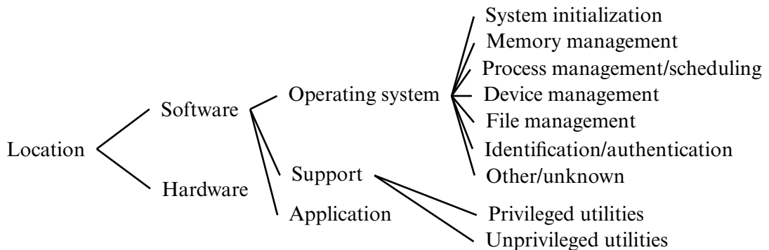
Figure 24-10 NRL taxonomy: flaws by location.
