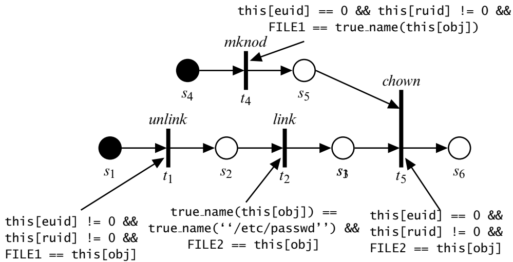
Figure 26-4 The mknod attack on page 853 described using a Colored Petri Automaton. The circles represent states, and the thick bars represent the commands causing transitions.
