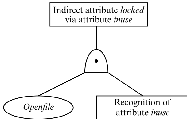
Figure 18-5 Fourth stage of building tree.
