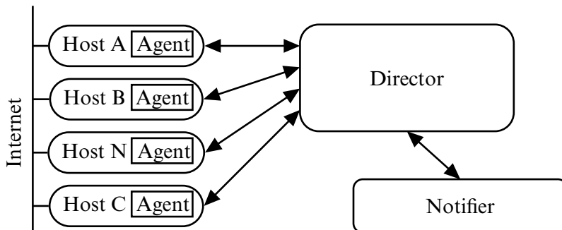
Figure 26–5 Architecture of an intrusion detection system. Hosts A, B, and C are general-purpose computers, and the agents monitor activity on them. Host N is designed for network monitoring, and its agent reports data gleaned from the Internet to the director.
