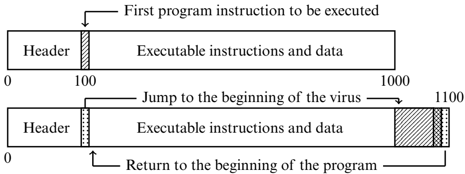
Figure 23–1 How an executable infector works. It inserts itself into the program so that the virus code will be executed before the application code. In this example, the virus is 100 words long and appends itself to the executable code. The first instruction is changed to a branch to the computer virus, and the computer virus arranges to execute the replaced instruction.
