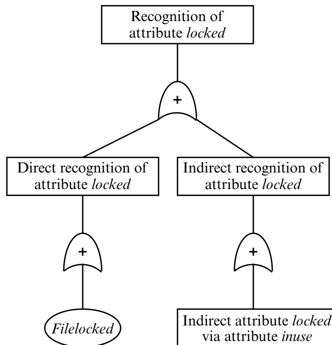
Figure 18–4 Third stage of building tree.
