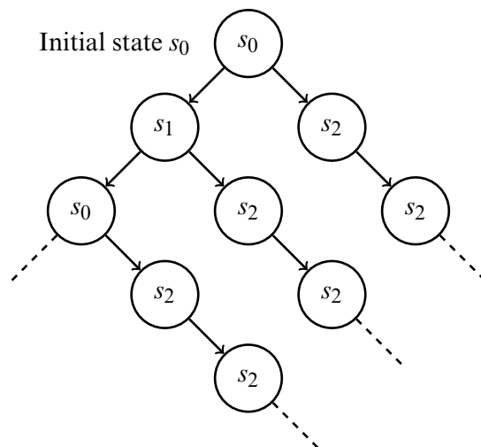
Figure 21-4 Unwinding the graph of M .
