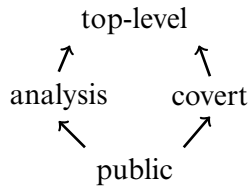
Figure 17–2 An example of a government agency information flow policy. Public information is available to all. All other types of information are restricted, with analysis data and covert data (about secret missions) being distinct types of data. Top-level data is synthesized from both covert and analysis data.
