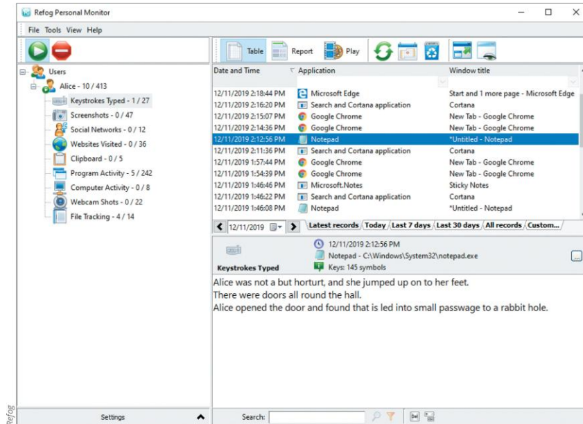
Figure 3-5 Software keylogger
