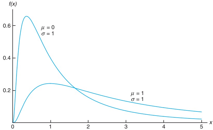
Figure 6.29: Lognormal distributions.
