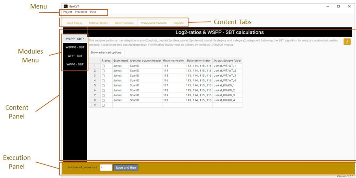
Figure 4. Main View of iSanXoT.
