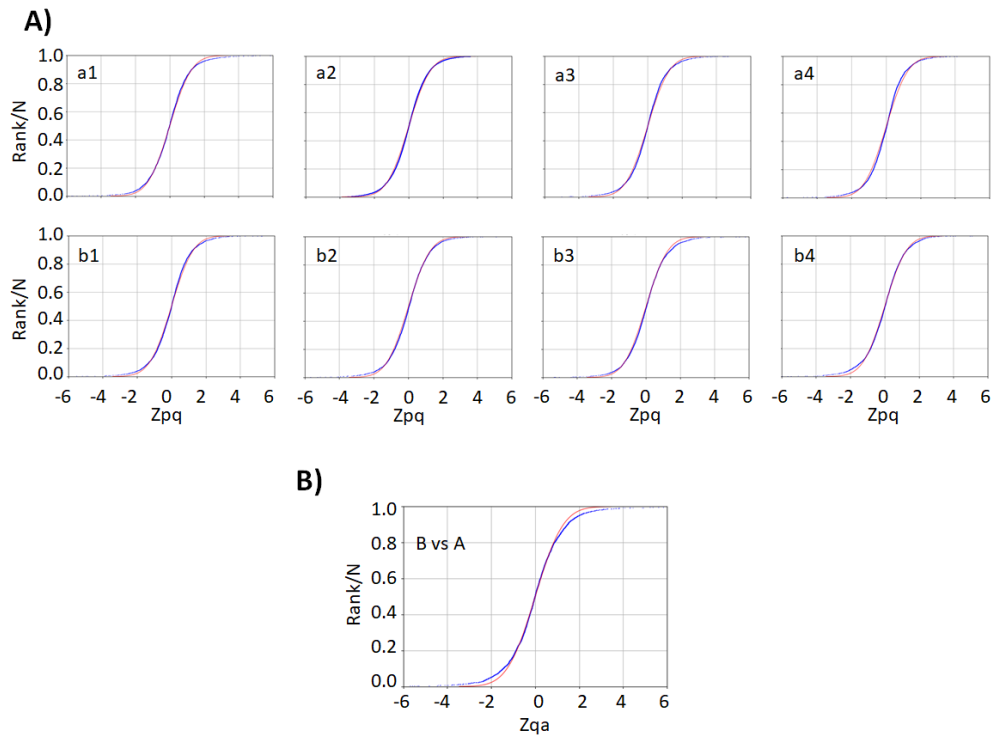
Figure 73. Distribution of the standardized variable at the peptide ( Z_{pq} ) and protein ( Z_{qa} ) levels for label-free data analyzed with iSanXoT. A) Z_{pq} distribution for the eight individual A-type and B-type samples. B) Z_{qa} distribution for the B-type vs A-type comparison. Red: null hypothesis (standard distribution); blue: experimental data.
