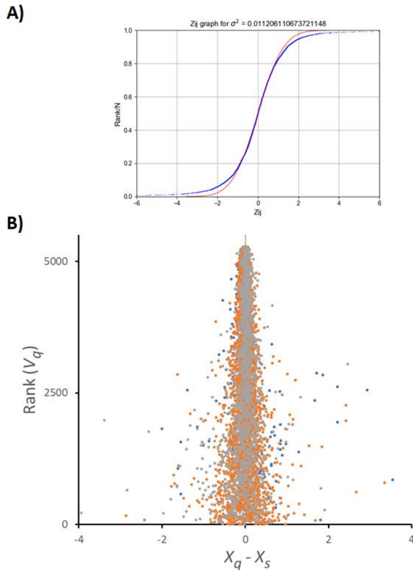
Figure 79. (A) Distribution of the standardized log 2 protein ratios ( Z_{qs} ) resulting from the protein-to-species integration of B\_vs\_A . Red represents the null hypothesis (standard distribution), and blue represents the experimental data. (B) Quantification of human (orange), yeast (grey), and E. coli (blue) proteins using the protein-to-species workflow with NORCOMBINE. The log 2 -ratios are normalized by the respective species ( X_q - X_s ). The letters 'q' and 's' denote the protein and species, respectively.
