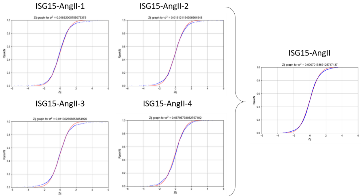
Figure 51. Distribution of the standardized log 2 protein ratios ( Z_{qj} ) from the four individual ISG15-AngII VSMC samples (Left panel). This illustrates how the WSPP model aligns well with the expected null distributions in the four cases. In the right panel, the Figure shows the distribution from the integrated ISG15-AngII sample group obtained with the NORCOMBINE module. This demonstrates how the GIA assumption of a global biological variance is a valid approach to address the biological variability within this group. Red: null hypothesis (standard distribution); blue: experimental data.
