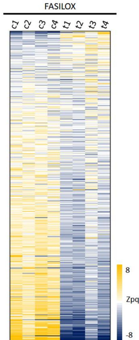
Figure 63. (A) The task table for Workflow 3 is in the REPORT module. (B) Relative abundance of Cys-containing peptides in MEF samples is represented by peptide log 2 ratios expressed in units of standard deviation corrected by the protein mean (Zpq). The data for the heatmap were derived from the "Nscan2pep_Quanpepprot_filtered" report table.
