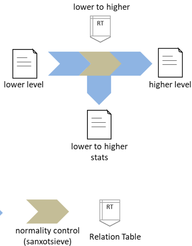
Figure 12. Schematic representation of the INTEGRATE module. The integration is carried out from any lower level to any higher level using the programs “SanXoT” and “SanXoTSieve” and the generic integration algorithm (GIA).
