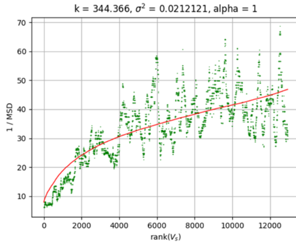
Figure 48. Automatically generated graphs to supervise the accuracy of calibrations. These graphs illustrate 1/MSD versus the rank of V_s (scan weight, which at this level corresponds to reporter intensity). MSD represents the Mean Squared Deviation of the scans versus the respective mean of the peptide to which they belong. The scans are ordered by V_s , and the MSD is calculated in a sliding window of 200 scans [2].
