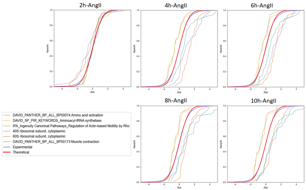
Figure 43. Examples of time-dependent coordinated protein behavior in VSMCs treated with angiotensin-II, revealed by the distribution of the standardized log2 ratio (Zqa) of protein components in each category.
