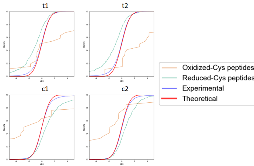
Figure 64. Distribution of the standardized variable at the peptide level ( Z_{pq} ) in control MEF samples (t1, t2, c1 and c2) for all the peptides quantitated (blue) and the oxidized (orange) and reduced (green) Cys-containing peptide subpopulations. The theoretical normal distribution N(0,1) is shown in red. Positive/negative Z_{pq} values indicate increased/decreased peptide abundance with respect to the average. These sigmoidal curves were created from the "Nscan2pep_Quanpeprot" table generated by REPORT.
