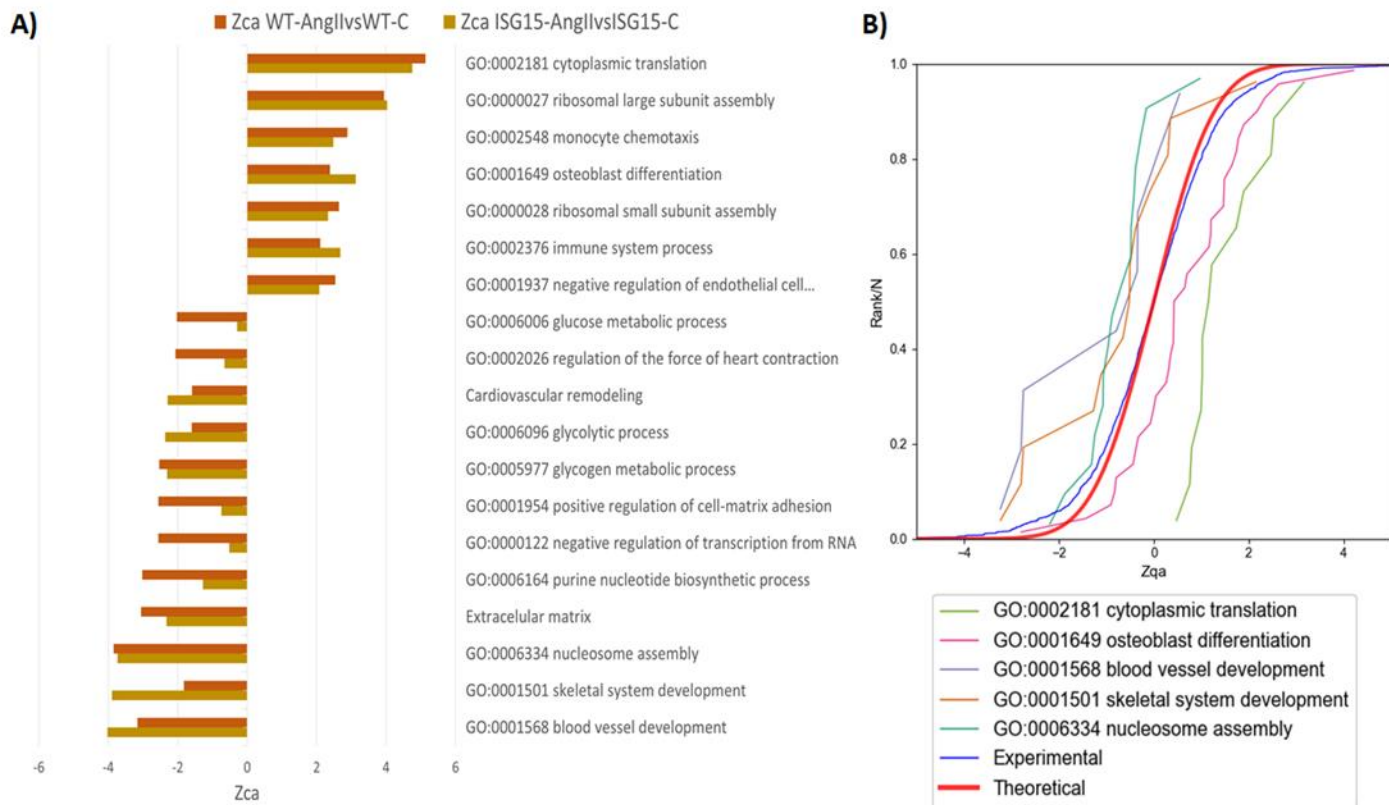
Figure 56. Functional category changes arising from coordinated protein behavior. A) Bar graph for functional categories (Zca) constructed from the "Nprot2cat_Quanecat_filtered" REPORT table. B) The distributions of the standardized log2 protein ratios (Zqa) are shown for some of the functional categories that are significantly down-regulated (Left) or up-regulated (Right). The data to create the sigmoid curves are taken from the "Nprot2cat_Quanecat_Quanprot_filtered" REPORT table.
