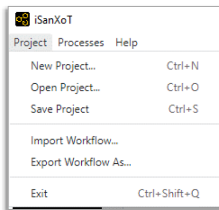
Figure 2. Project menu.
