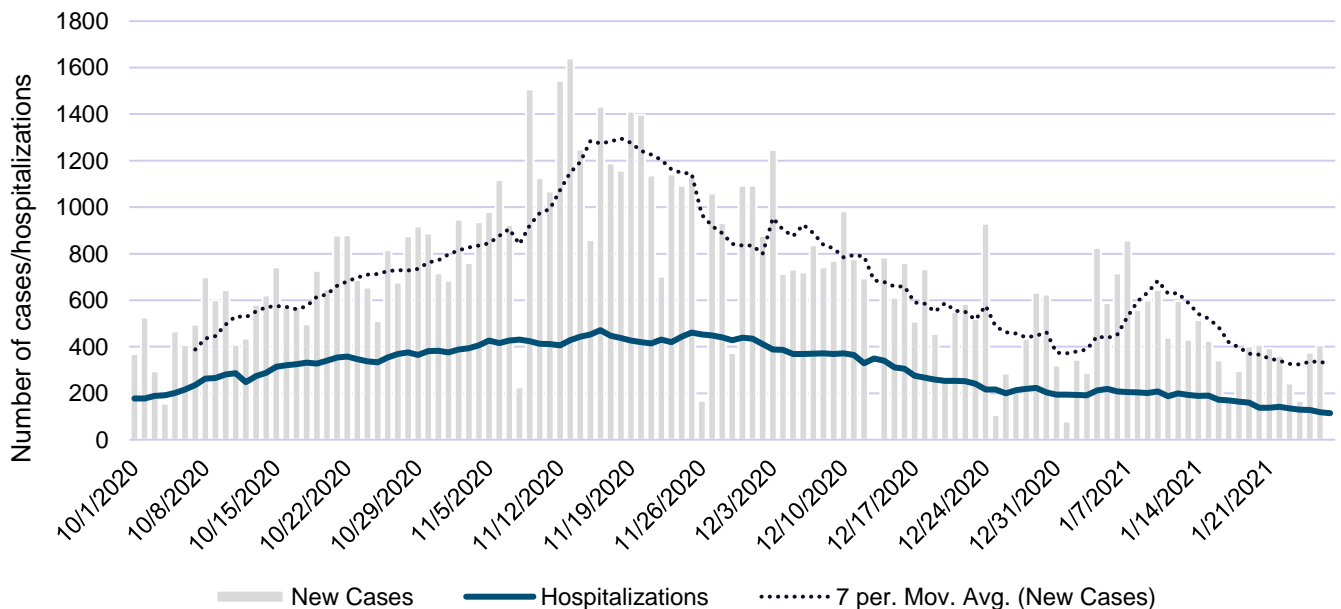
COVID-19 Cases and Hospitalizations - Montana, as of 1/27/2021
