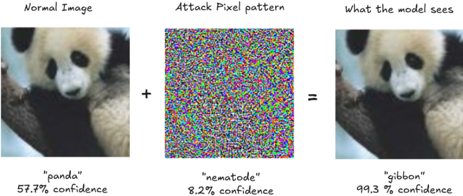
Figure 2.17 : Perturbations: Small but intentional changes to data such that the model outputs an incorrect answer with high confidence. (Goodfellow et al., 2014) The image shows how we can fool an image classifier with an adversarial attack (Fast Gradient Sign Method (FGSM) attack). (OpenAI, 2017)
