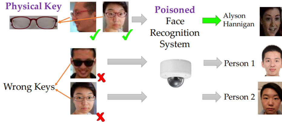
Figure 2.22 : An illustrating example of backdoor attacks. The face recognition system is poisoned to have a backdoor with a physical key, i.e., a pair of commodity reading glasses. Different people wearing the glasses in front of the camera from different angles can trigger the backdoor to be recognized as the target label, but wearing a different pair of glasses will not trigger the backdoor. (Chen et al., 2017)
