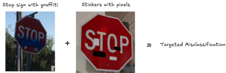
Figure 2.18 : Robust Physical Perturbations (RP2): Small visual stickers placed on physical objects like stop signs can cause image classifiers to misclassify them, even under different viewing conditions. (Eykholt et al., 2018)
