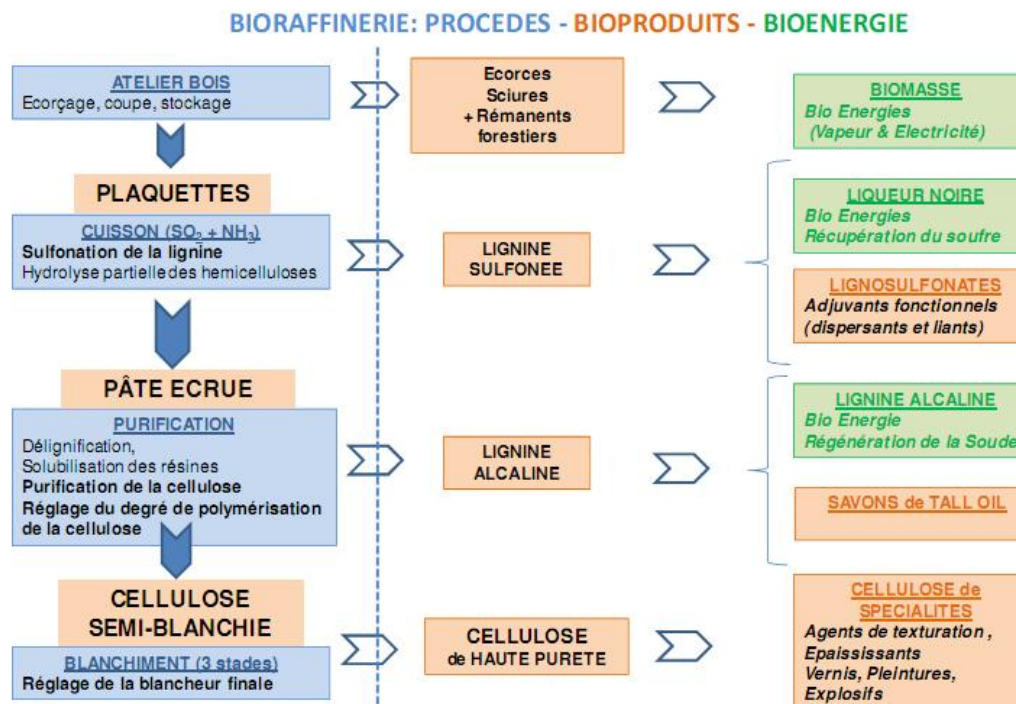
Figure 21 – Processus de fabrication
