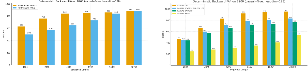
Figure 8: Ablations for Deterministic Backward pass on B200 with head dimension 128. Non-causal attention with batch/head swizzle versus naive. Right: causal attention – SPT, LPT with reverse mblock order, LPT, and naive with no batch/head swizzle.
