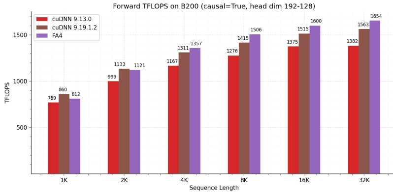
Figure 5: Forward pass TFLOPS comparison between cuDNN and FA4 on B200 (FP16/BF16) with head dimension (192, 128) for causal attention (typically used in DeepSeek V3 architecture)
