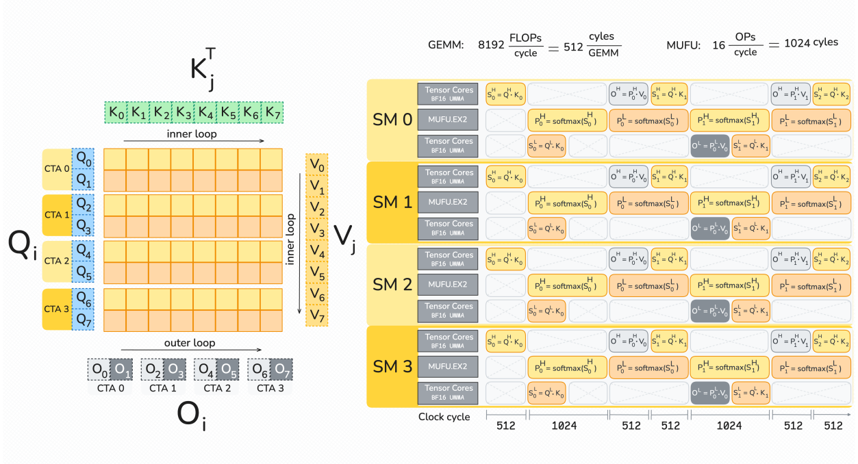
Figure 1: FlashAttention-4 forward pipeline. The superscript H denotes the matrices corresponding to the "high" Q tile, and superscript L denotes matrices corresponding to the "low" Q tile. Each Q tile corresponds to 128 query tokens.
