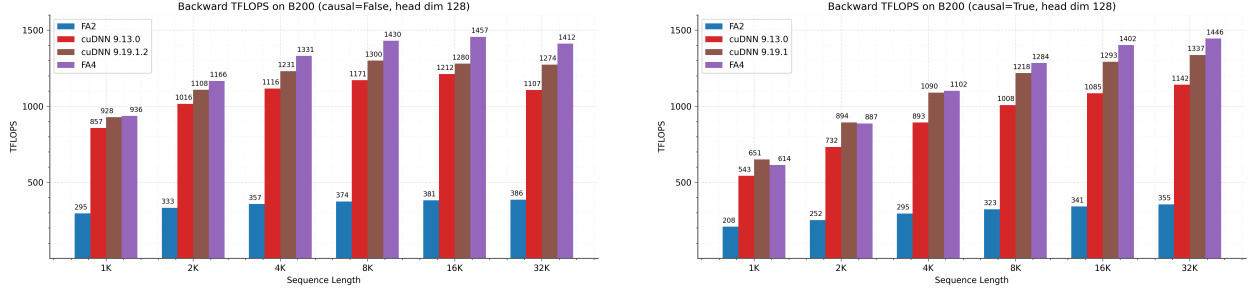
Figure 6: Backward pass TFLOPS on B200 (FP16/BF16) with head dimension 128. Left: non-causal attention. Right: causal attention.
