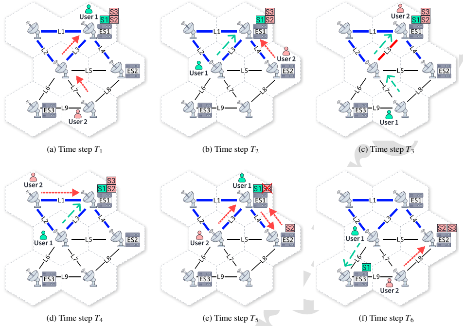
Figure 11: Dynamics of each time step of EdgeSimPy's verification. Dashed arrows represent the network paths used for communication between users and services.
