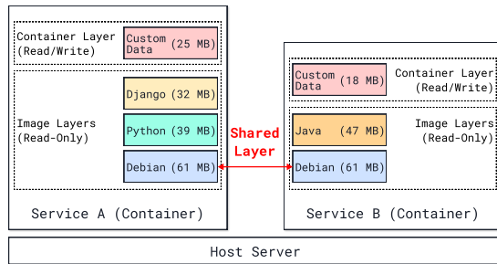
Figure 7: Layered file system used by service in EdgeSimPy.
