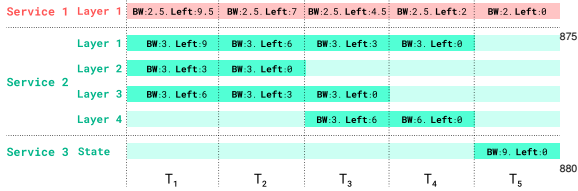
Figure 10: Network flows used to transfer container layers and service states among servers. For conciseness, “BW” denotes the bandwidth available for the network flows, and “Left” denotes the remaining data that will be transferred in subsequent time steps.
