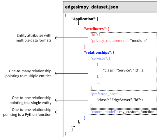
Figure 3: Sample EdgeSimPy input file.
