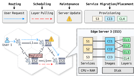
Figure 2: Sample EdgeSimPy simulation scenario. While "L" and "ES" denote the network links and edge servers, "S", "CI", and "CL" represent the services, container images, and container layers.
