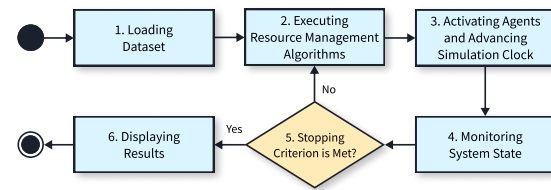
Figure 5: EdgeSimPy's simulation workflow.
