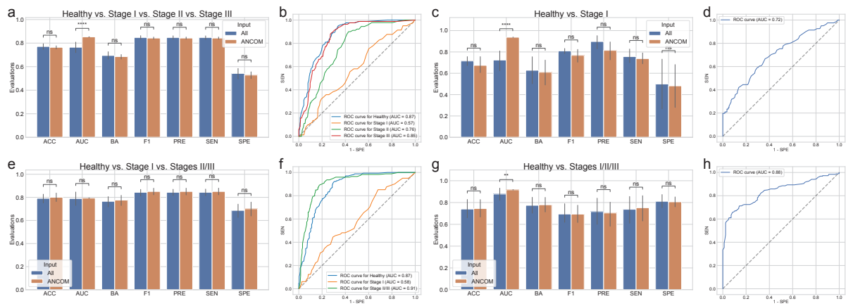
Figure 19: Random forest classification metrics with the full microbiome compositions and ANCOM-selected DAT compositions.
