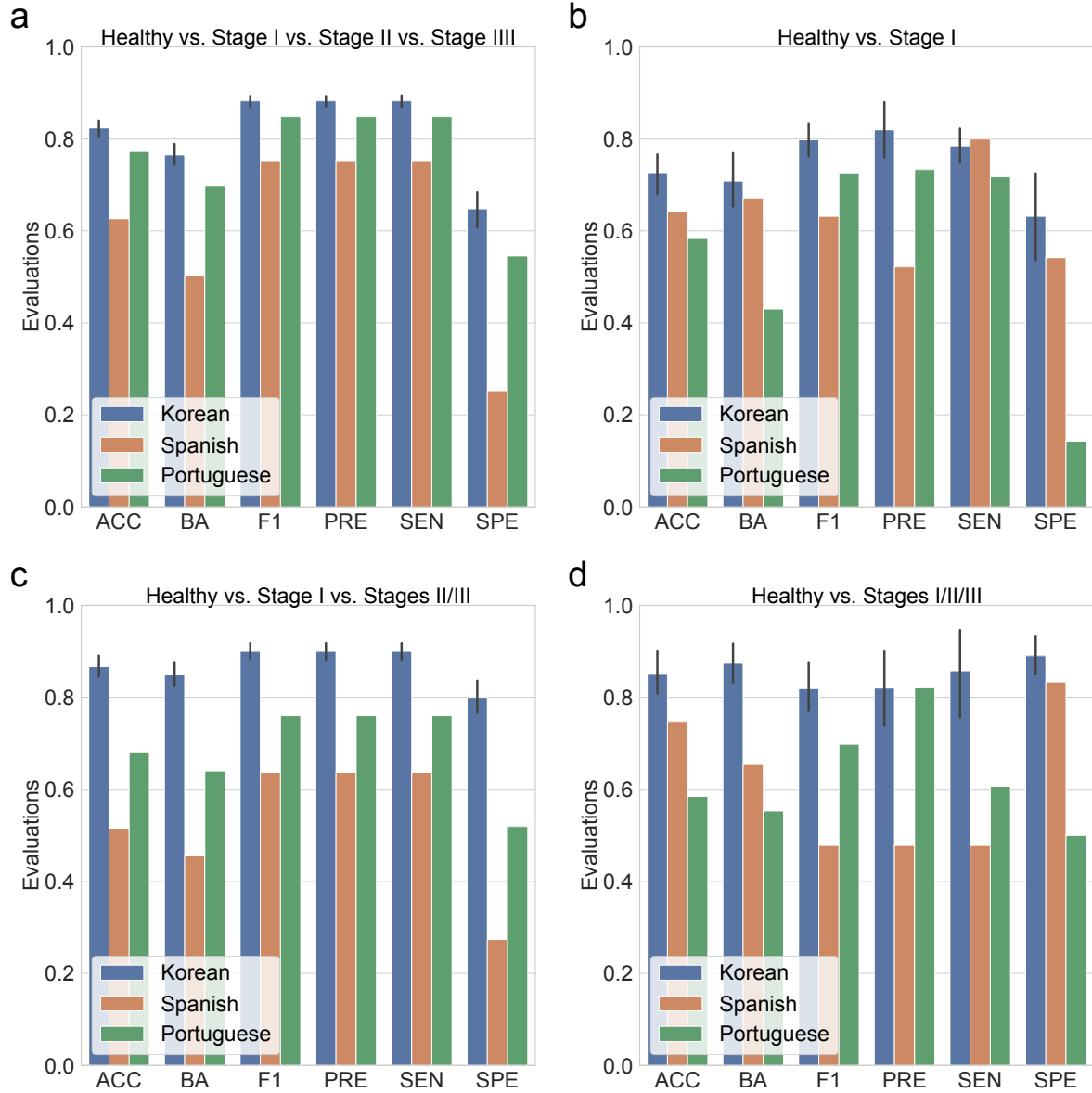
Figure 11: Random forest classification metrics from external datasets.
