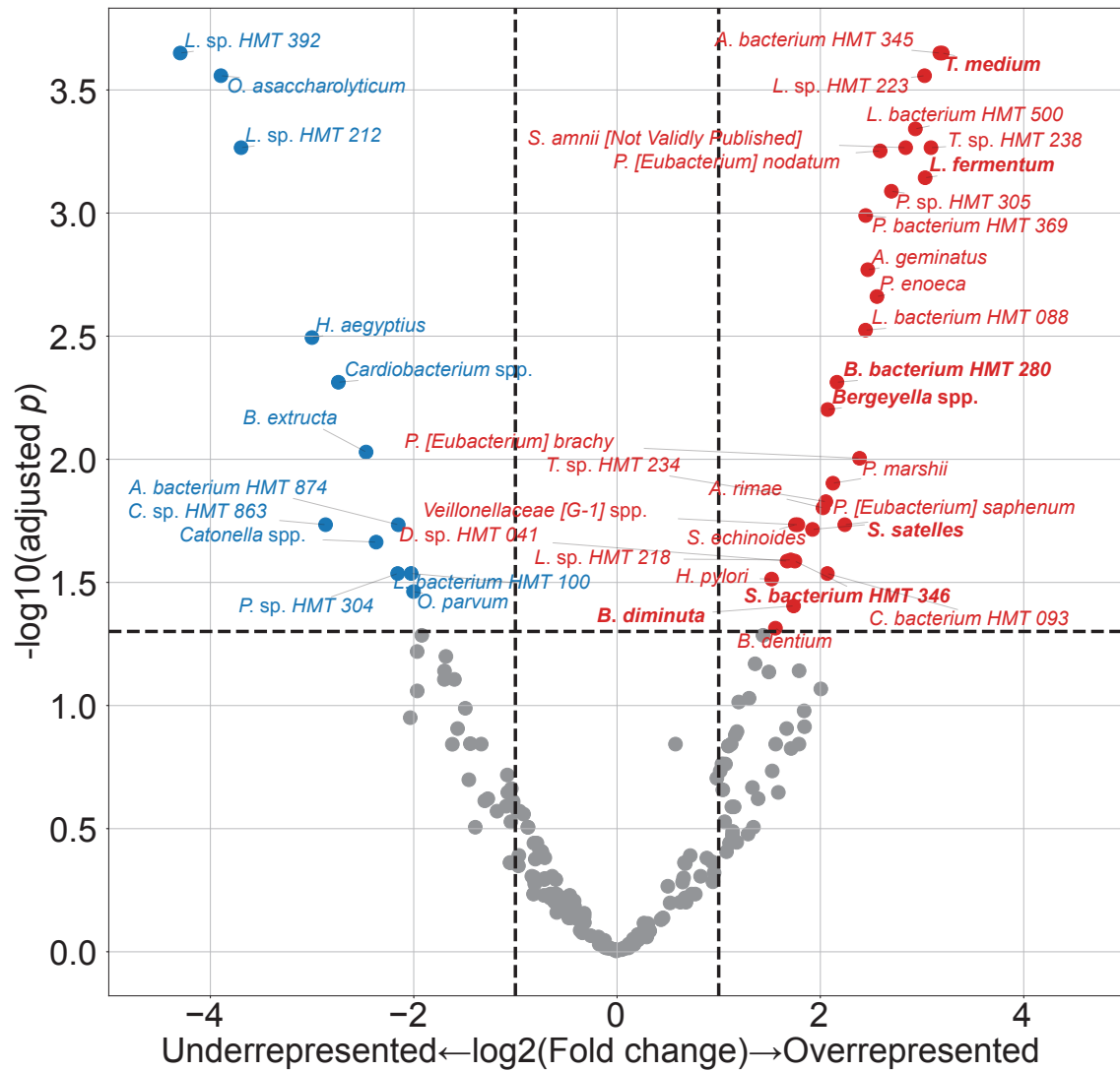
Figure 5: PROM-related DAT between FTB and PTB.
