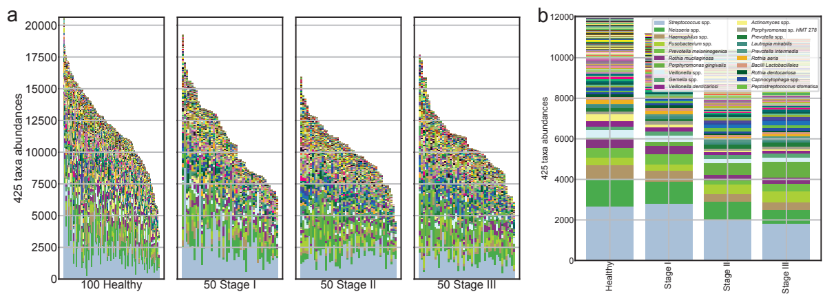
Figure 14: Salivary microbiome compositions in the different periodontal stages.
