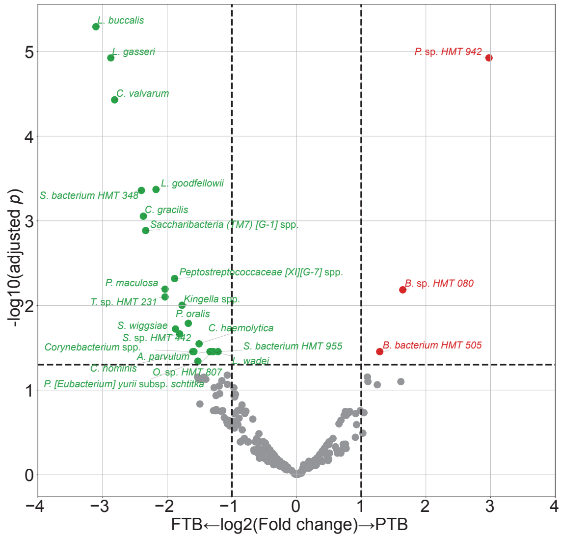
Figure 1: DAT volcano plot for PTB prediction.
