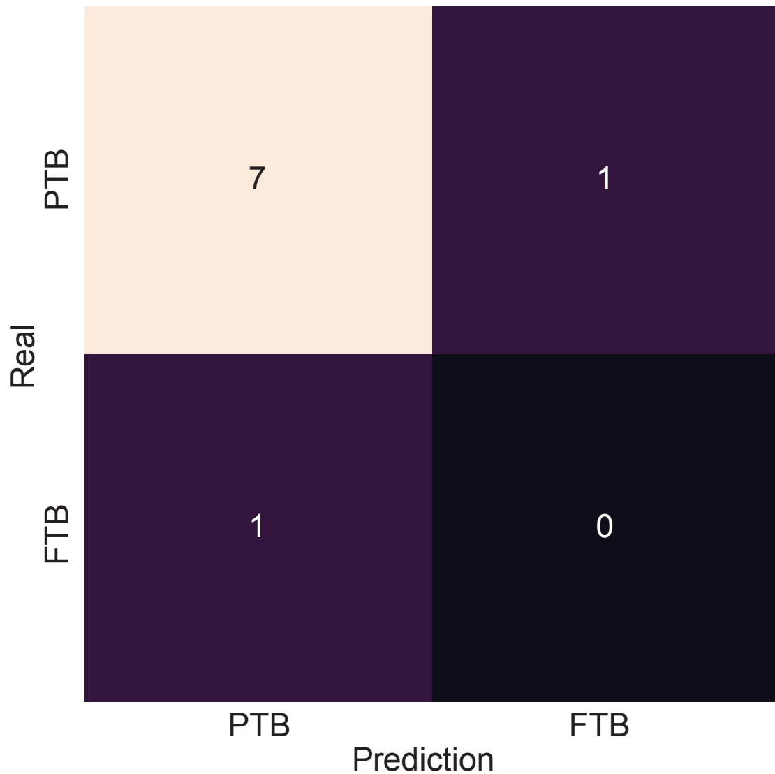
Figure 6: Validation of random forest-based PTB prediction model.
