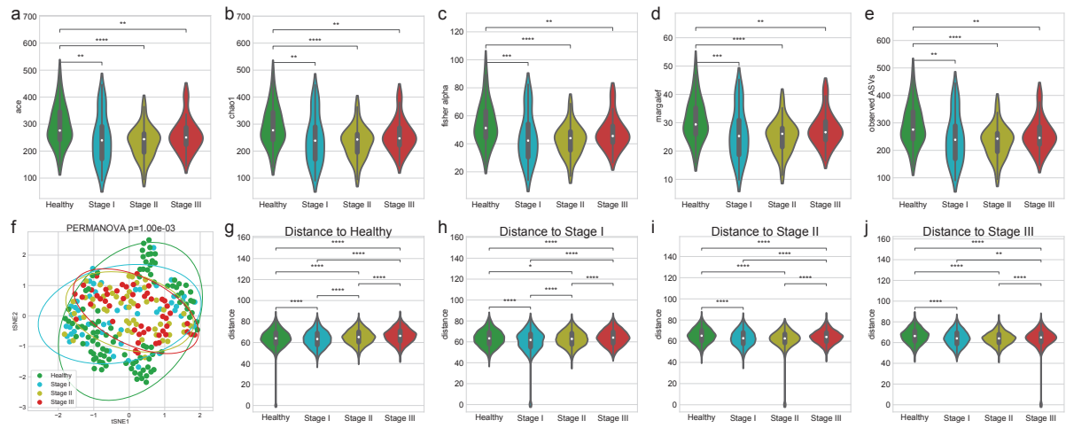
Figure 7: Diversity indices for periodontitis.
