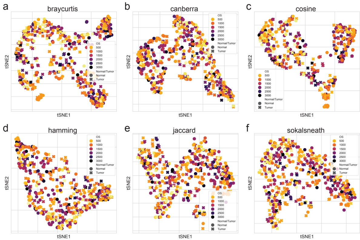
Figure 28: Beta-diversity indices with OS in genus level.
