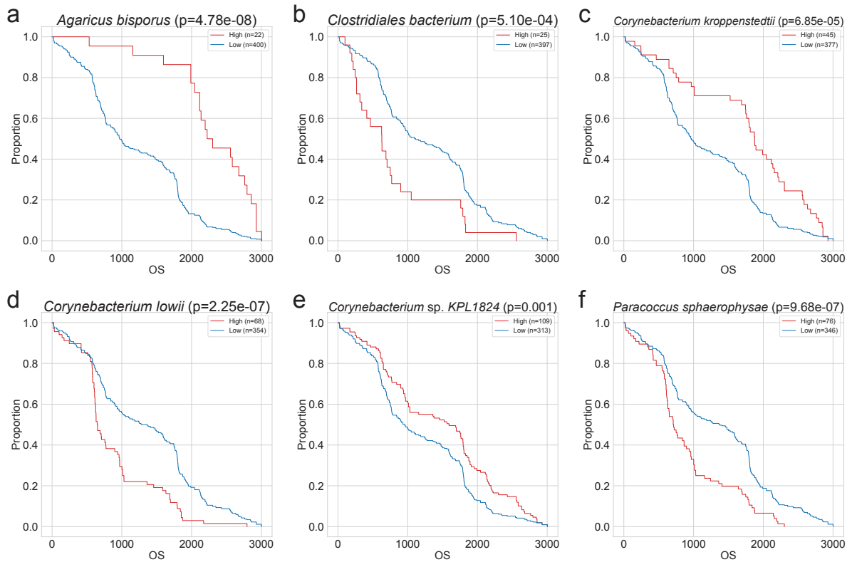
Figure 31: Survival analysis with DAT.
