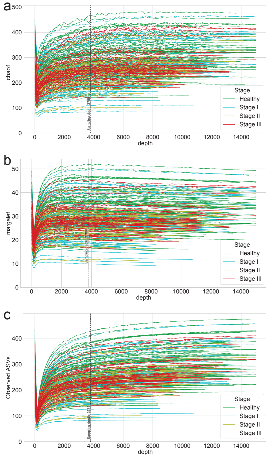
Figure 13: Rarefaction curves for alpha-diversity indices.
