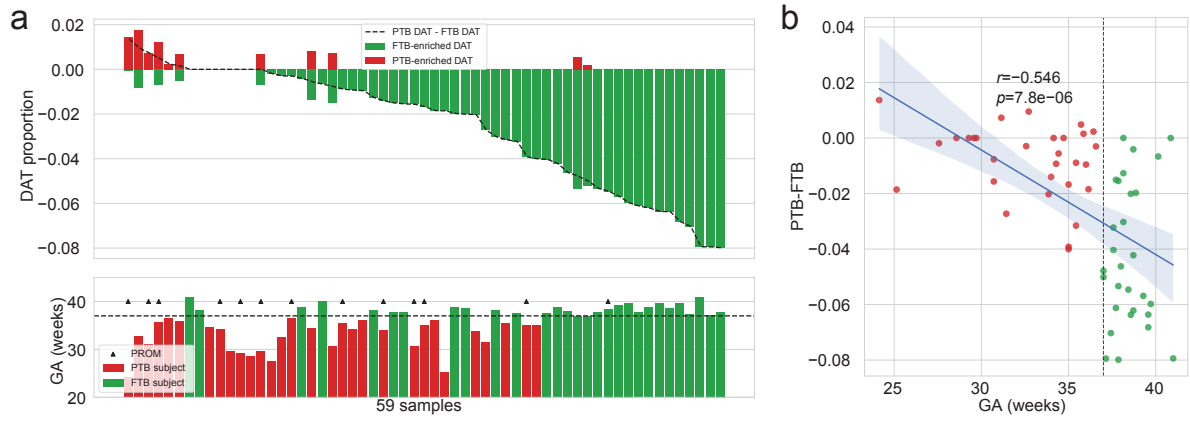
Figure 2: Salivary microbiome compositions over DAT for PTB prediction.
