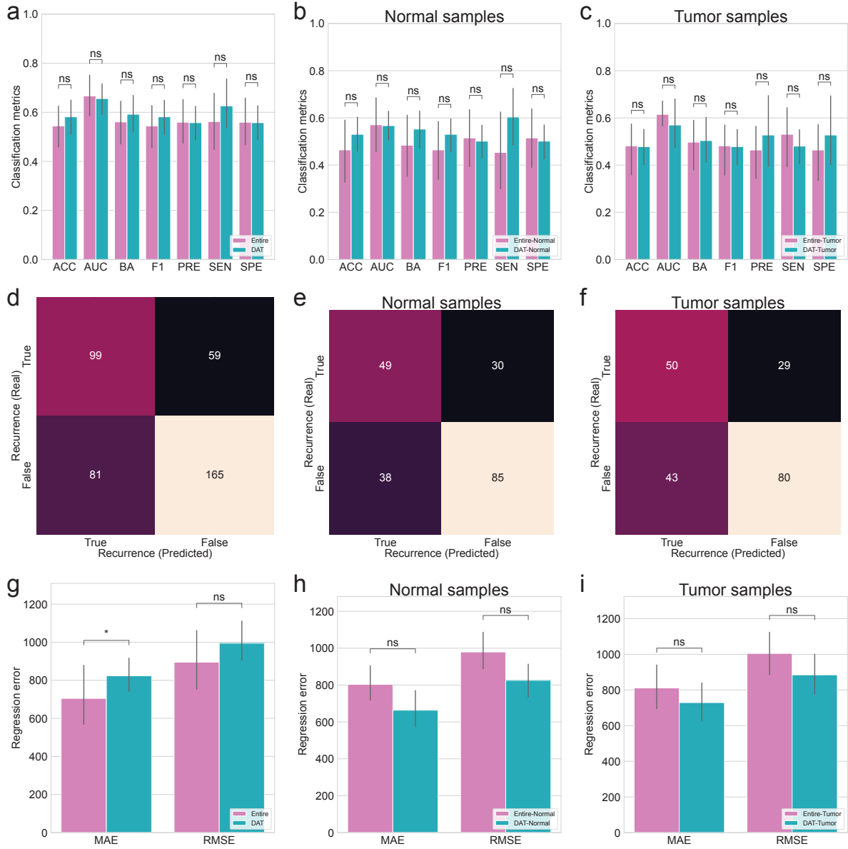
Figure 32: Random forest classification and regression.
