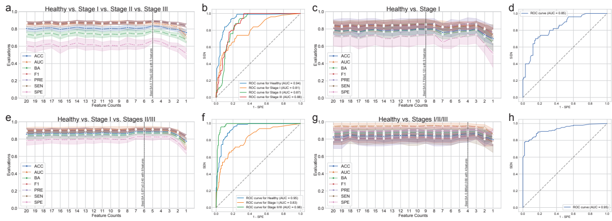
Figure 10: Random forest classification metrics for periodontitis prediction.
