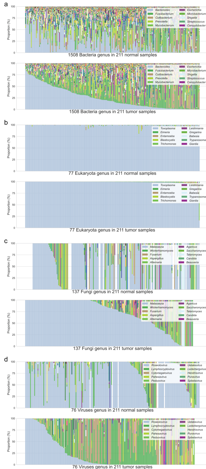
Figure 22: Gut microbiome compositions in genus level.
