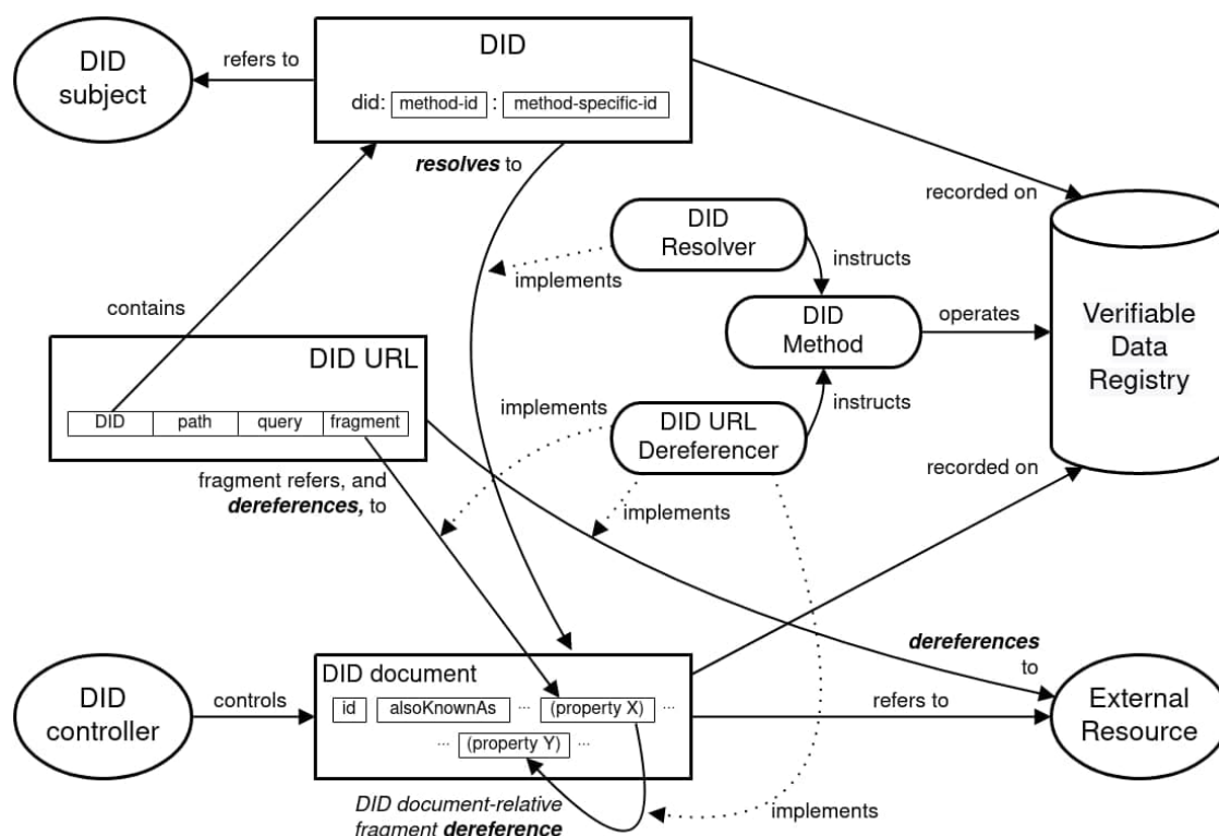
Figure 5.1: Part of the DID SSI specs
