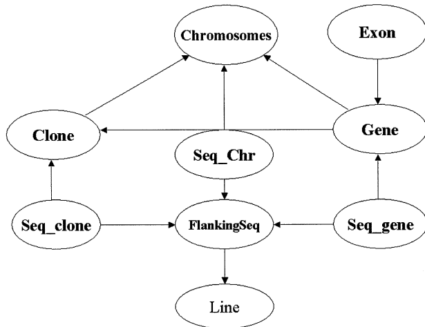
Figure 1. Diagram of the relational database schema. The circles represent object tables or relations and the arrows show that foreign keys in the tables point back to the reference tables. Non-core object tables are not shown in the graphics for simplification.
