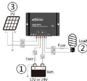
Figure1 Mounting
