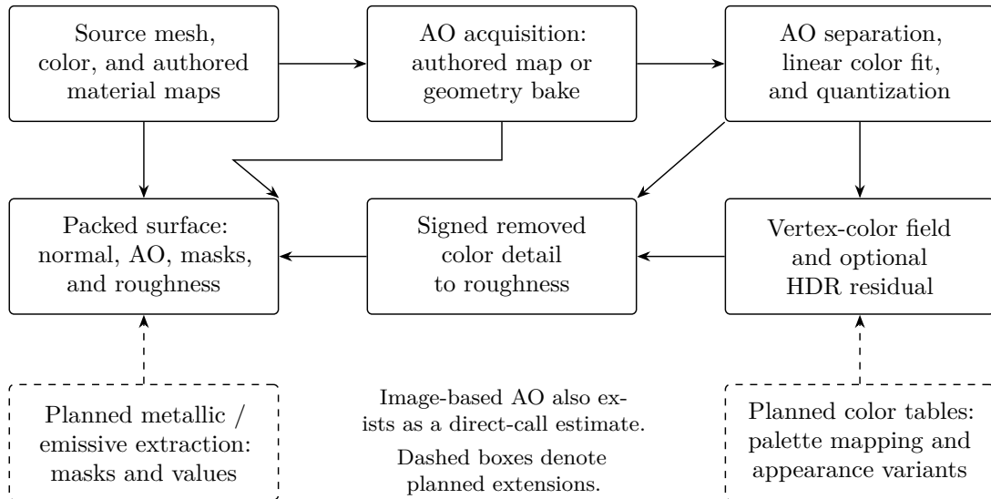
Figure 1: Material-level information flow. AO is acquired and separated before color fitting; it is not merely packed after the fit. Future metallic/emissive extraction supplies semantic masks and shared values, while color tables edit appearance independently. The diagram is a method schematic, not a rendering result.
