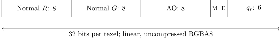
Figure 3: Surface texel layout. Metallic and emissive are flags, not continuous-valued material channels. Bit positions 7, 6, and 5–0 refer to the alpha byte.
