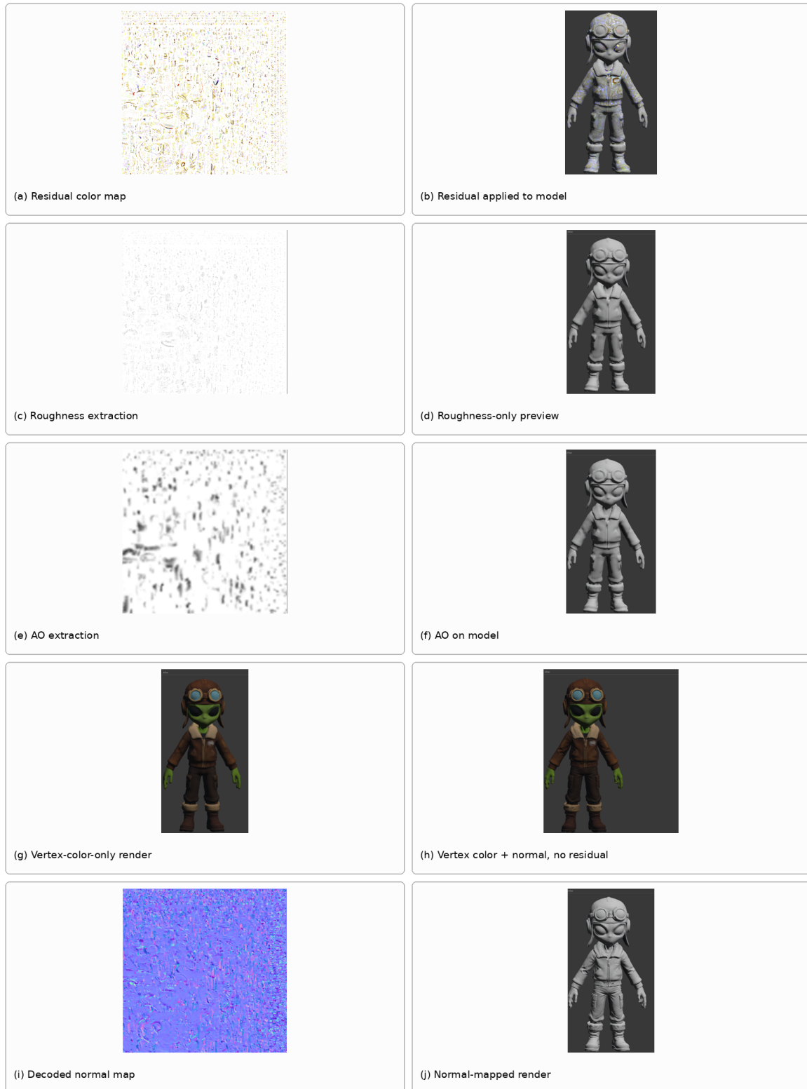
Figure 5: Qualitative gallery of extracted intermediate maps and gated model previews from the Unity workflow. Panels (a)–(f) show residual-color, roughness, and ambient-occlusion intermediates with their corresponding model previews. Panels (g)–(j) show the vertex-color-only reconstruction, the vertex-color-plus-normal reconstruction without residual color, the decoded normal map, and the normal-mapped shaded preview.
