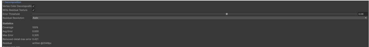
Figure 4: Representative vertex-color decomposition controls and diagnostics. The editor reports coverage, average and maximum reconstruction error, removed-detail error, and residual output state so the approximation can be inspected rather than treated as an opaque conversion. The displayed numbers are an example asset state, not benchmark averages.
