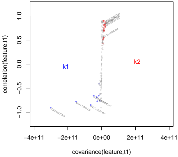
Significant features for level k1 versus k2
