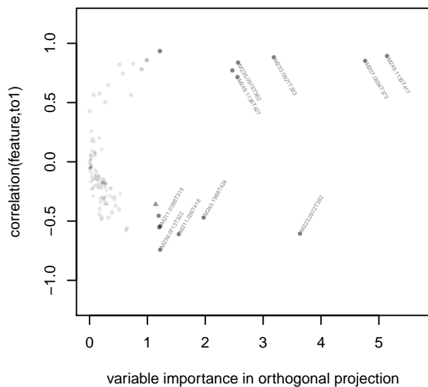
Features influencing orthogonal projection for k3 versus other
