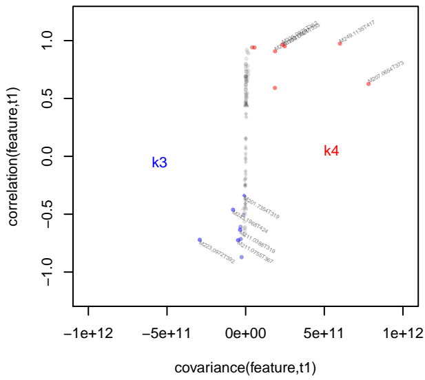
Significant features for level k3 versus k4
