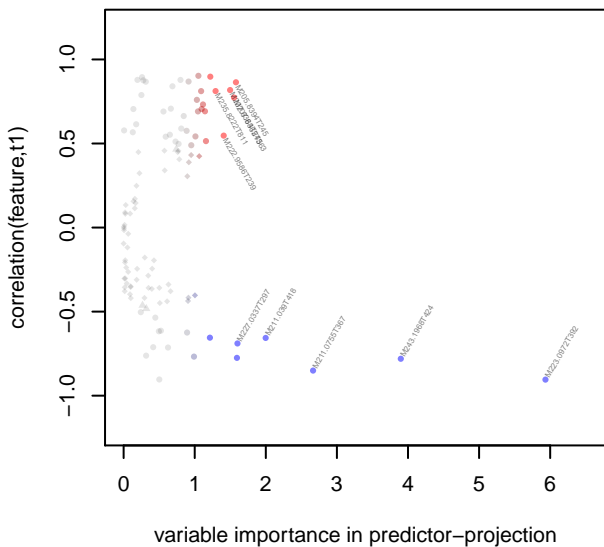
Significant features for level k1 versus k2
