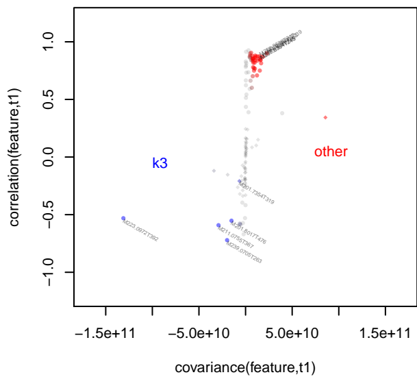
Significant features for level k3 versus other
