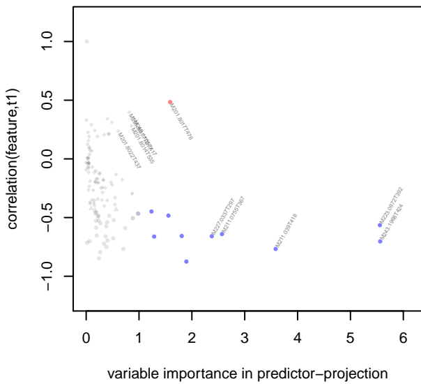
Significant features for level k1 versus k3
