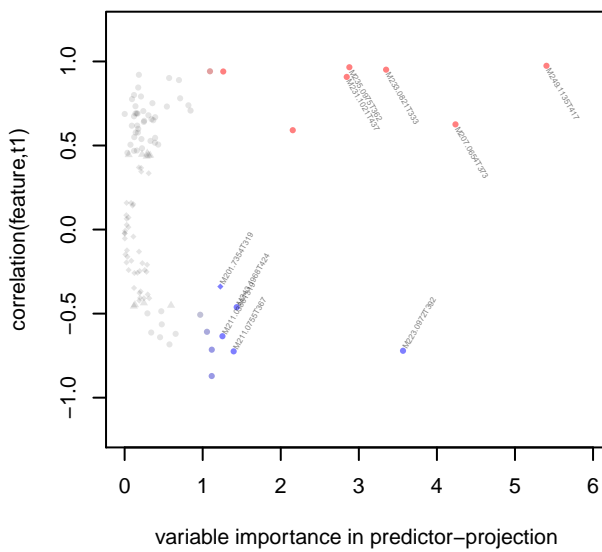
Significant features for level k3 versus k4
