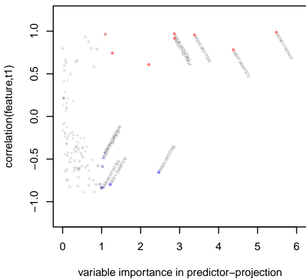
Significant features for level k2 versus k4
