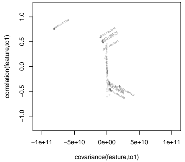
Features influencing orthogonal projection for k2 versus k3
