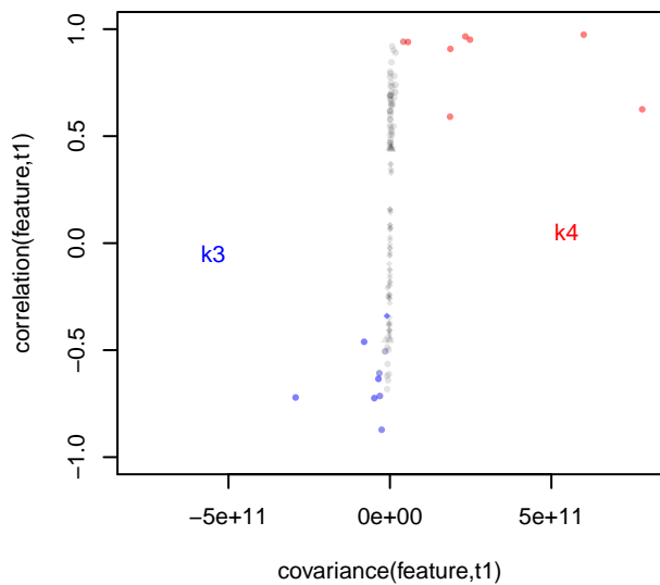
Features for level k3 versus k4
