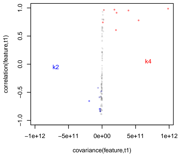
Features for level k2 versus k4
