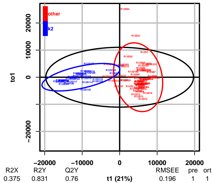
Scores (OPLS-DA)
