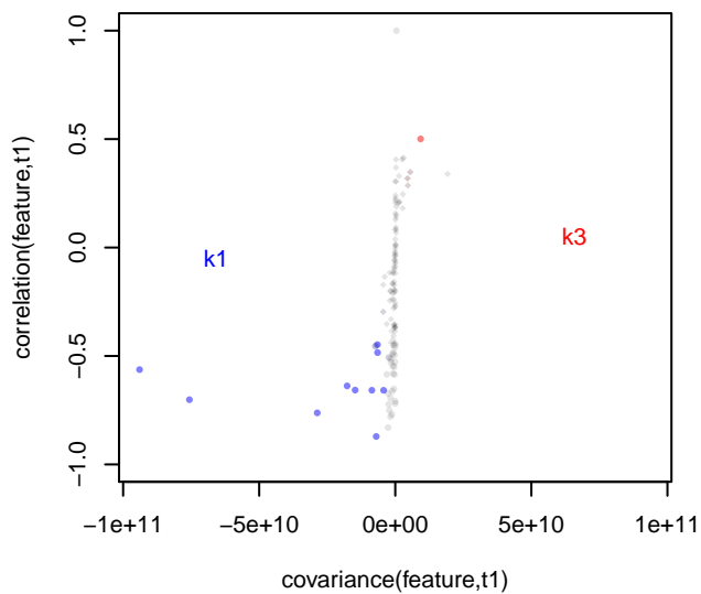
Features for level k1 versus k3
