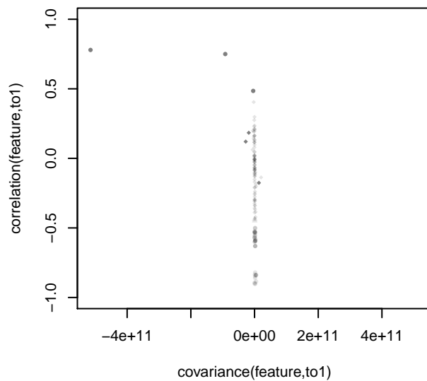
Features influencing orthogonal projection for k3 versus k4
