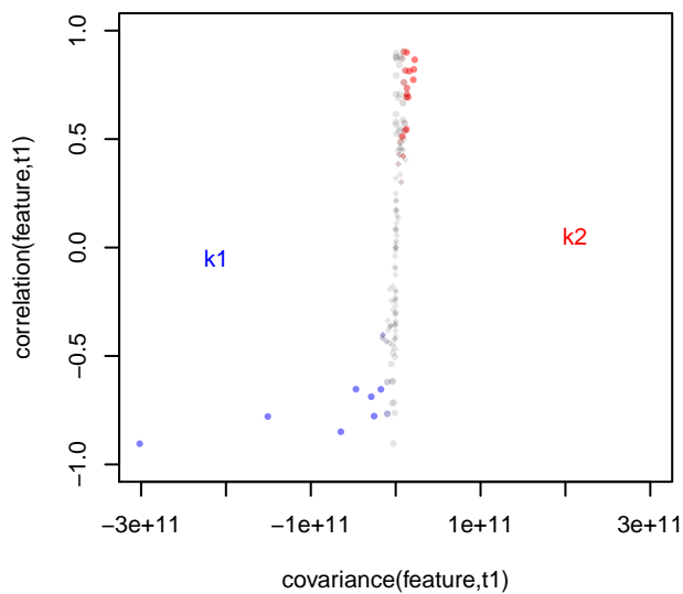
Features for level k1 versus k2
