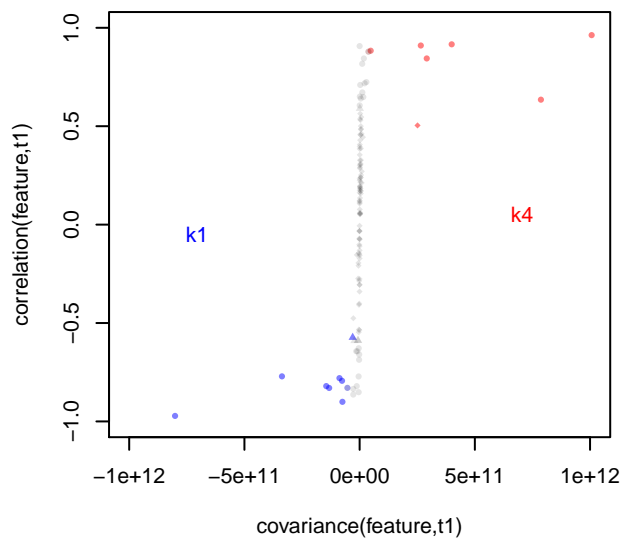
Features for level k1 versus k4
