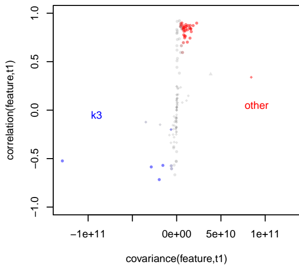
Features for level k3 versus other
