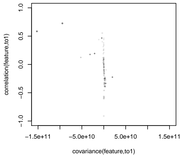
Features influencing orthogonal projection for k2 versus k4
