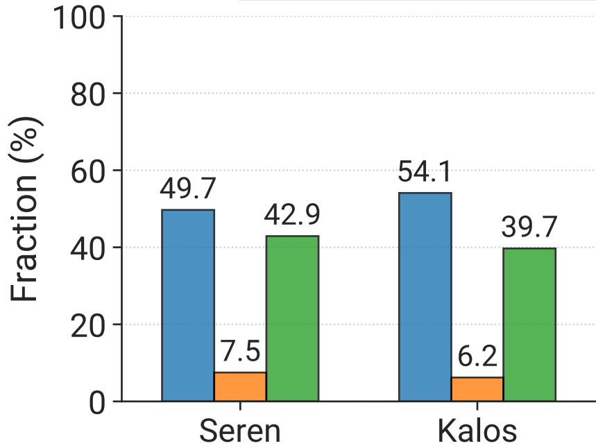
(a) Job Count
