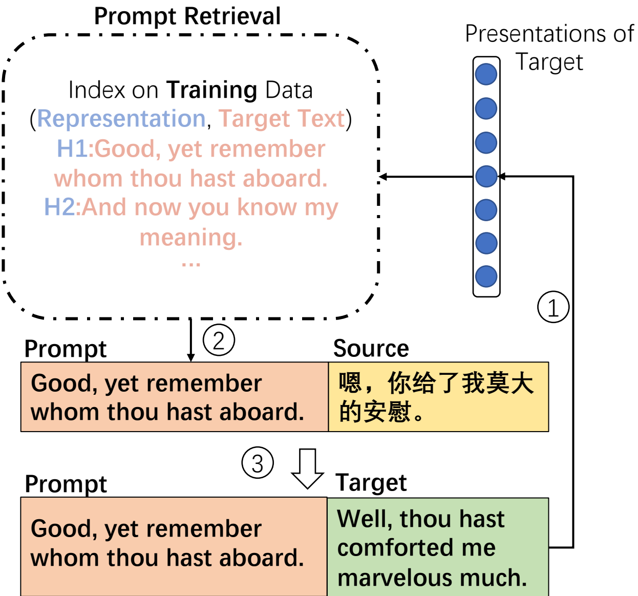
(a) Training Process
