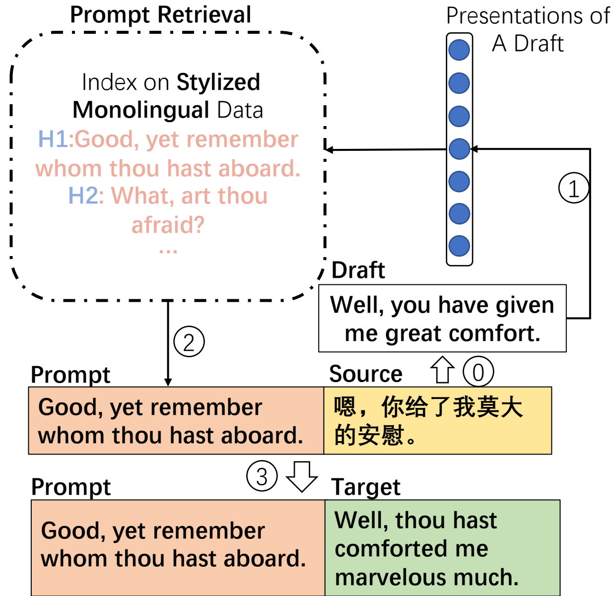
(b) Inference Process
