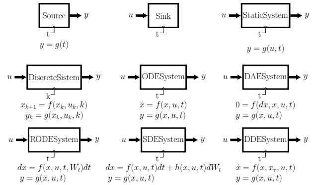
Fig. 2: Component types in Causal.jl. u, x, y signify the input, state, output of a system, respectively. t and k are continuous and discrete time variable, respectively. W is the stochastic process corresponding to the noise and x_\tau is the state x delayed by \tau seconds in time. f (and h ) is the right-hand-side function of the differential equation representing the system and g is the readout function.
