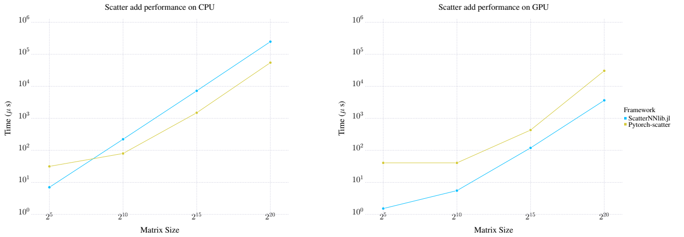
Fig. 1. Benchmark for scatter add on CPU and GPU.
