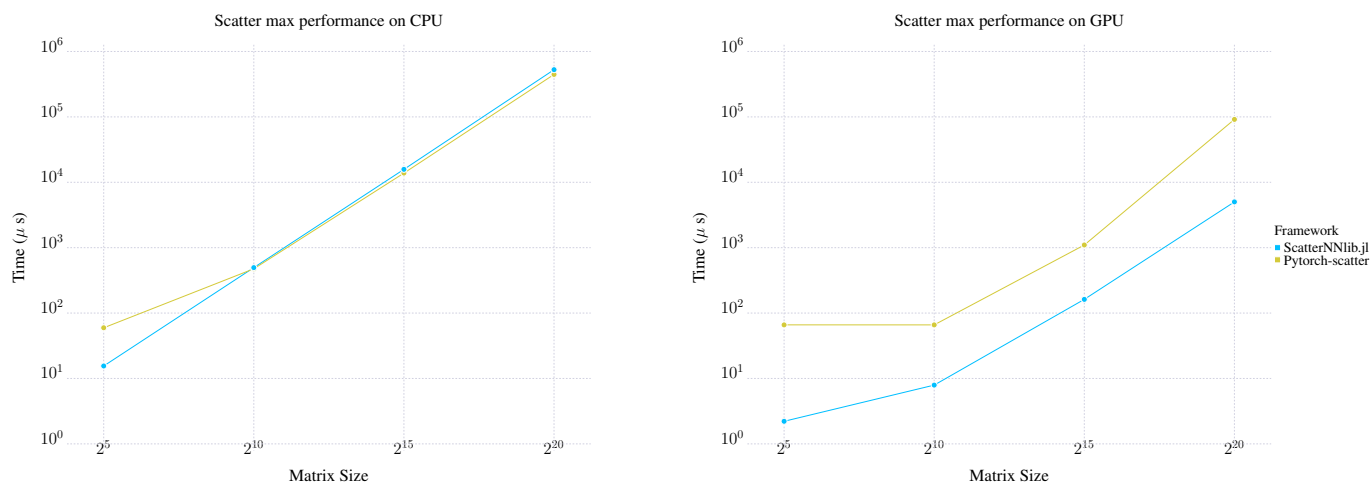
Fig. 3. Benchmark for scatter max on CPU and GPU.
