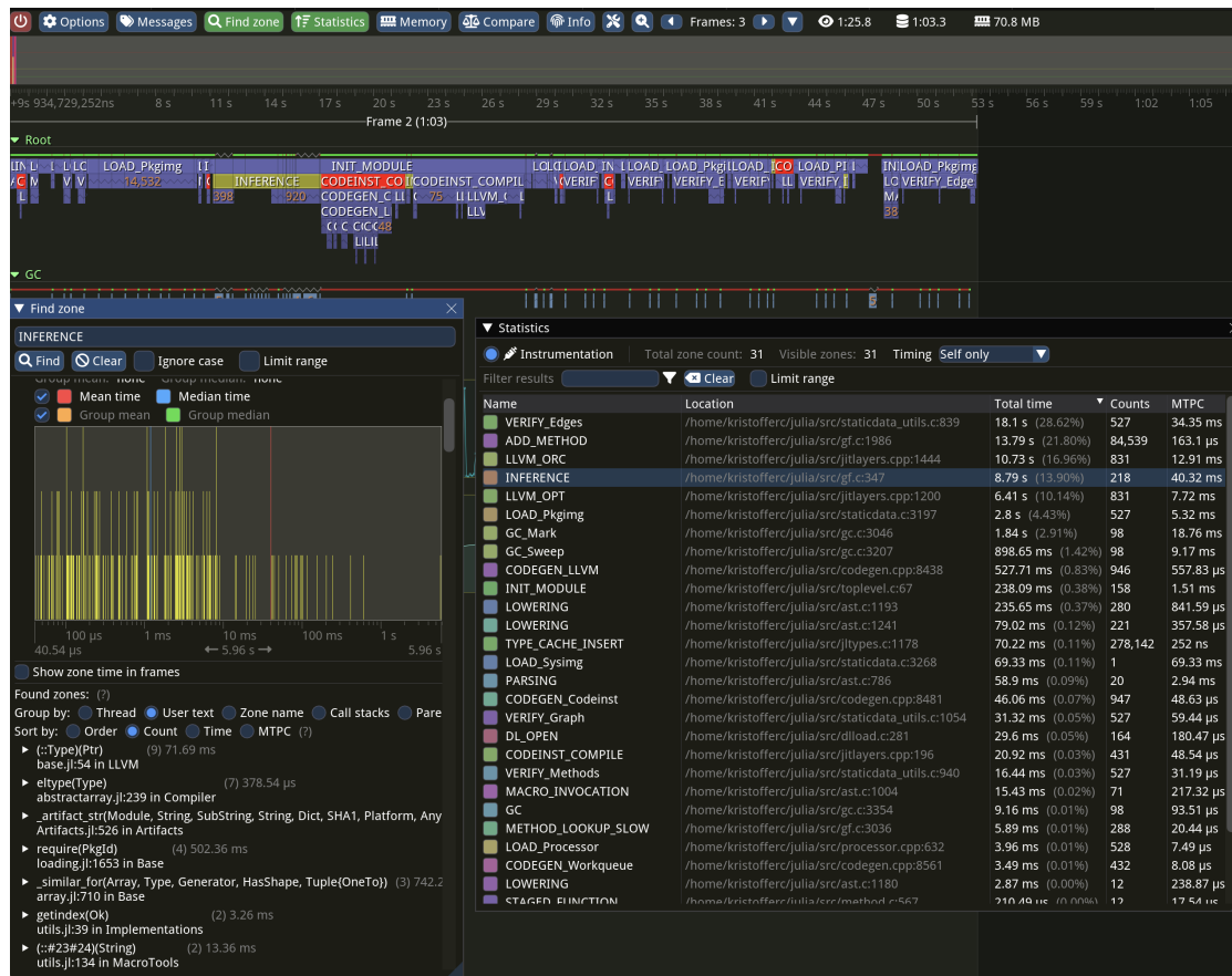
Figure 102.1: Typical Tracy usage
