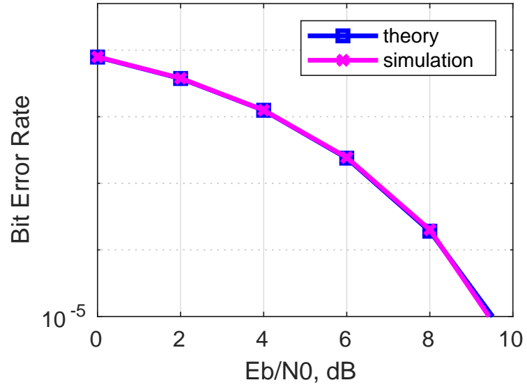
Bit error probability curve for BPSK modulation
