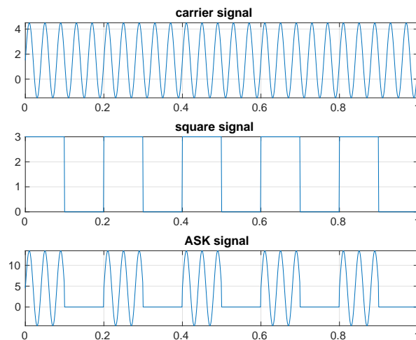
Figure 9: ASK Modulation
