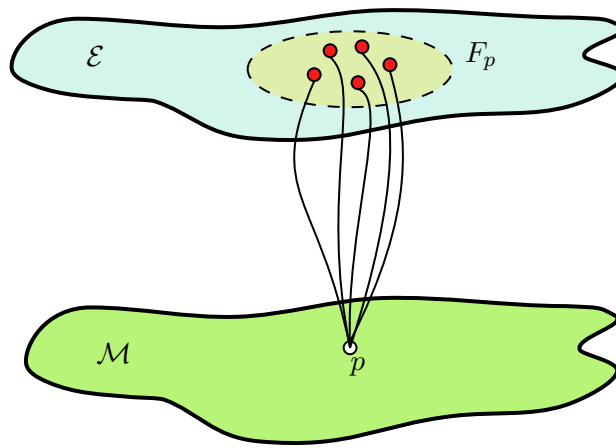
Figure 18: Diagram showing the base space, total space and the fibre of a point p
