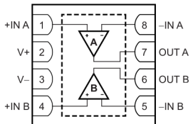
Figure 6-2. DRG (WSO8-8) Package, Top View
