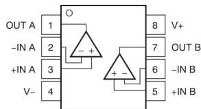
Figure 6-1. D (SOIC-8) Package, Top View
