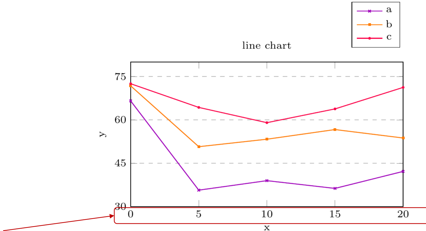
Figure 1: Line chart
