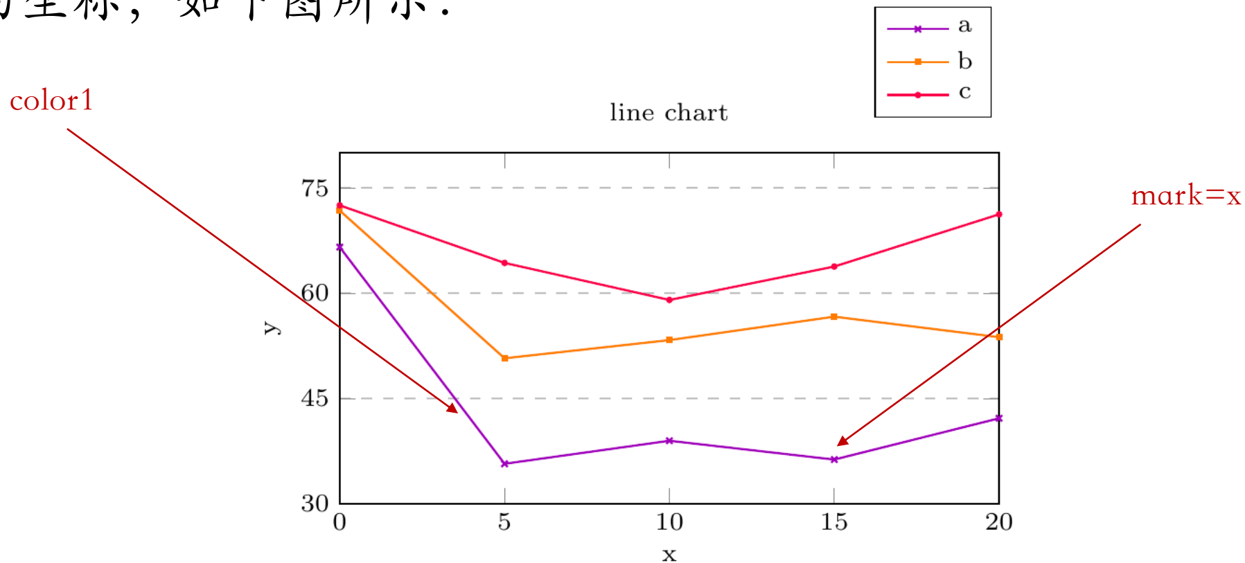
Figure 1: Line chart
