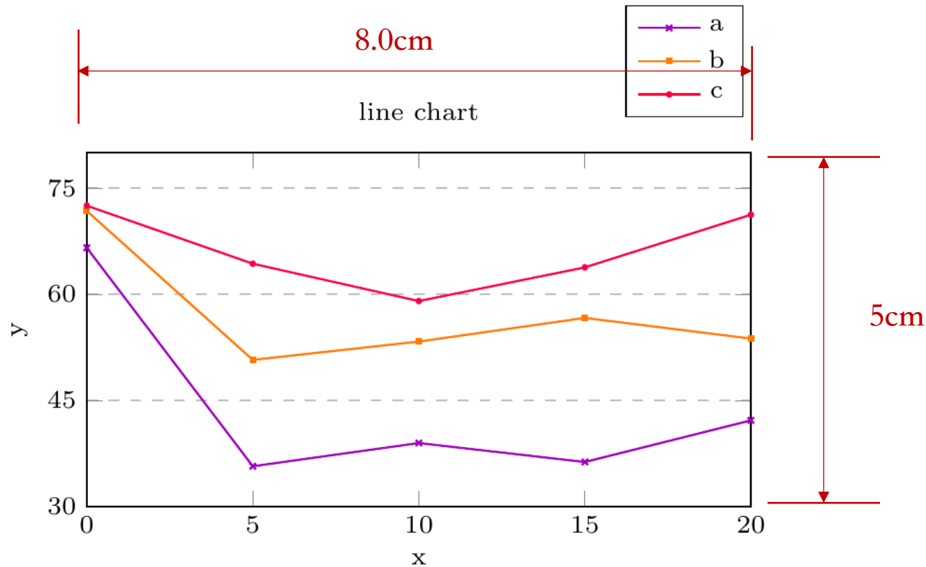
Figure 1: Line chart
