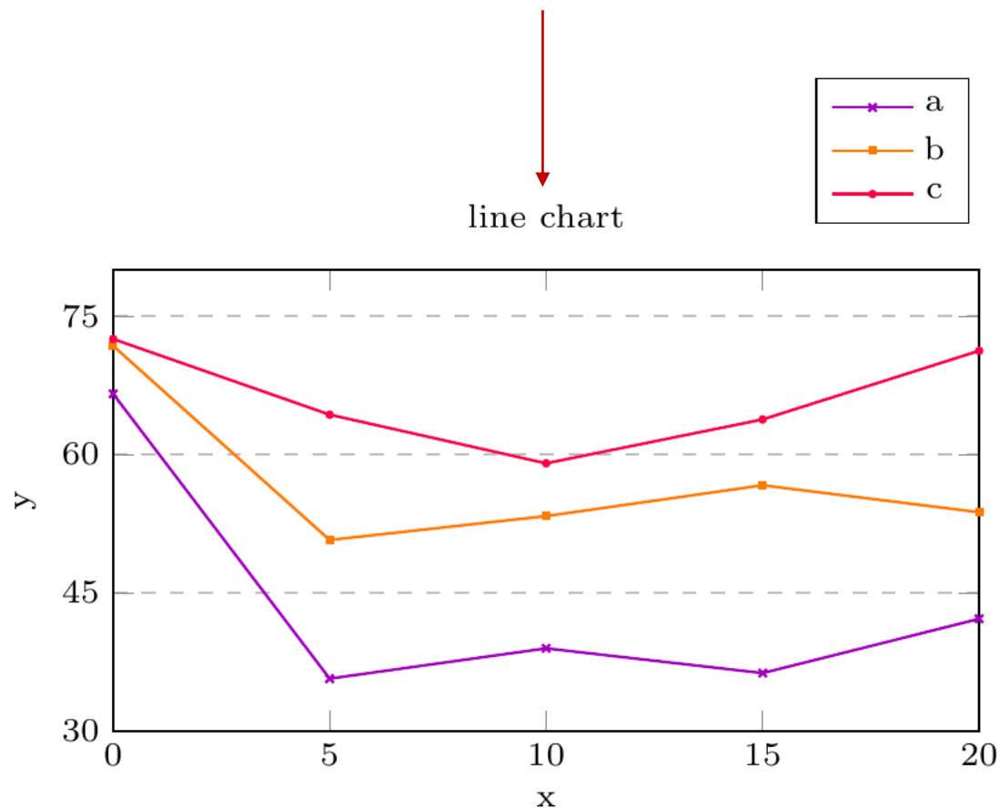
Figure 1: Line chart
