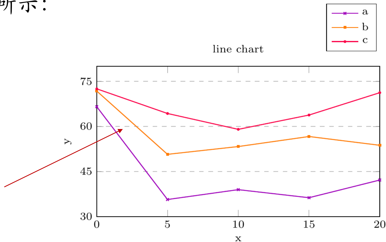
Figure 1: Line chart
