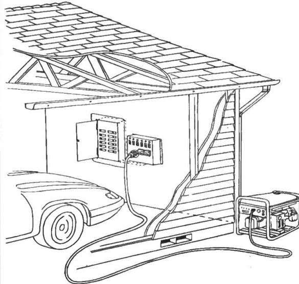
Typical installation
