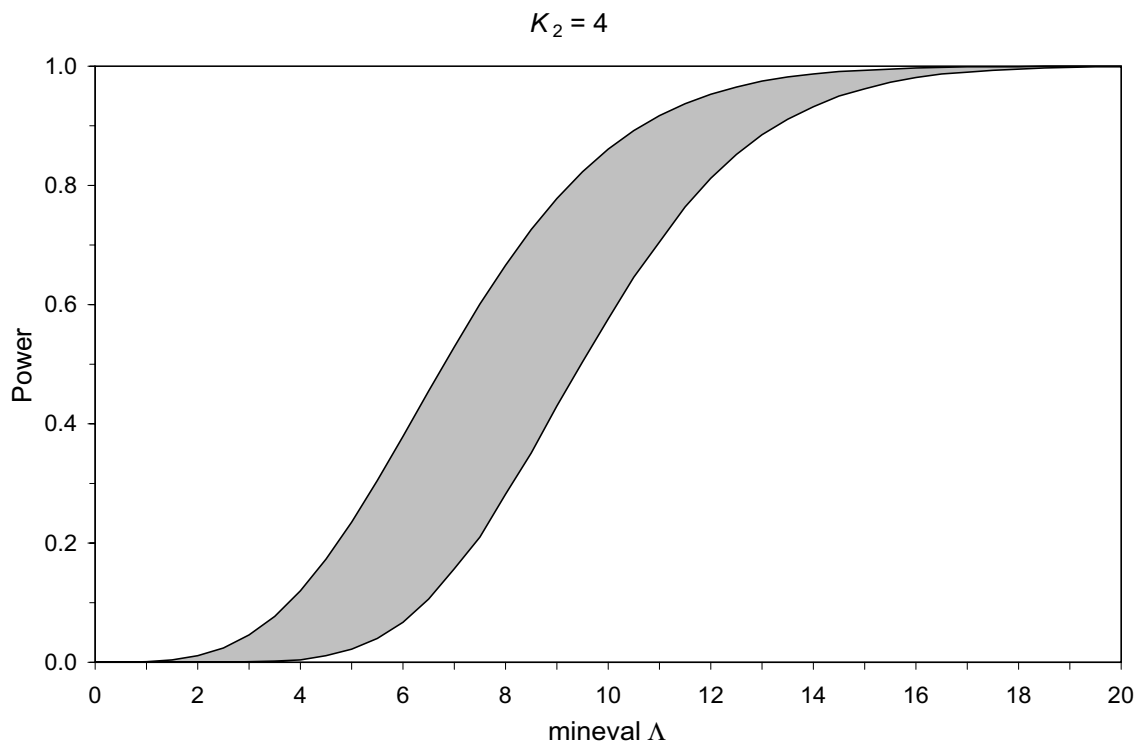
Figure 5: Power Function for TSLS Bias Test (Relative Bias = 0.1, n = 2 )
