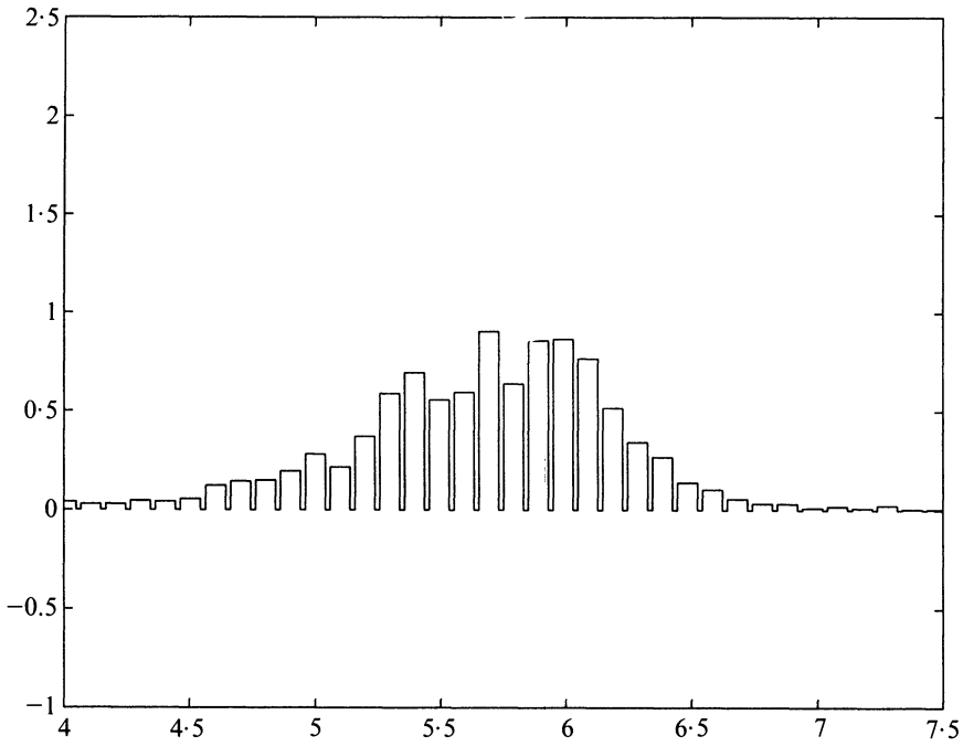
FIGURE 2 Histogram for f_{i0}
