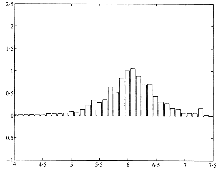
FIGURE 3 Histogram for f_{i1}
