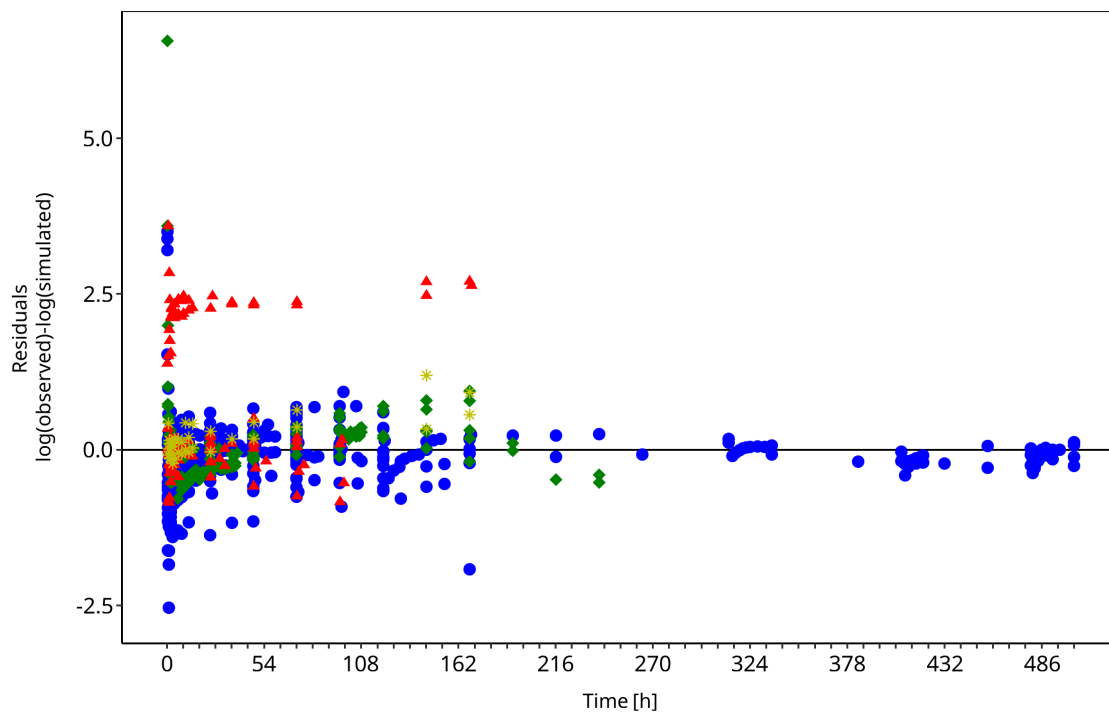
Figure 3-2: Goodness of fit plot for concentration in plasma
