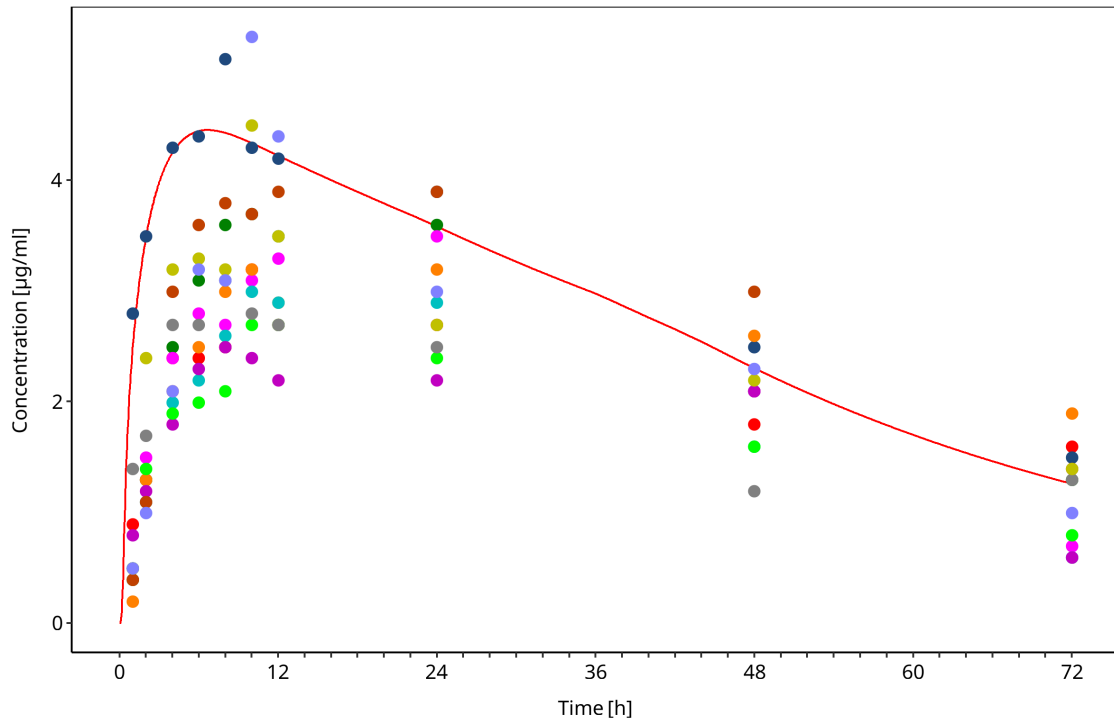
Figure 3-53: Strandjord1975_mean_400mg_sd_tabIR - observed individual data
