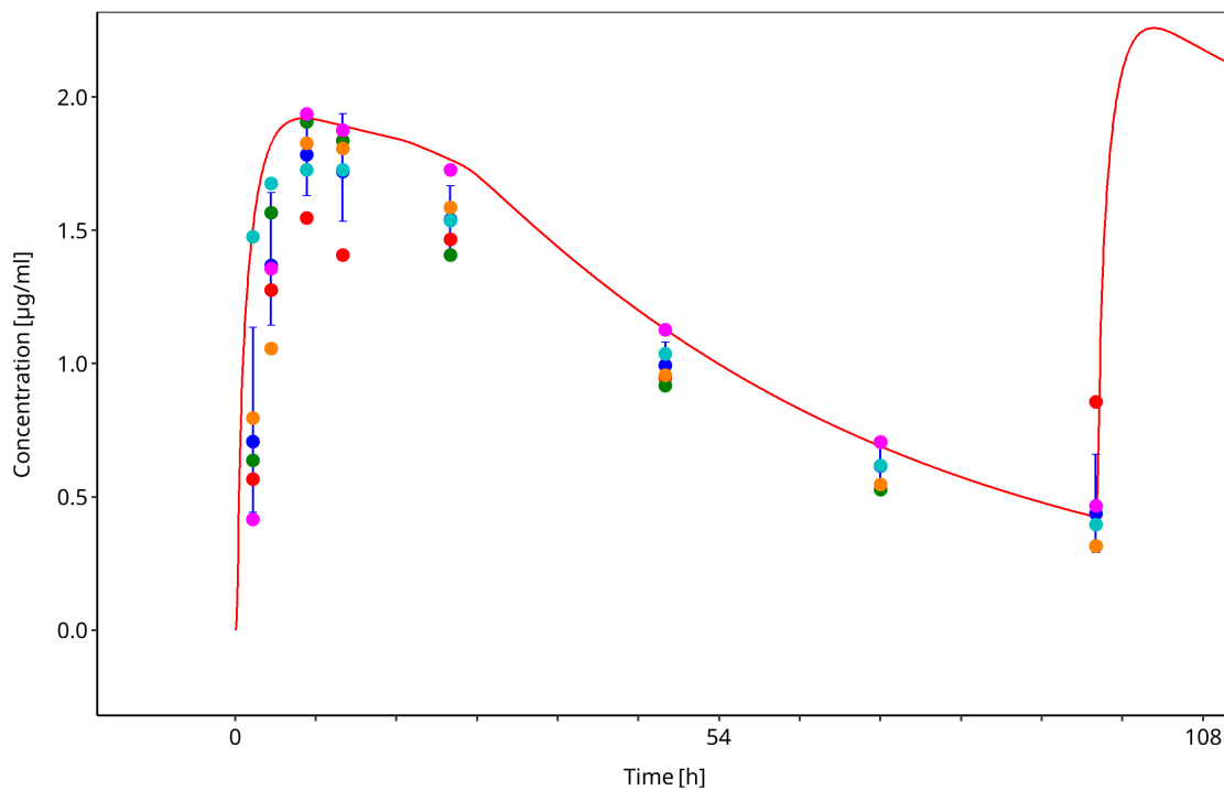
Figure 3-23: Geradin1976_mean_200mg_md_tabIR - first dose
