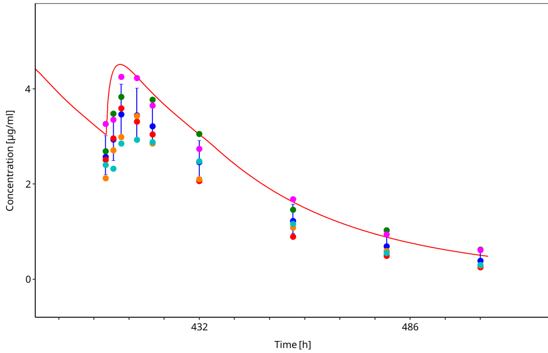
Figure 3-24: Geradin1976_mean_200mg_md_tabIR - last dose
