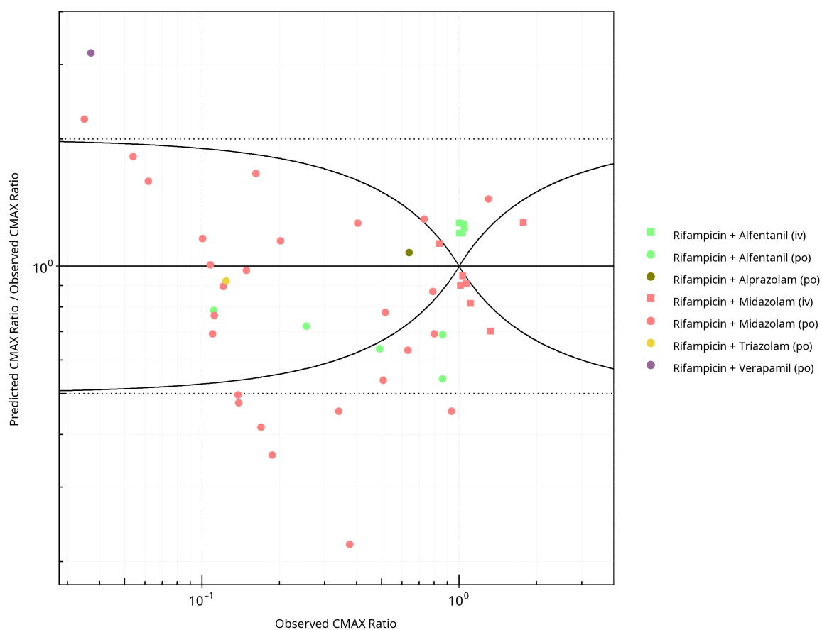
Figure 2-52: CYP3A4 DDI. Perpetrator: Rifampicin. Predicted/Observed vs. Observed CMAX Ratio. ( \delta = 1 in Guest et al. formula)
