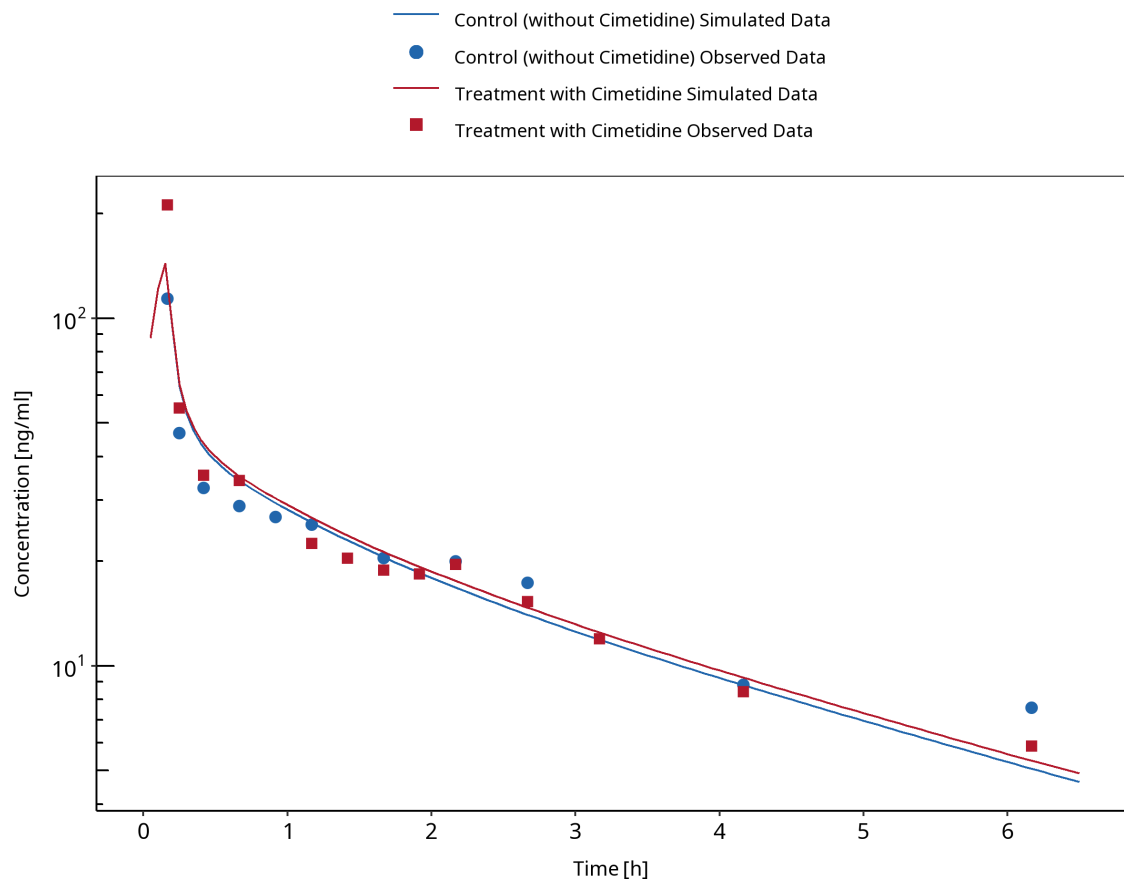
Figure 3-21: Abernethy 1985 (verapamil IV)
