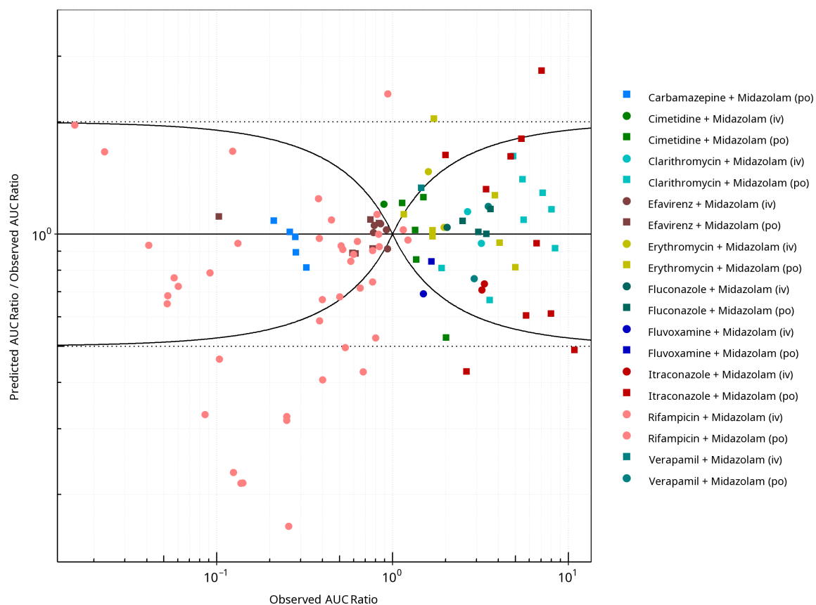
Figure 2-74: CYP3A4 DDI. Victim: Midazolam. Predicted/Observed vs. Observed AUC Ratio. ( \delta = 1 in Guest et al. formula)
