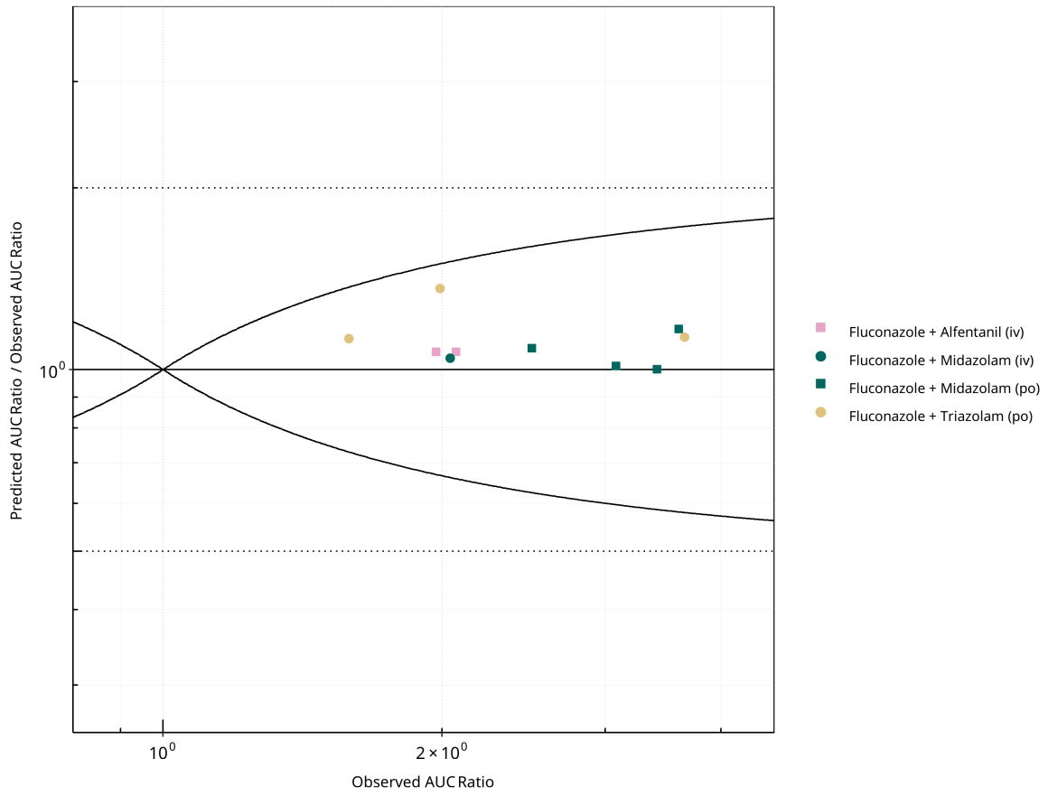
Figure 2-38: CYP3A4 DDI. Perpetrator: Fluconazole. Predicted/Observed vs. Observed AUC Ratio. ( \delta = 1 in Guest et al. formula)
