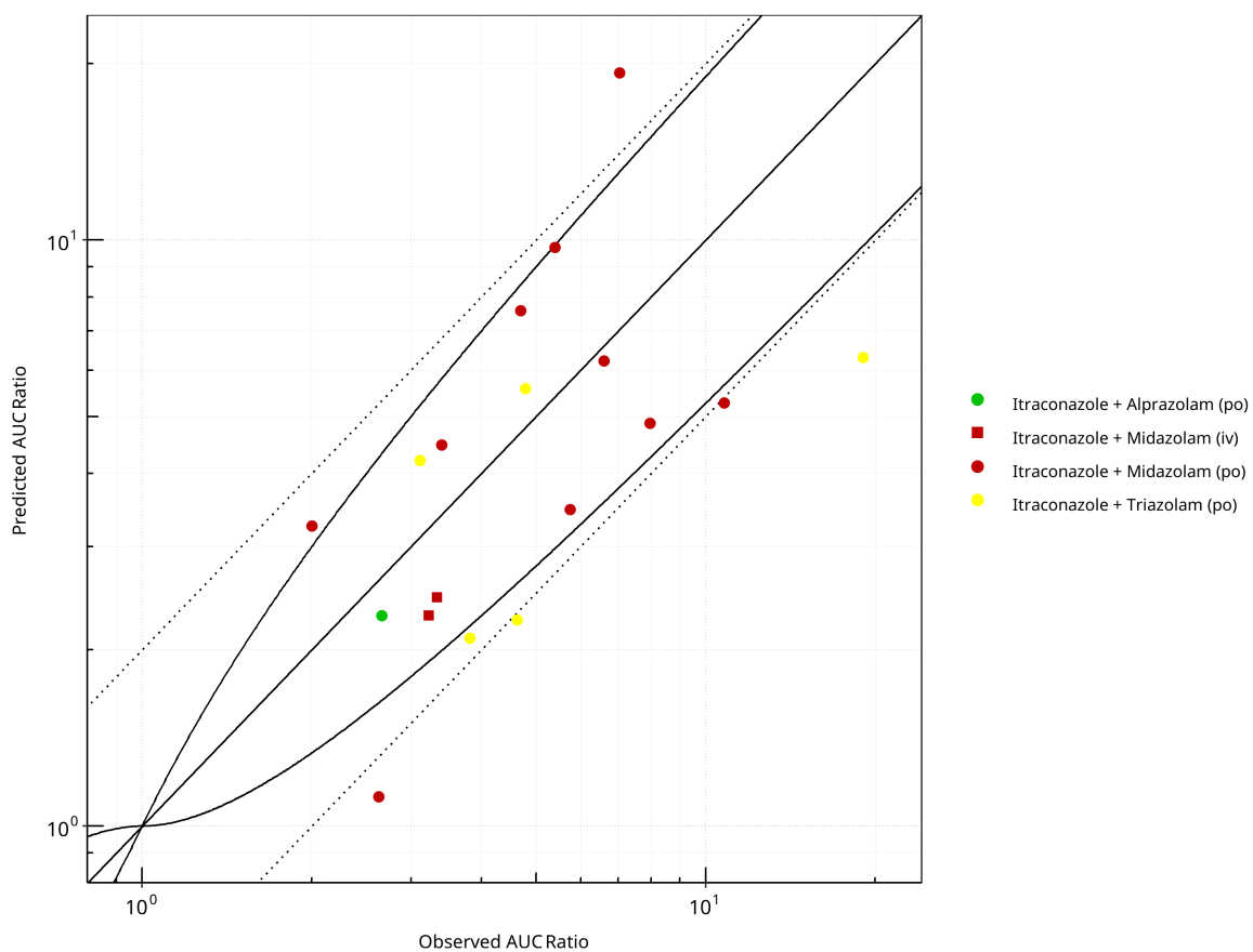
Figure 2-45: CYP3A4 DDI. Perpetrator: Itraconazole. Predicted vs. Observed AUC Ratio. ( \delta = 1 in Guest et al. formula)
