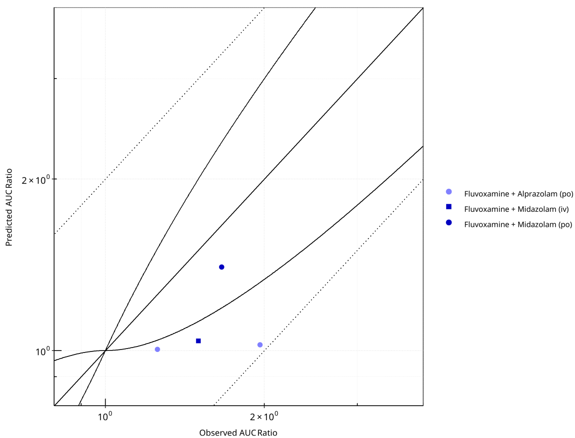
Figure 2-41: CYP3A4 DDI. Perpetrator: Fluvoxamine. Predicted vs. Observed AUC Ratio. ( \delta = 1 in Guest et al. formula)
