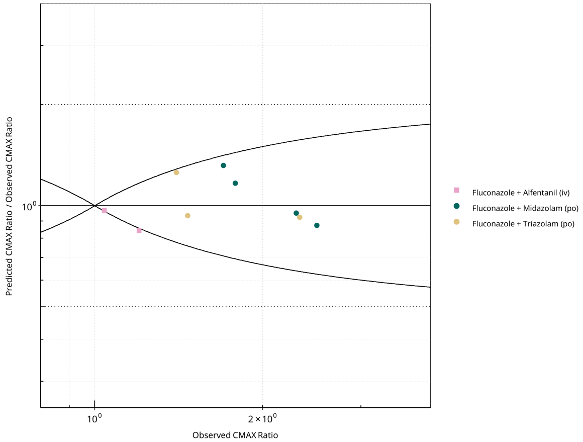
Figure 2-40: CYP3A4 DDI. Perpetrator: Fluconazole. Predicted/Observed vs. Observed CMAX Ratio. ( \delta = 1 in Guest et al. formula)
