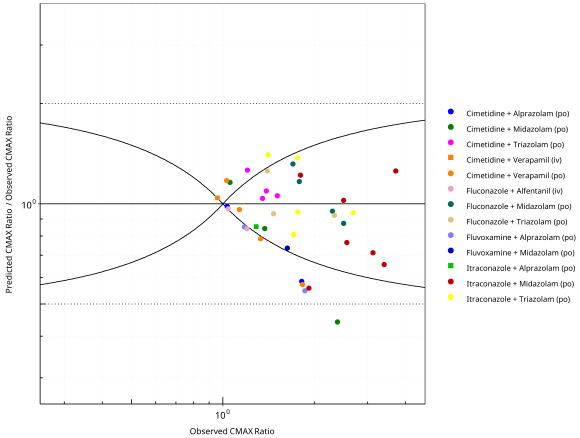
Figure 2-16: CYP3A4 DDI. Mechanism: Reversible Inhibition. Predicted/Observed vs. Observed CMAX Ratio. ( \delta = 1 in Guest et al. formula)
