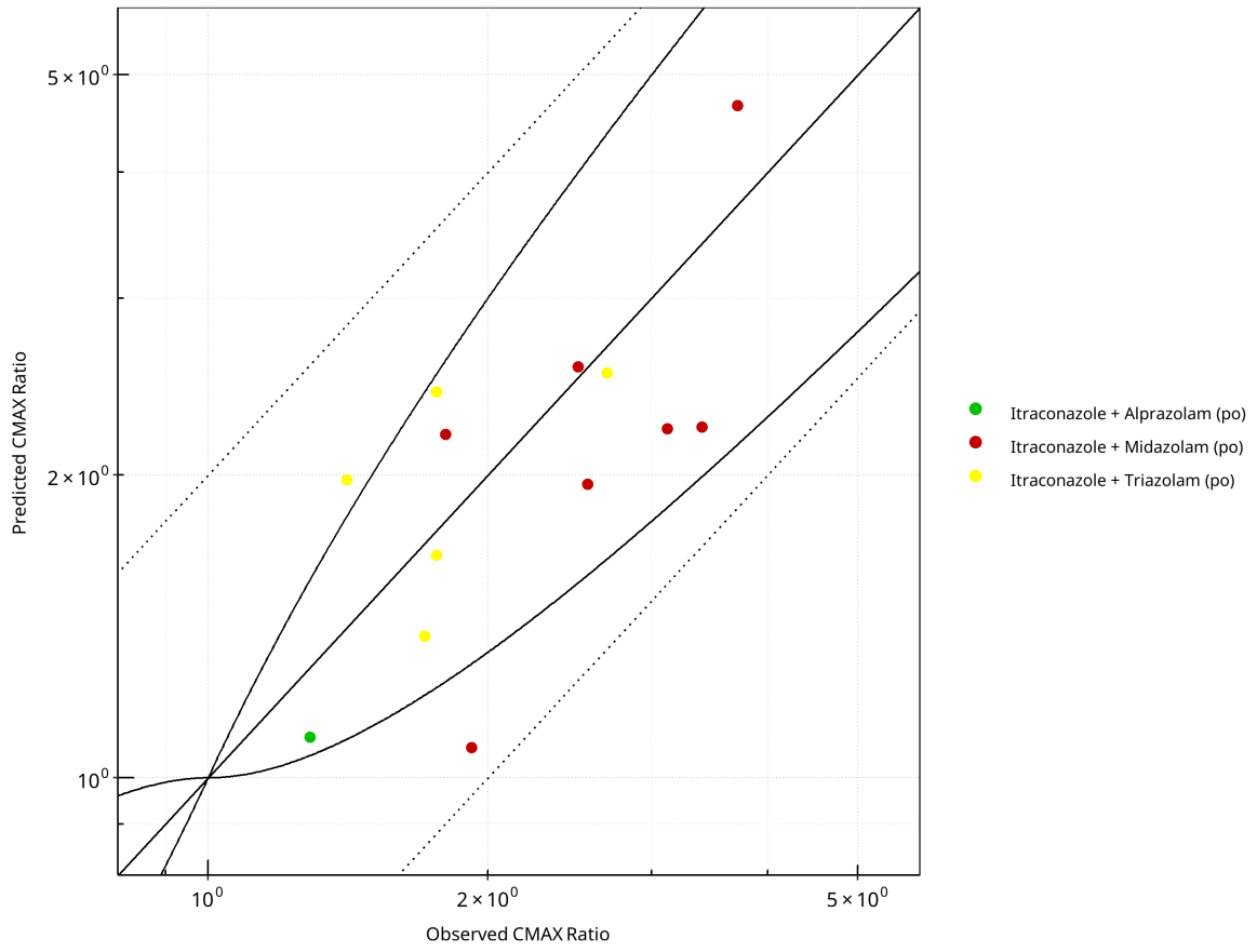
Figure 2-47: CYP3A4 DDI. Perpetrator: Itraconazole. Predicted vs. Observed CMAX Ratio. ( \delta = 1 in Guest et al. formula)
