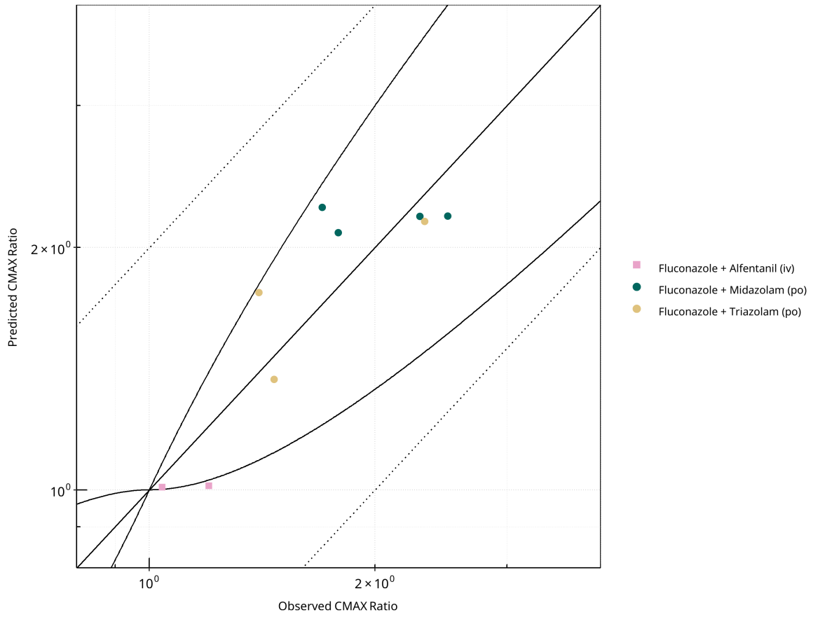
Figure 2-39: CYP3A4 DDI. Perpetrator: Fluconazole. Predicted vs. Observed CMAX Ratio. ( \delta = 1 in Guest et al. formula)
