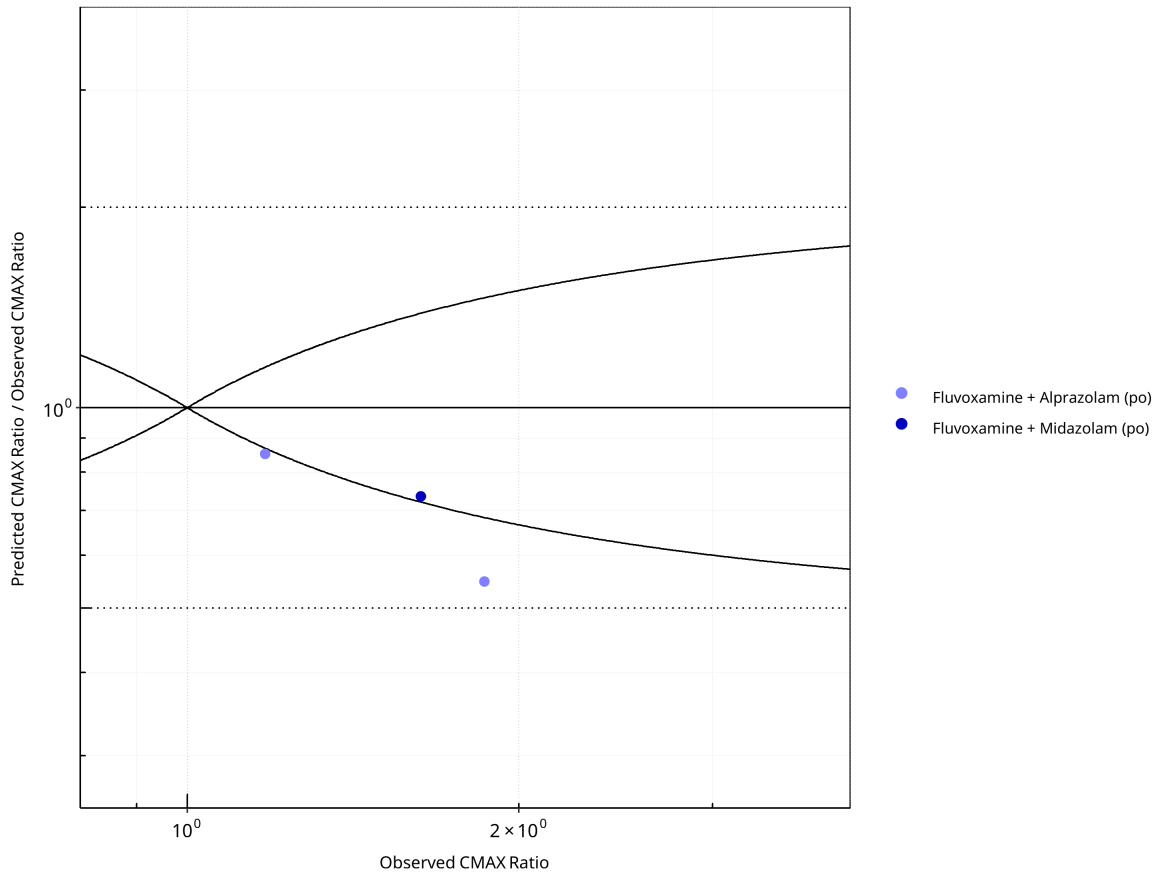
Figure 2-44: CYP3A4 DDI. Perpetrator: Fluvoxamine. Predicted/Observed vs. Observed CMAX Ratio. ( \delta = 1 in Guest et al. formula)
