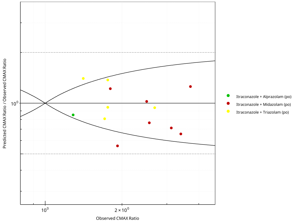
Figure 2-48: CYP3A4 DDI. Perpetrator: Itraconazole. Predicted/Observed vs. Observed CMAX Ratio. ( \delta = 1 in Guest et al. formula)
