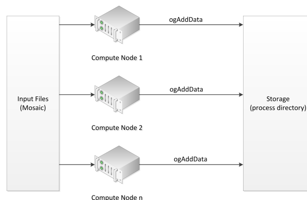
Figure 5: Calling ogAddData from different compute nodes
