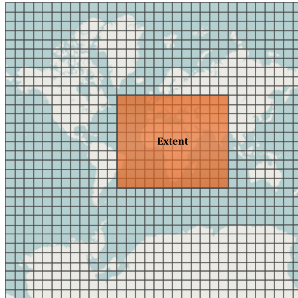
Figure 4: Example of an extent in tile coordinates
