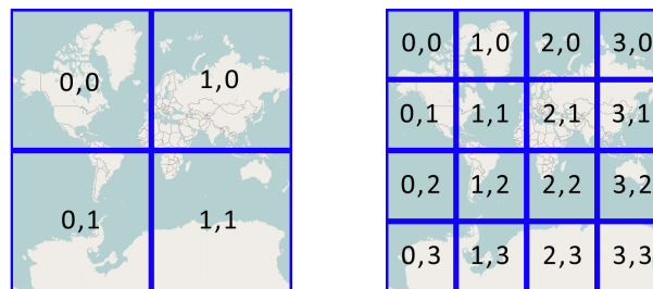
Figure 2: Tile Coordinates at different zoom levels
