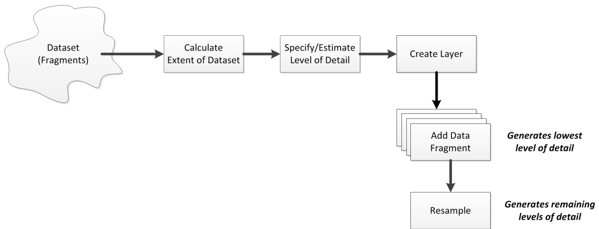
Figure 3: Workflow for data processing
