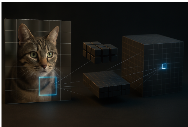
Figure 8.4: Receptive field grows with depth - allowing the model to capture global context.
