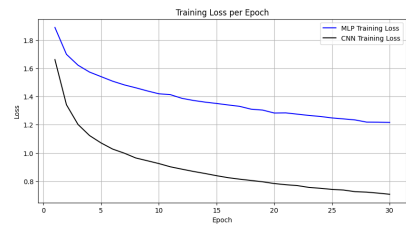
Figure 7.5: Training loss: CNN (black) reaches lower error than MLP (blue), faster.
