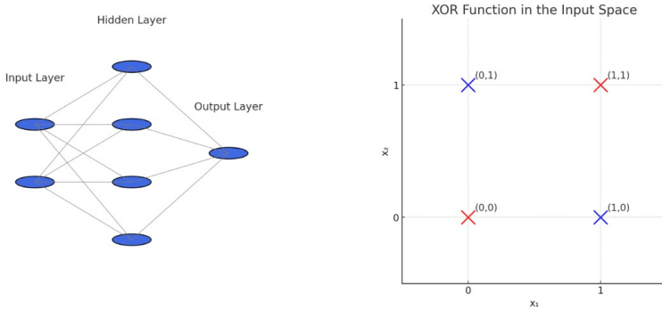
Figure 2.2: XOR classification: simplified neural network (left) and XOR function plot (right).
