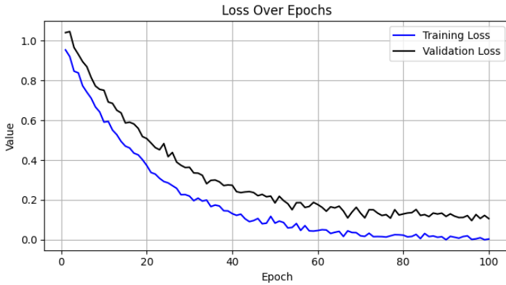
Figure 5.1: Training and validation loss over epochs: blue for training, black for validation.
