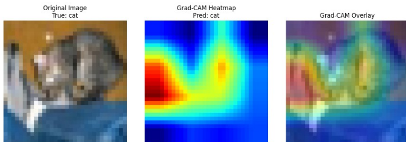
Figure 15.1: Example - visualizing a cat prediction in CIFAR-10. The image shows a Grad-CAM explanation for a CNN trained on CIFAR-10. The model correctly classifies the image as a cat , and Grad-CAM highlights the most relevant regions that led to this prediction.
