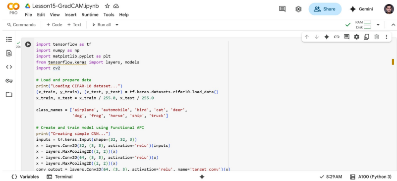
Figure 17.1: Google Colab Screenshot.
