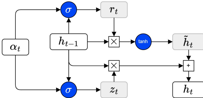
Figure 9.3: GRU architecture showing two gates: update and reset.
