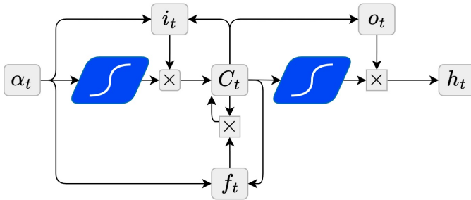
Figure 9.2: Internal structure of an LSTM unit.
