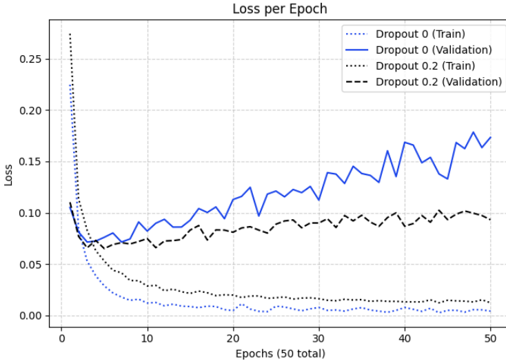
Figure 6.2: Validation loss and over epochs. Blue: without dropout. Black dashed: dropout with p = 0.2 .
