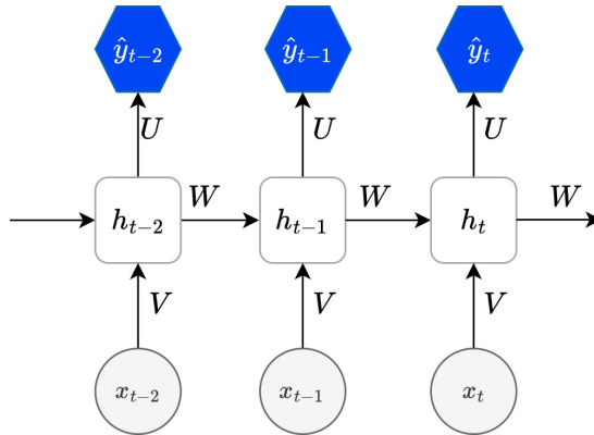
Figure 9.1: Unrolled Recurrent Neural Network architecture.
