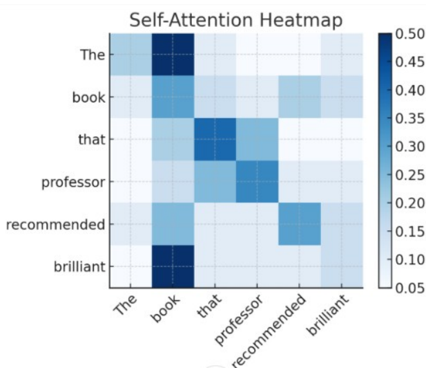
Figure 11.1: Self-Attention Heatmap for the sentence: "The solution that the professor recommended was brilliant."
