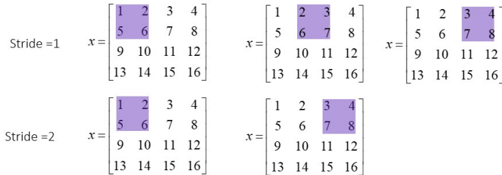
Figure 8.2: Effect of stride: top - stride 1 (dense scanning), bottom - stride 2 (coarser sampling).
