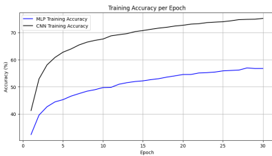
Figure 7.4: Training accuracy: CNN (black) reaches higher accuracy than MLP (blue), faster.
