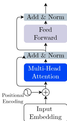
Figure 11.2: Encoder Illustration
