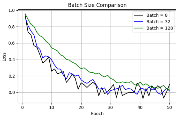
Figure 4.3: Batch size comparison. Black: small, Blue: medium, Green: large.
