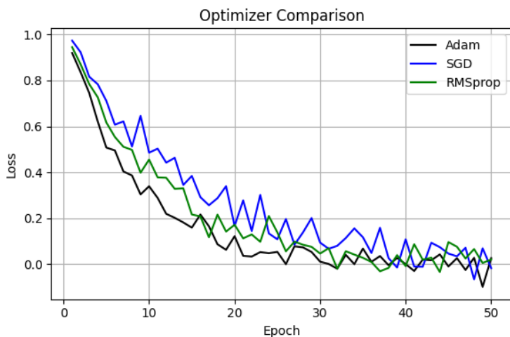
Figure 4.1: Optimizer comparison - Loss vs. Epoch. Black: Adam, Blue: SGD, Green: RMSProp.
