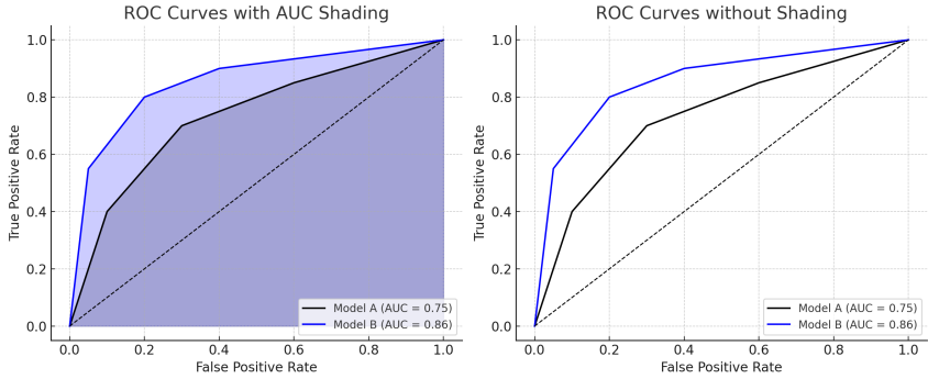
Figure 5.3: ROC curve with AUC (shading): Model A: black, AUC=0.75; Model B: blue, AUC=0.86.
