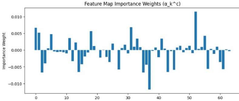
Figure 15.2: Bar chart showing the Grad-CAM importance weights \alpha_k^c for each feature map. Each feature map captures a specific visual pattern learned by the CNN (e.g., textures, shapes, parts). Positive weights indicate maps that supported the "cat" prediction; negatives were filtered by ReLU.
