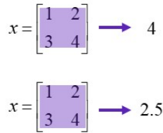
Figure 8.3: Pooling variants: top - max pooling; bottom - average pooling. Both reduce spatial resolution.
