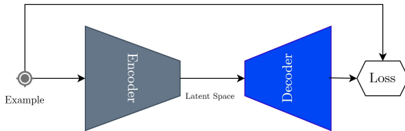
Figure 10.1: Autoencoder Illustration.
