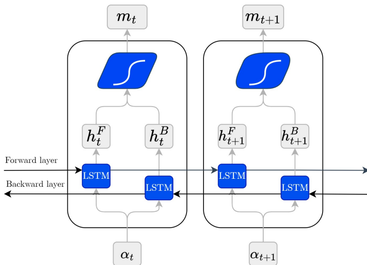
Figure 9.4: Bi-directional LSTM: combining forward and backward hidden states.
