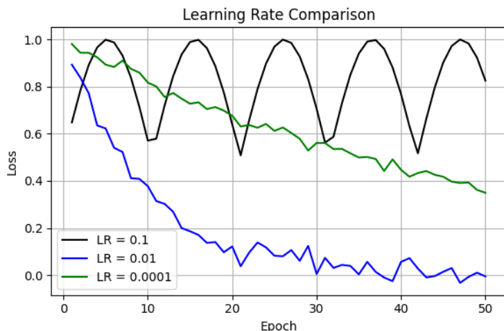
Figure 4.2: Learning rate comparison. Black: high \eta , Blue: medium \eta , Green: low \eta .
