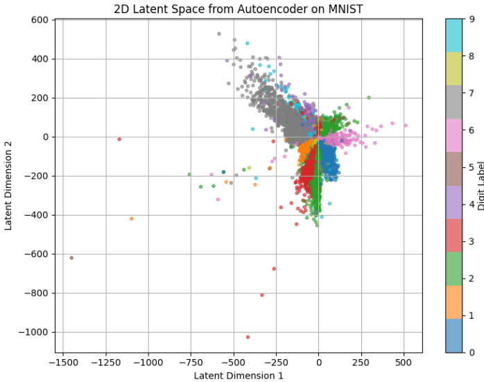
Figure 10.3: 2D latent space learned by the autoencoder. Colors indicate true digit labels (used for visualization only).
