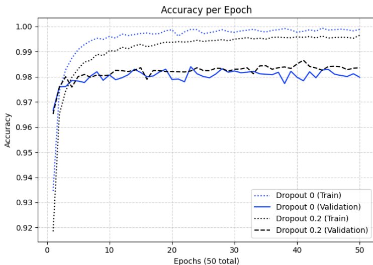
Figure 6.1: Accuracy over epochs. Blue: without dropout. Black dashed: dropout with p = 0.2 .
