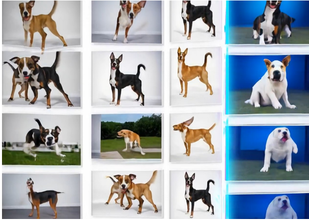
Figure 13.1: Augmentation Examples.
