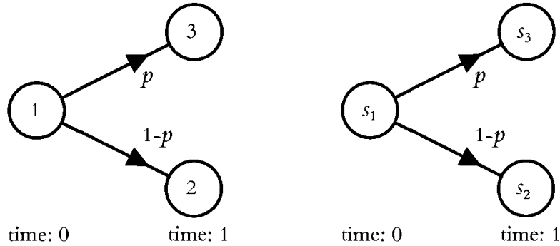
Figure 2.1 The binomial branch
