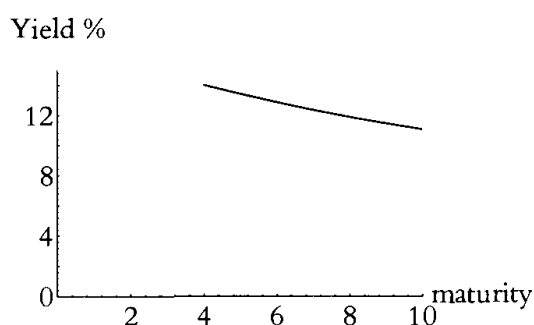
Figure 5.4 Yield curve at t = 4
