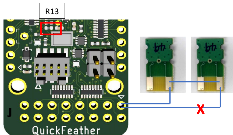
Figure 10: Microphones Wiring recommendation
