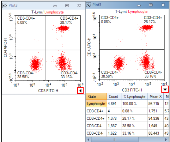
Figure 74. Statistical Data
