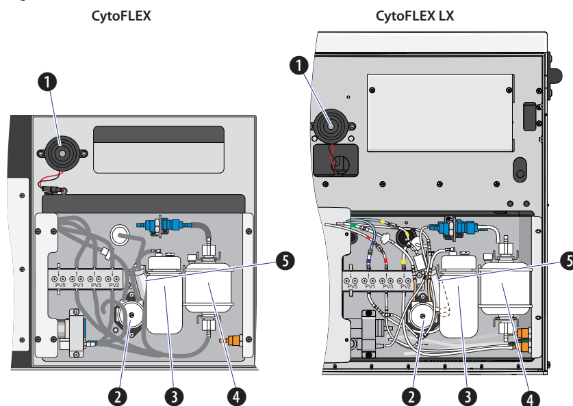
Figure 1.9 Fluidics Module View
