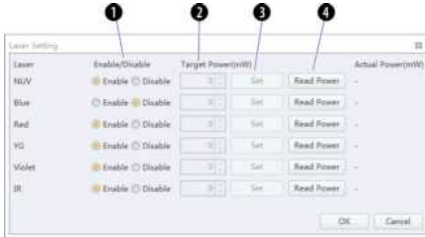
Figure 6.9 Laser Setting Window [CytoFLEX LX shown]
