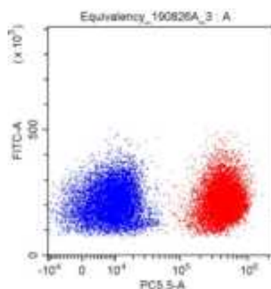
Dot plot with log-linear
