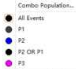
Figure 6.3 All Gates - Example Experiment
