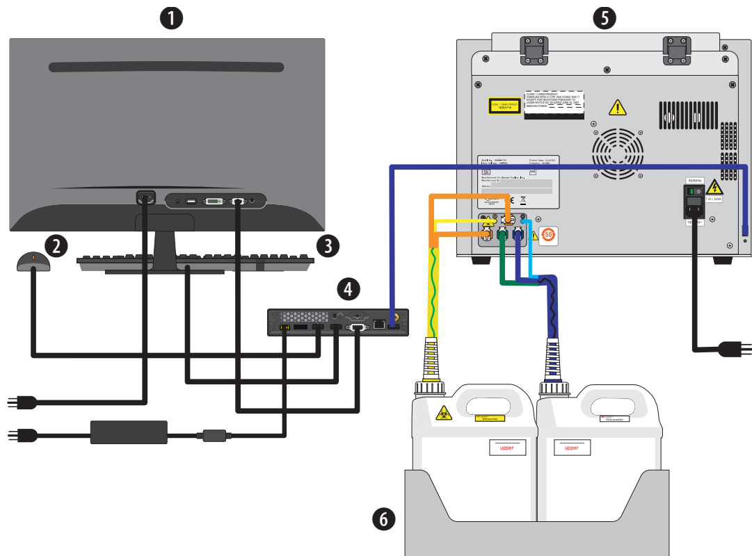
Figure 1.22 System Connections
