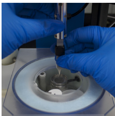
figure 1-33. Releasing the plunge tweezers from the plunge rod
