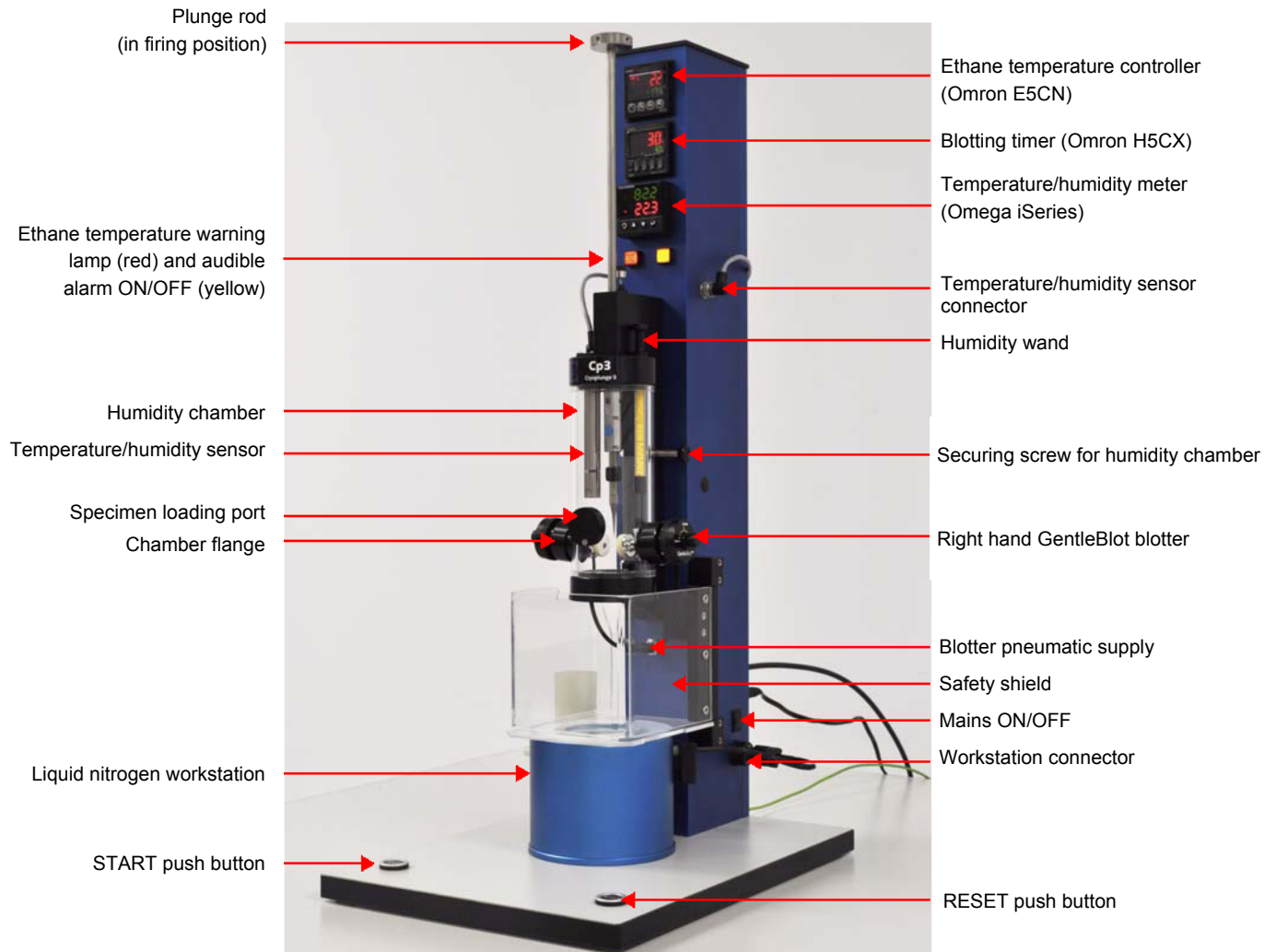
figure 1-1. Cryoplunge3 front view
