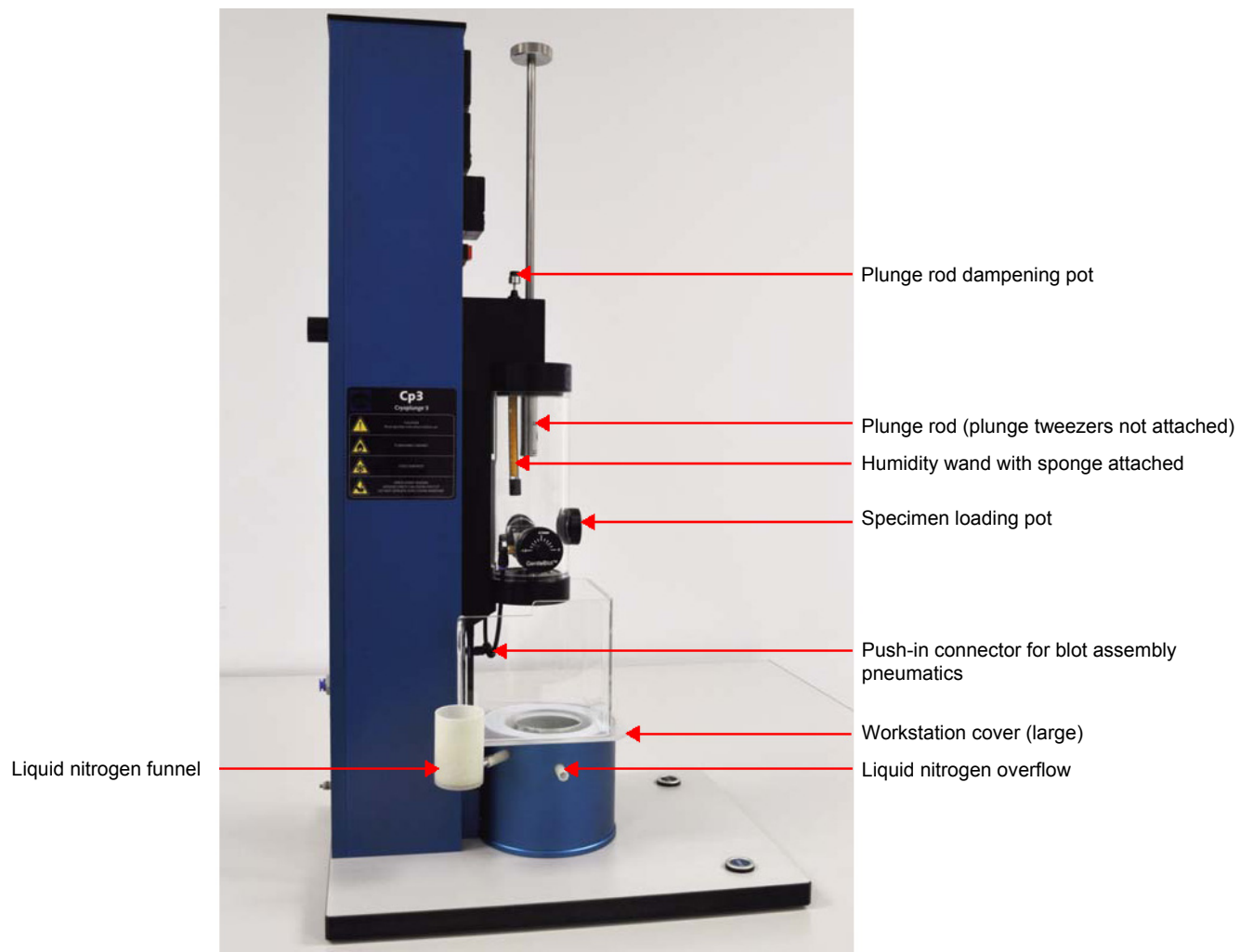
figure 1-2. Cryoplunge3 side view left
