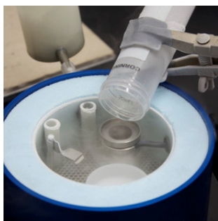
figure 1-26. Pouring the condensed ethane into the precooled ethane pot
