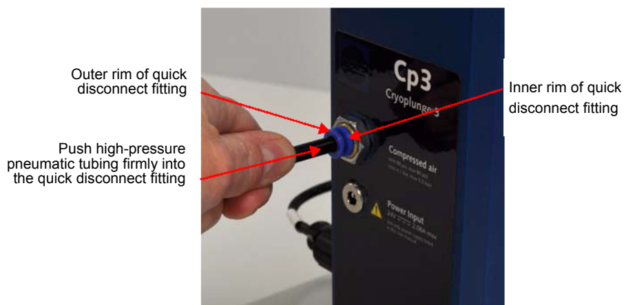
figure 1-8. Pneumatic connection
