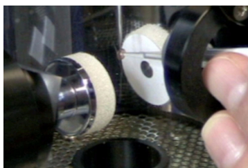
figure 1-30. Applying sample aliquot to the support film
