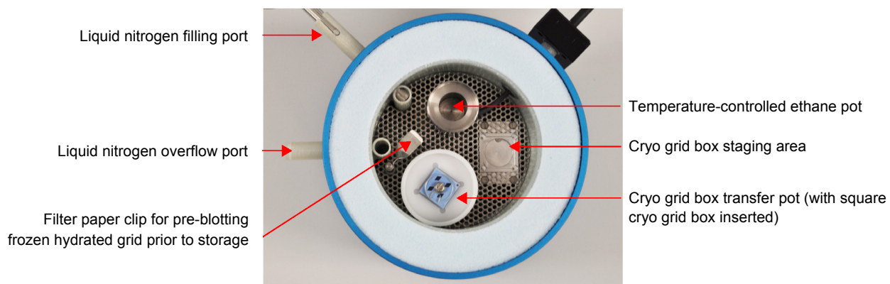
figure 1-4. Workstation
