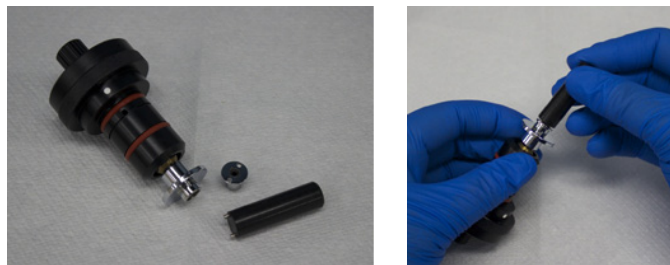
figure 1-18. Removing the spindle
