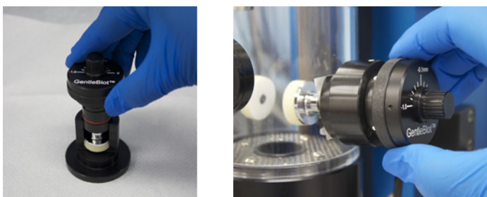
figure 1-21. Attaching the filter paper disk and inserting the blotter
