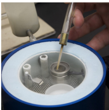
figure 1-24. Condensing ethane directly into the pre-cooled ethane pot
