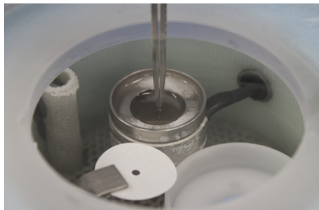
figure 1-32. Grid plunging into the liquid ethane
