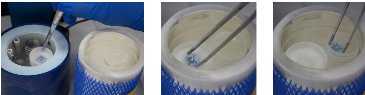
figure 1-37. Transfer the grid box to the storage tube filled with liquid nitrogen
