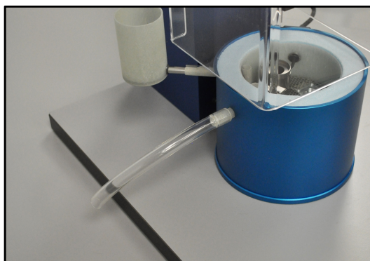
figure 1-11. Workstation overflow port with Tygon tubing attached
