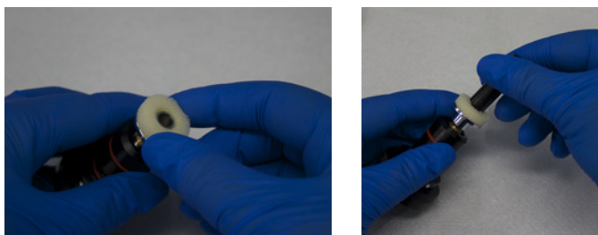
figure 1-19. Inserting the sponge pad
