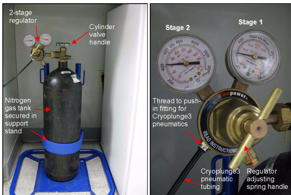
figure 1-5. Pneumatics supply for Cryoplunge3 (left), 2-stage nitrogen regulator (right)
