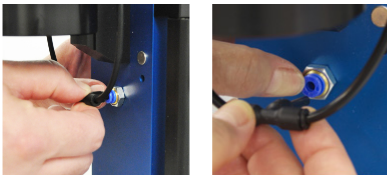
figure 1-41. Disconnect the pneumatic supply for the blotter assemblies
