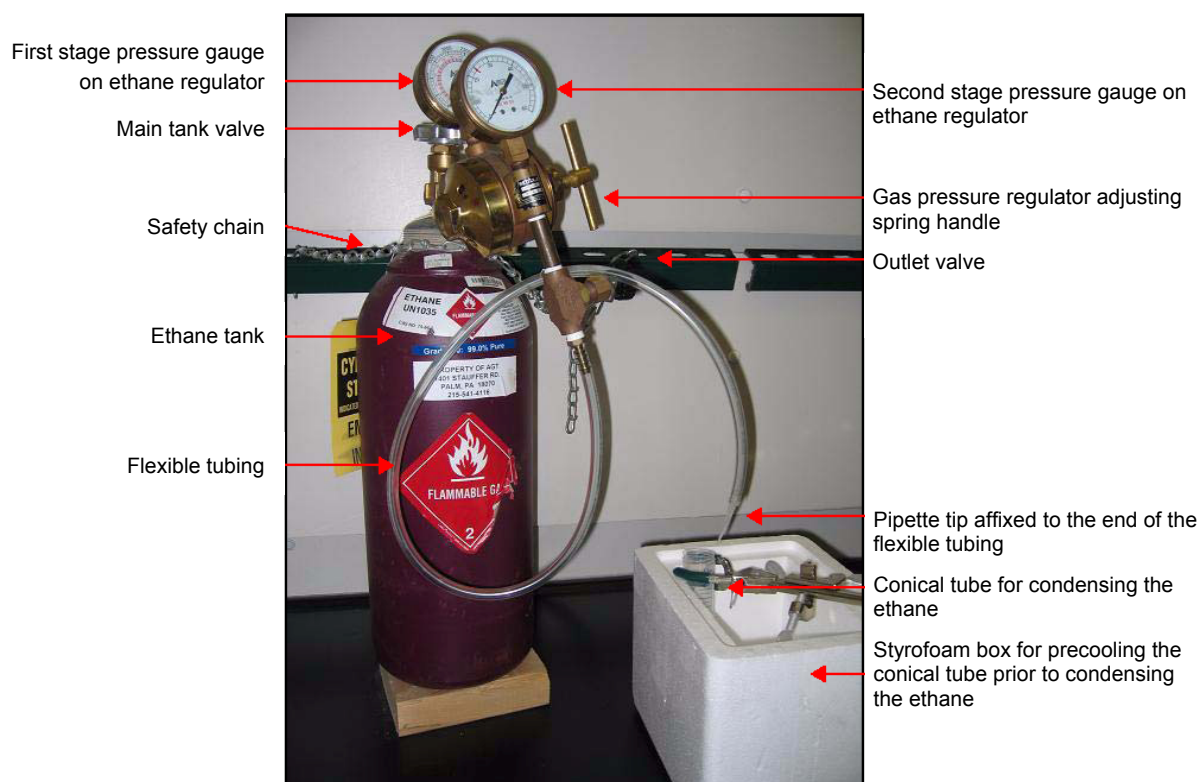
figure 1-6. Ethane tank and regulator
