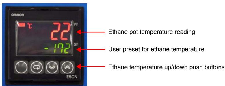
figure 1-22. Meter for ethane temperature controller
