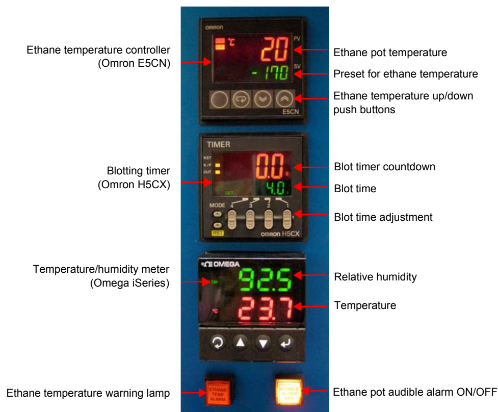
figure 1-15. Meters and alarms for Cryoplunge3
