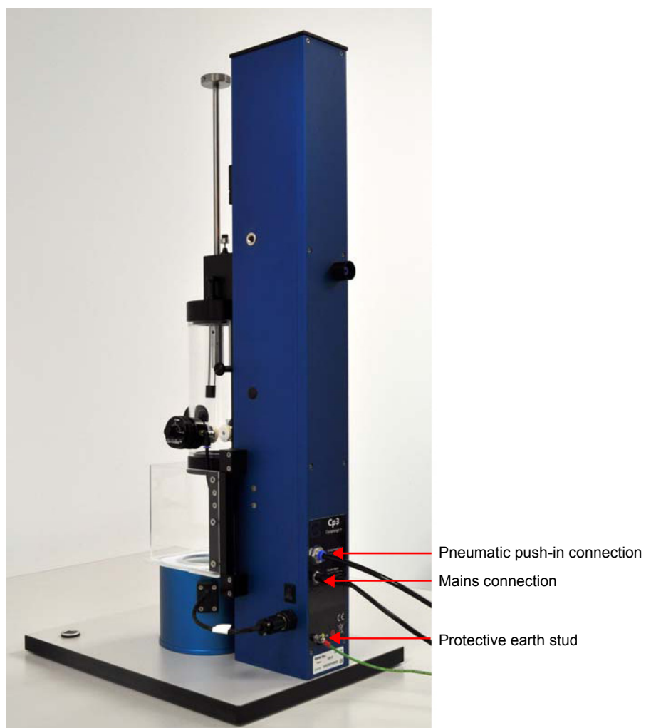
figure 1-3. Cryoplunge3 side view back and right
