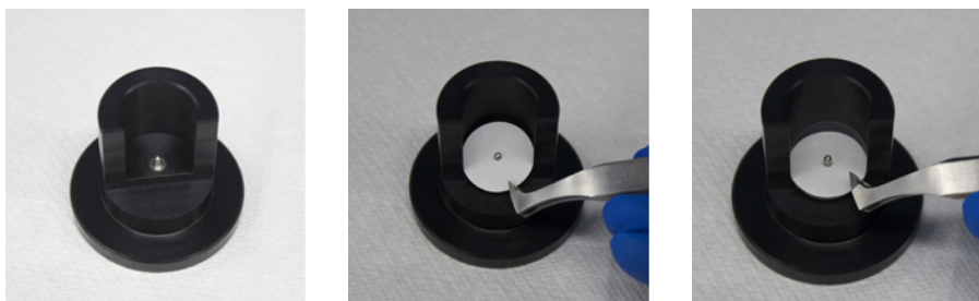
figure 1-20. Loading the filter paper disk and protective plastic backer
