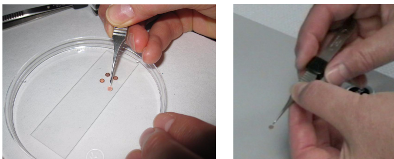
figure 1-27. Securing the specimen grid to the plunge tweezers
