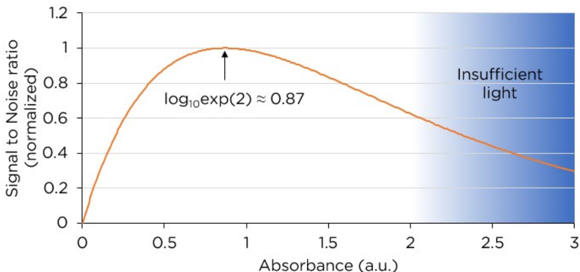
Figure 105: Signal-to-noise ratio as a function of absorbance.
