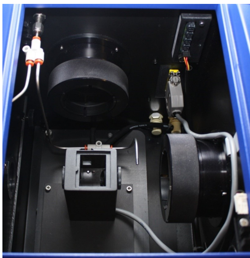
Figure 26: The interior of the sample chamber with the threaded spacer and detector cowling removed
