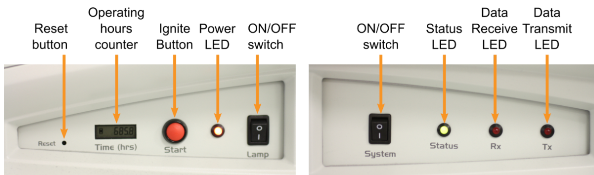
Figure 10: The front panel, including lamp panel (left) and system panel (right)
