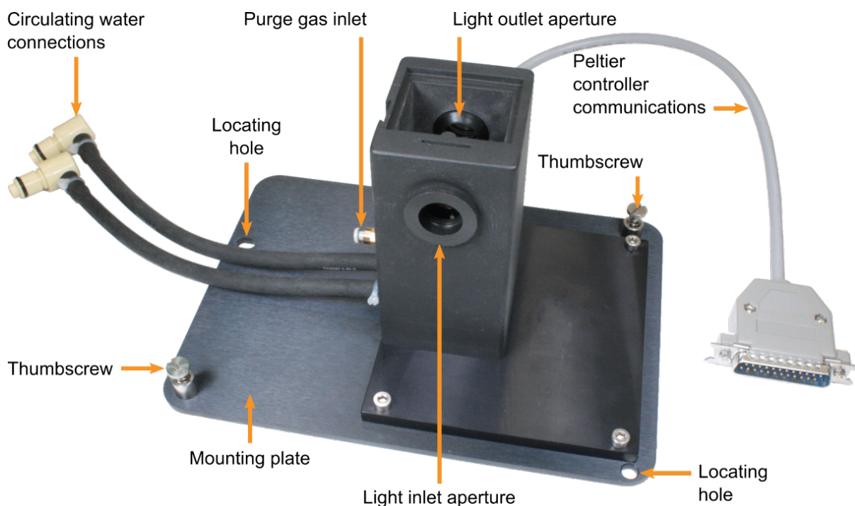
Figure 16: The Single Cell Peltier Holder
