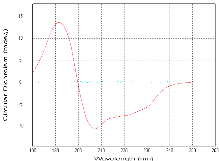
Figure 8: Smoothed and baseline-corrected spectrum of lysozyme (red) and smoothing residuals (cyan)
