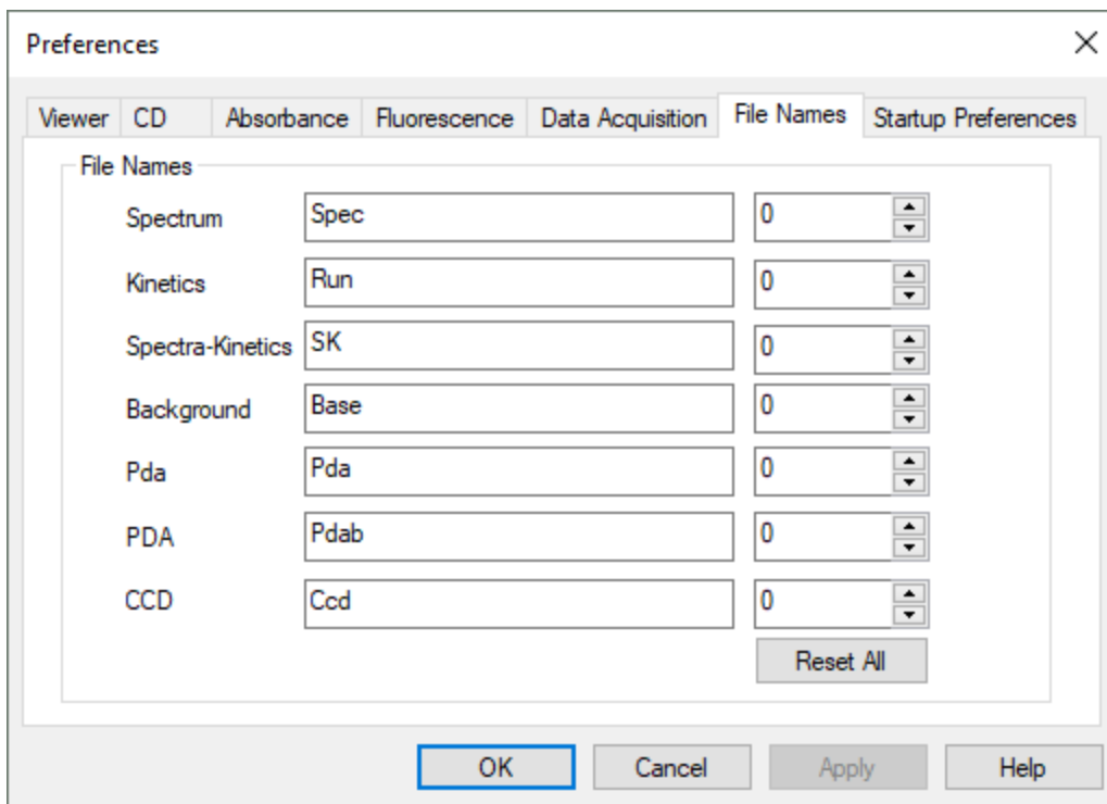
Figure 54: The File Names tab
