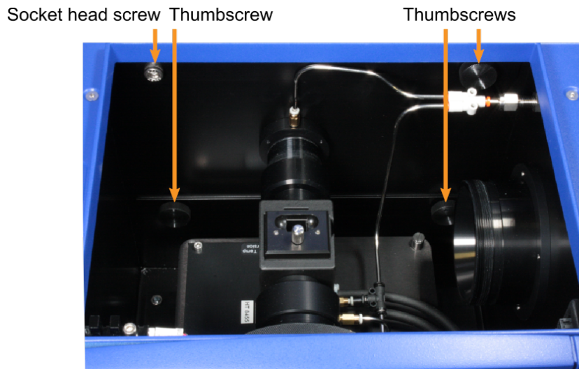
Figure 22: The interior of the sample chamber, viewed from the right
