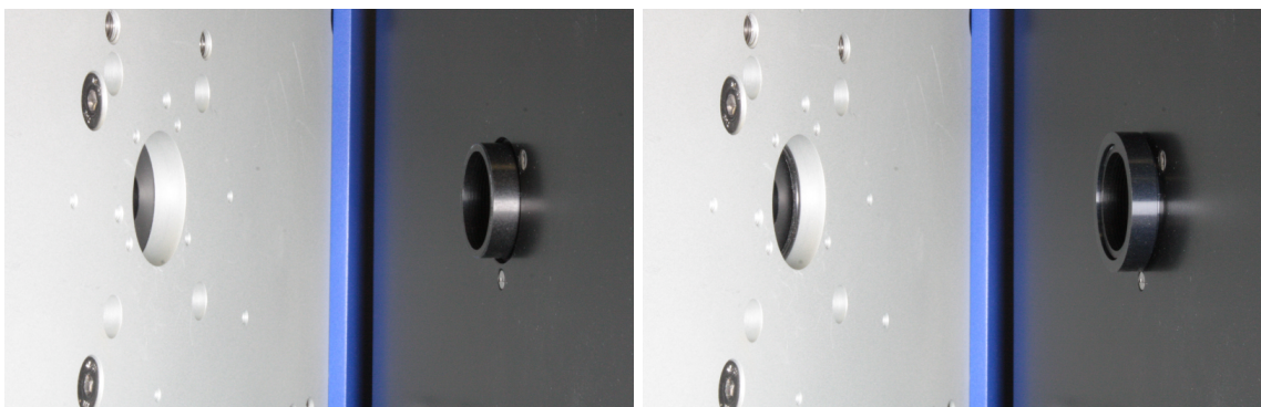
Figure 24: The monochromator on the left side and the sample chamber monochromator port on the right side without (left) and with O-ring and locator guide in place (right)
