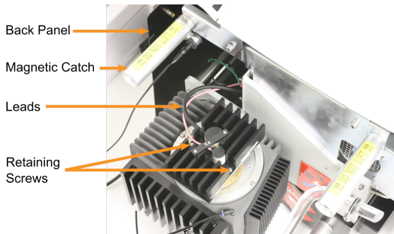
Figure 114: Lamp housing fittings with lamp cover removed
