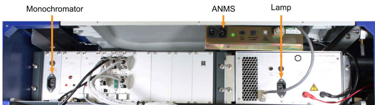
Figure 11: Rear of the spectrometer showing the three mains connections
