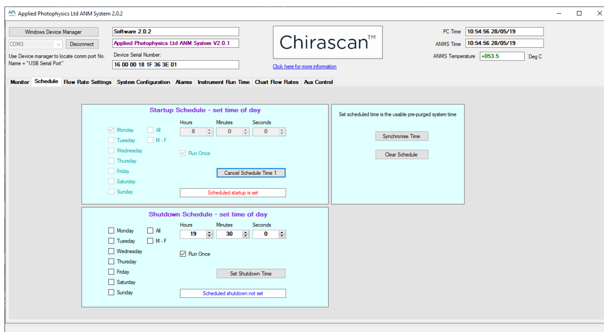
Figure 30: The Schedule tab of ANMS
