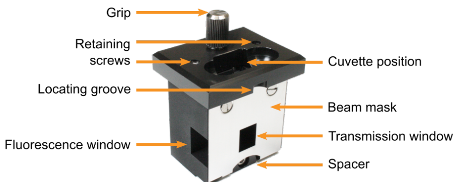
Figure 17: 10-mm cuvette holder
