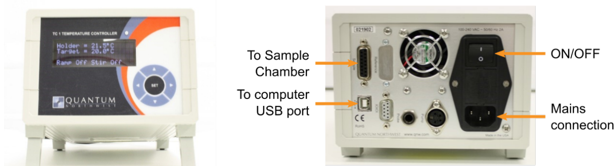
Figure 19: The Peltier temperature control unit for the sample chamber front view (left) and rear view with connections (right)
