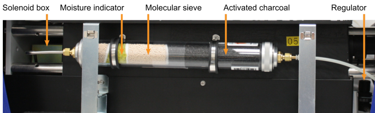
Figure 12: Components of the nitrogen purge gas flow
