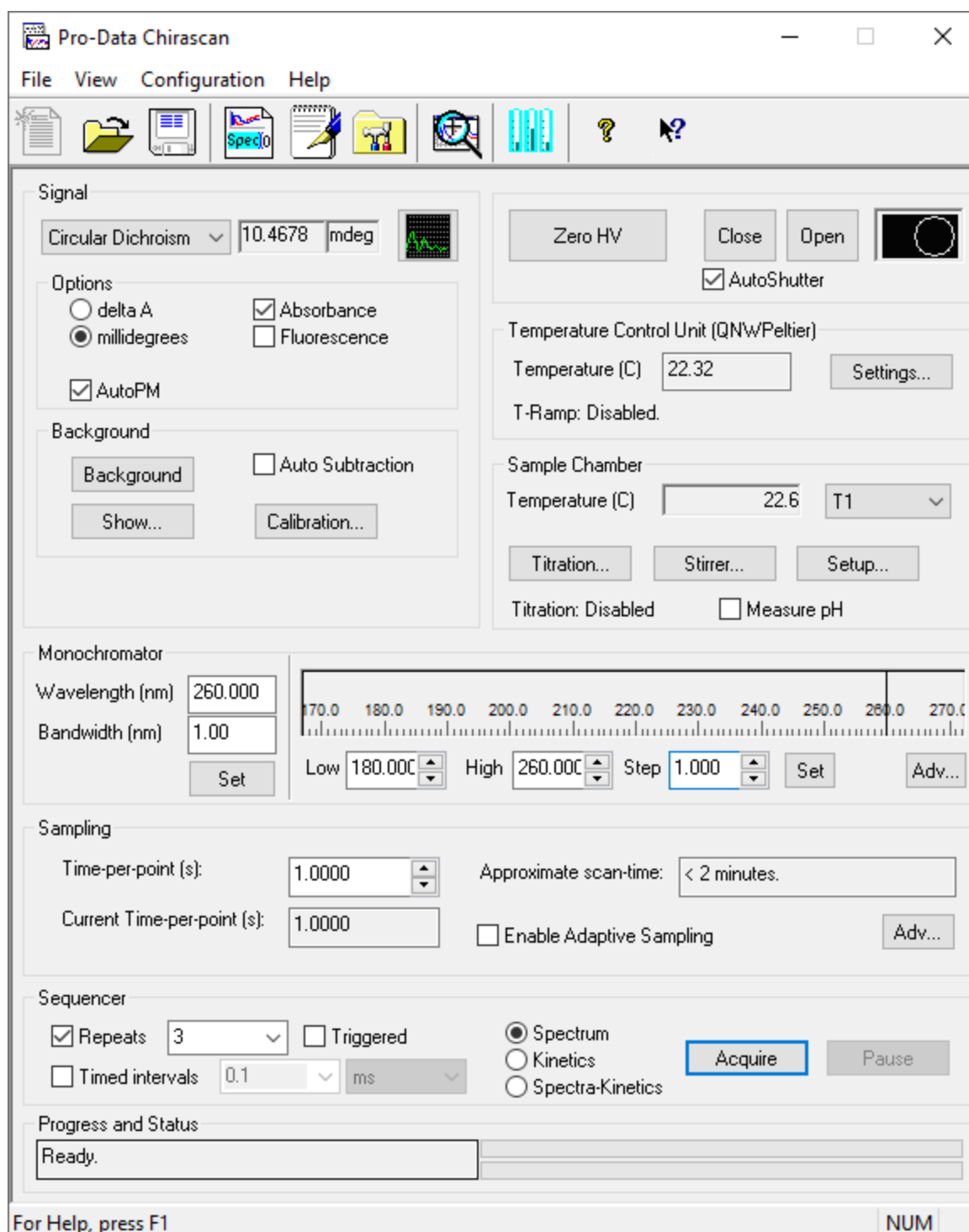
Figure 32: The Spectrometer Control Panel
