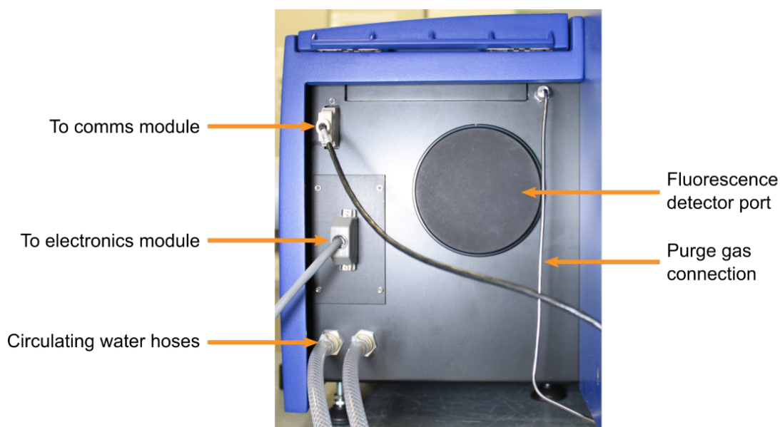
Figure 14: The rear of the sample chamber
