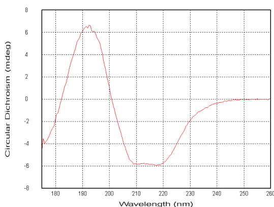
Figure 106: CD spectrum of alcohol dehydrogenase
