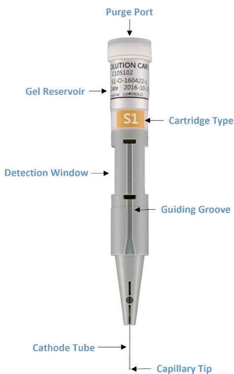
Figure 13 Pen-Shaped Gel Cartridge
