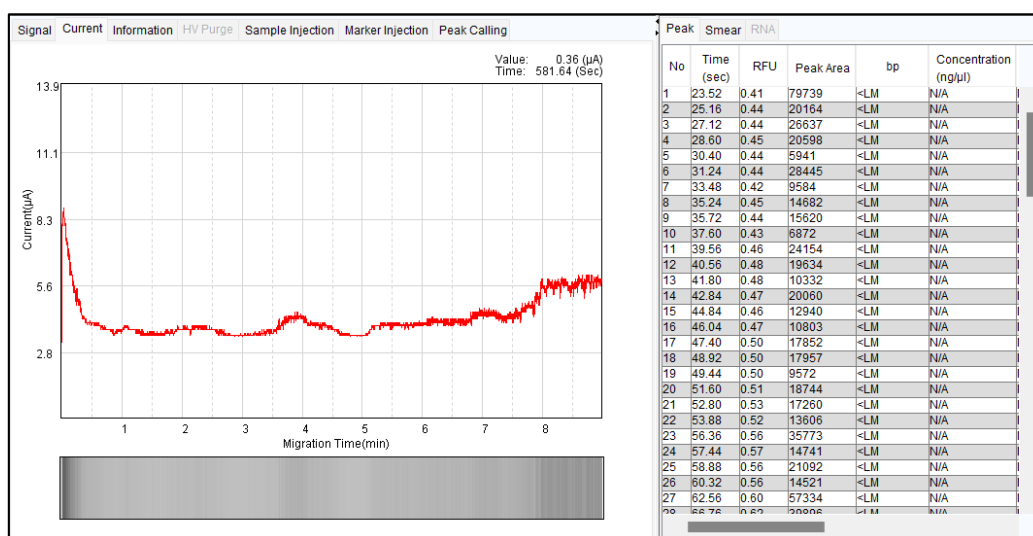
Figure 28 Low and Unstable Current
