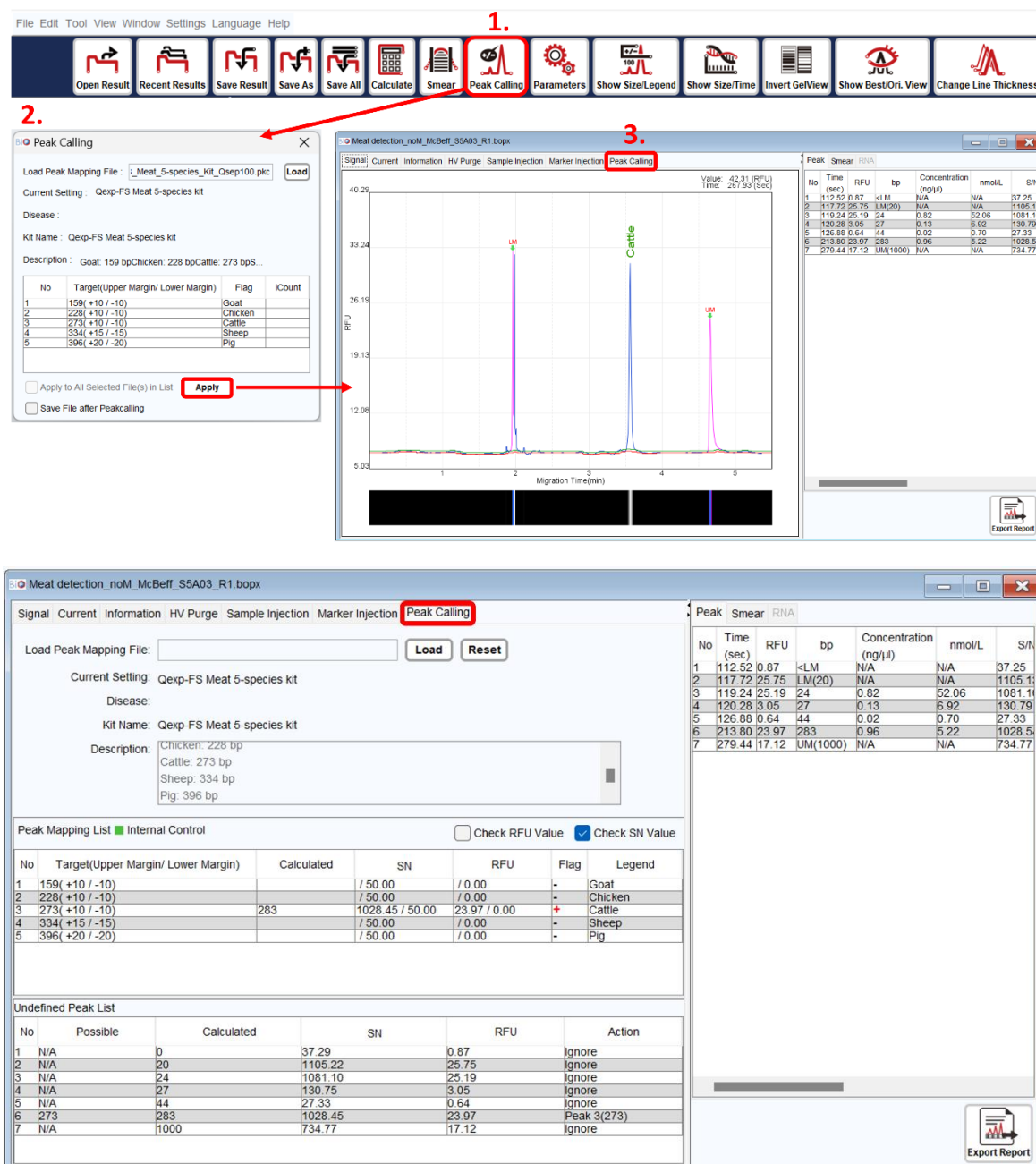
Figure 37 Peak Calling Function
