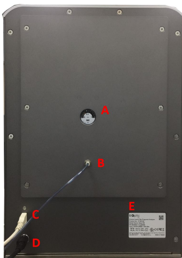
Figure 2 Back View of Qsep 100
