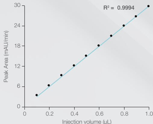
Injection volume linearity of a caffeine standard from 0.1 to 1.0 μL using flow injection analysis.
