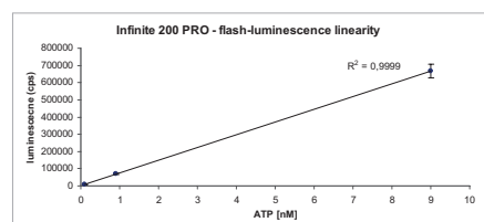
Flash luminescence linearity of the Infinite 200 PRO using optimized conditions for ATP detection.
