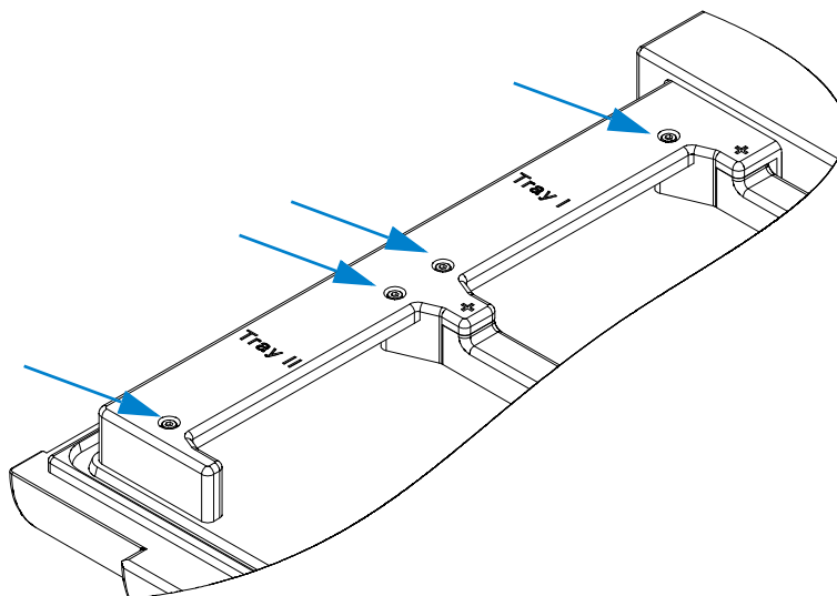
Figure 25 Disassembling the anode connector.
