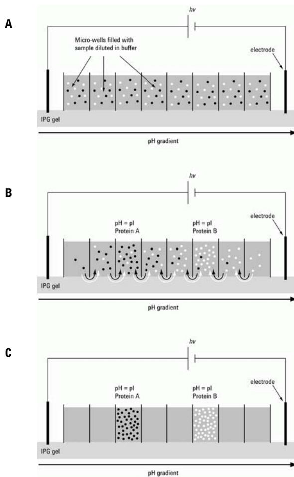
Figure 1 Fractionation principle of the Agilent 3100 OFFGEL Fractionator.
