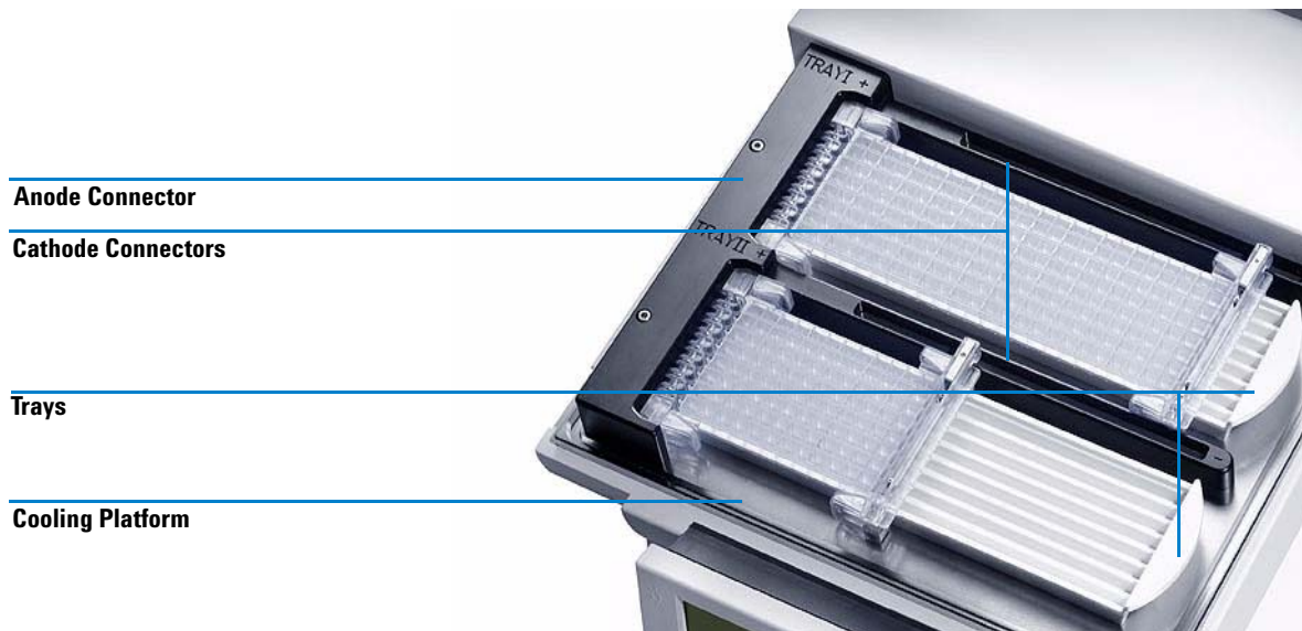
Figure 3 View inside the instrument.
