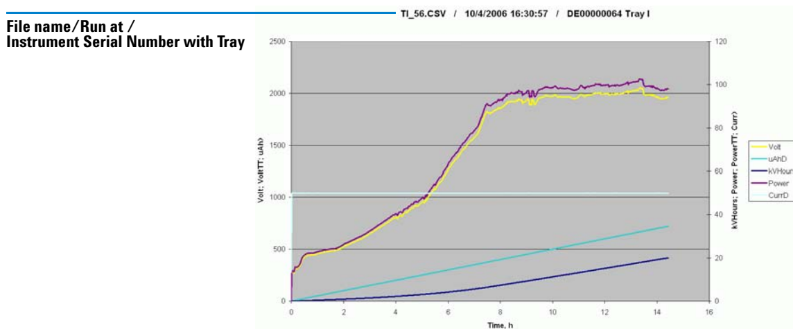
Figure 22 Plotted graph of run parameters (y-axes) versus time [h].
