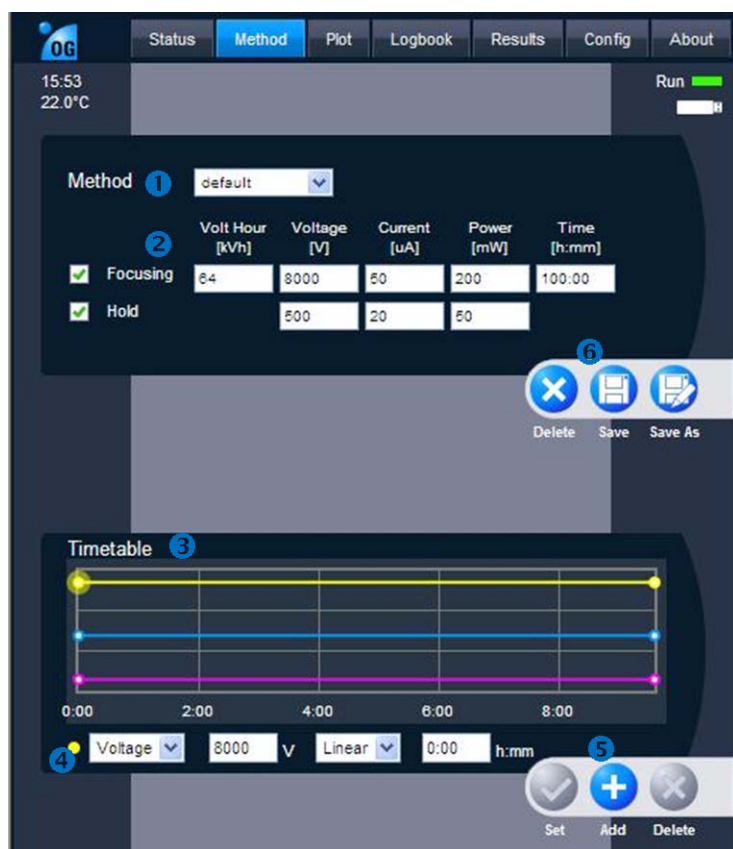
Figure 14 Editing Methods
