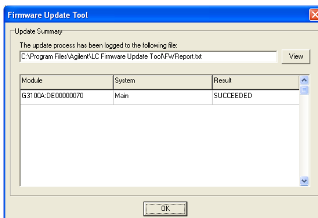
Figure 40 Report Screen
