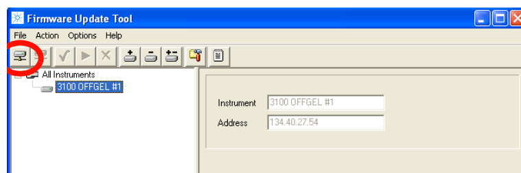
Figure 34 Select "3100 OFFGEL #1"
