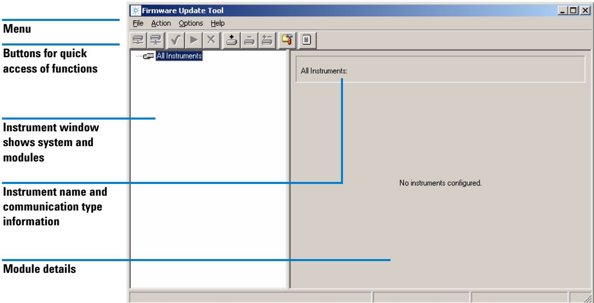
Figure 28 Start-up screen
