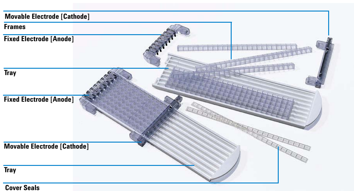
Figure 4 Electrodes, trays and frames
