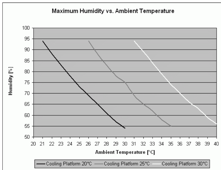
Figure 1 Plot of humidity versus ambient temperature assuming the cooling platform to be set at 20 °C, 25 °C or 30 °C. For non-condensing condition the humidity has to be below the plotted curves.
