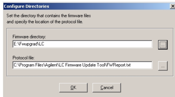
Figure 30 Configure Directories
