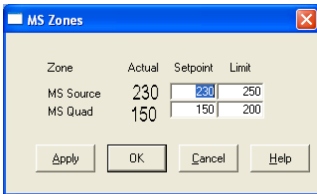
Figure 15 Setting temperatures
