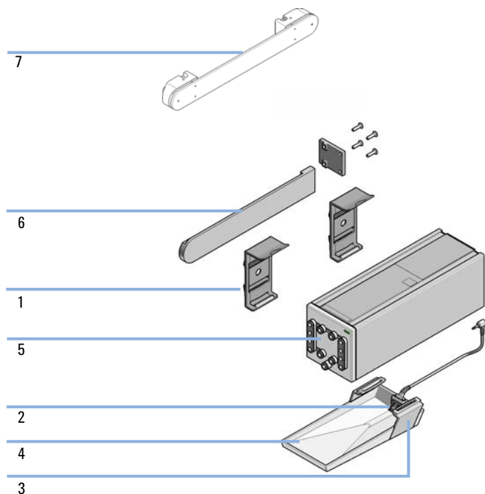
Figure 9 Valve Drive Parts
