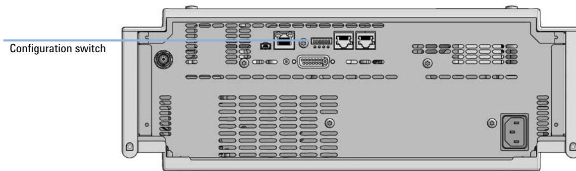
Figure 13 Location of Configuration switch (example shows a G7114A/B VWD)
