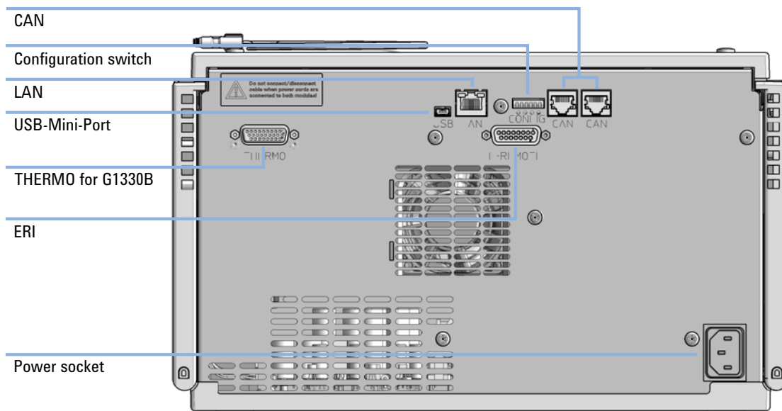
Figure 11 Fraction collector electrical connections
