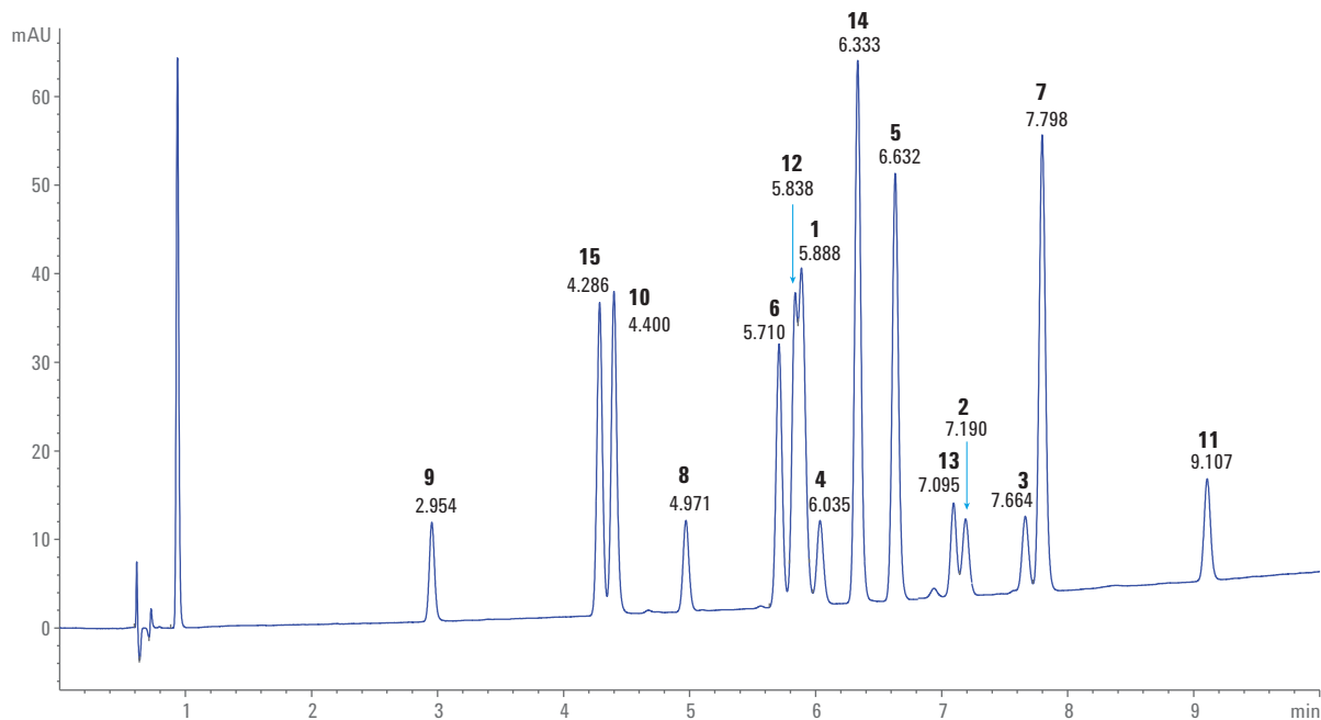
Figure 10. Separation of a complex 15 pesticide sample in UHPLC mode on an C18 phase column with water/acetonitrile as solvents (see the Experimental section).
