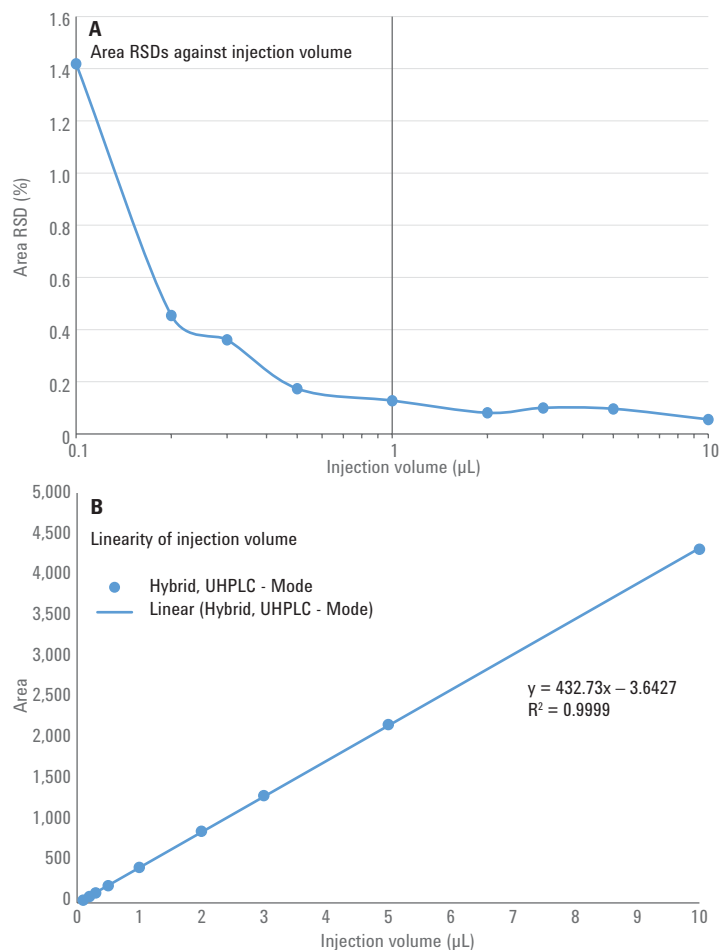
Figure 6. Performance in UHPLC mode. A) Determination of peak area RSDs in dependence of the injection volume (0.1, 0.2, 0.3, 0.5, 1.0, 2.0, 3.0, 5, and 10 \mu\text{L} ). Area RSDs are typically below 0.2 % for all injection volume above 0.5 \mu\text{L} . B) Peak area linearity of injection volumes between 0.1 and 10 \mu\text{L} , R^2 = 0.9999 .
