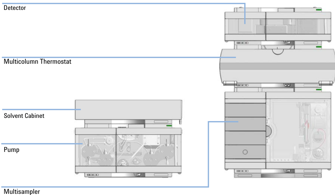
Figure 8 Recommended Two-Stack Configuration for 1290 Infinity II
